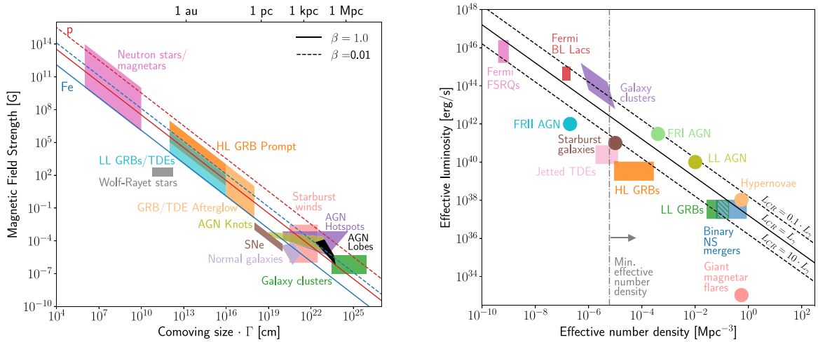
Fig. 2. Left: Hillas plot showing candidate UHECRs acceleration sites as colored areas on the size (horizontal axis) versus magnetic field (vertical axis) plane. The acceleration to 10 20 eV is not possible below diagonal lines which are red for proton, blue for iron, solid for maximum shock velocity \beta = 1 and dashed for \beta = 0.01 . \Gamma is the Lorentz factor of the acceleration region with respect to observer. Right: luminosity of the candidate sources versus their space number density (steady sources), or effective luminosity versus effective number density (transient sources, assumed lifetime 3 \times 10^5 yr). The black solid line shows the UHECRs energy production rate of 5 \times 10^{44} erg Mpc -3 yr -1 . The gray vertical line gives the lower limit on the UHECRs source number density. Source: Plots adopted from Ref. [660].
