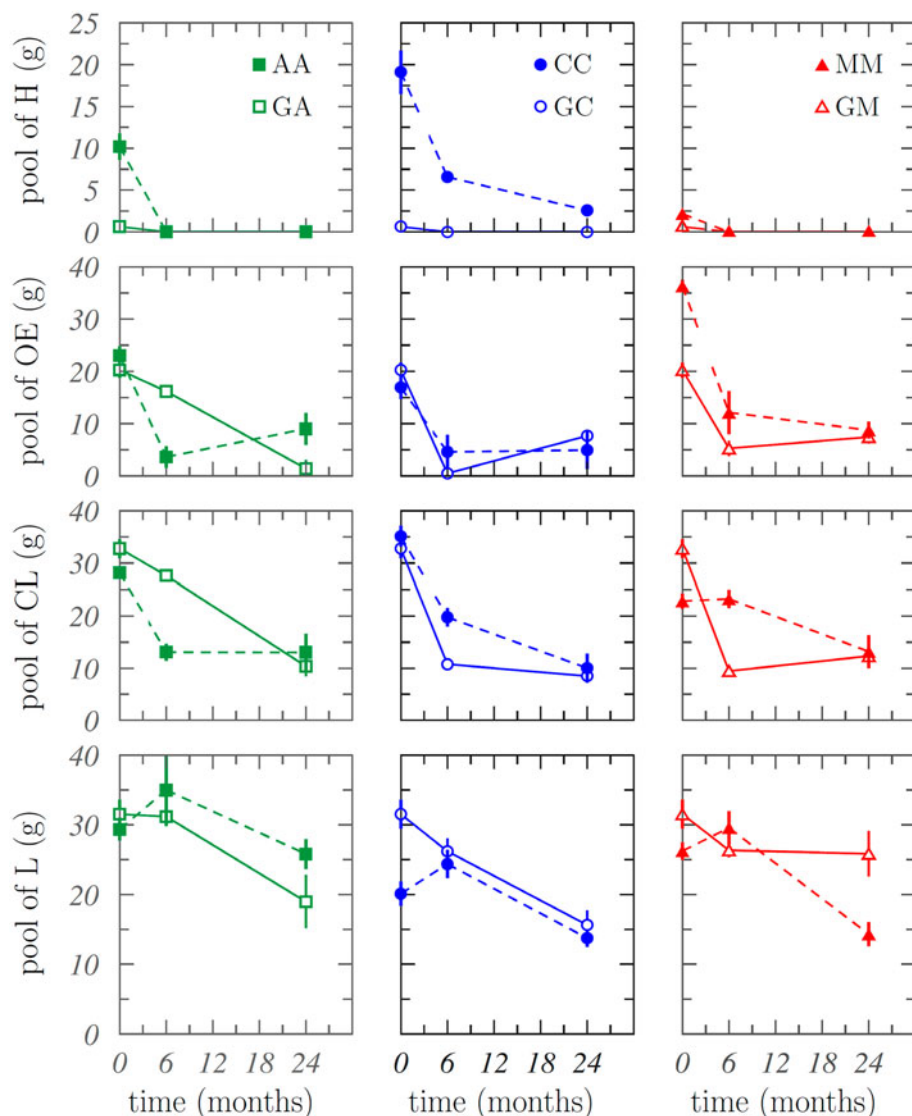
Fig. 4. (Colour online) Fibre pool (lignin (L), cellulose (CL), other extracts (OE) and hemicellulose (H)) in species (avocado pruning waste on avocado crop (AA), cherimoya pruning waste on cherimoya crop (CC) and mango pruning waste on mango crop (MM)) and garden waste (garden waste on avocado crop (GA), garden waste on cherimoya crop (GC) and garden waste on mango crop (GM)) in each sampling period. Note: Thin bars represent the standard error of the sample. P < 0.05 .
