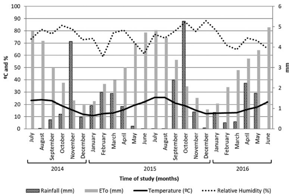
Fig. 1. Temperature, rainfall, reference ETo and relative humidity averages per month during the study period.
