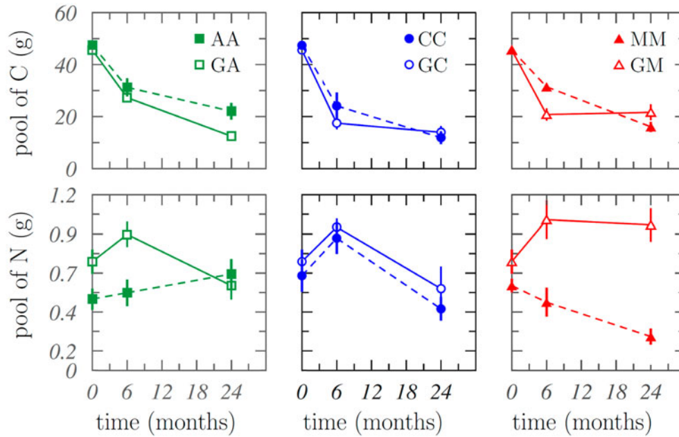
Fig. 3. (Colour online) Pools of carbon (C) and nitrogen (N) in species (avocado pruning waste on avocado crop (AA), cherimoya pruning waste on cherimoya crop (CC) and mango pruning waste on mango crop (MM)) and garden waste (garden waste on avocado crop (GA), garden waste on cherimoya crop (GC) and garden waste on mango crop (GM)) in each sampling period. Note: Thin bars represent the standard error of the sample. P < 0.05 .
