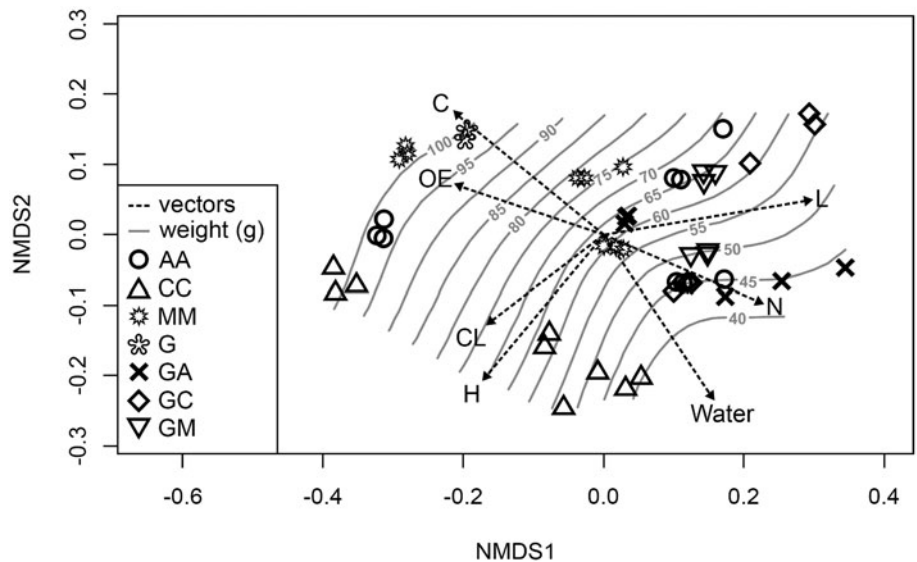
Fig. 5. NMDS plot of all the pruning waste generated, including all the variables (vectors) studied (carbon (C), nitrogen (N), lignin (L), cellulose (CL), hemicellulose (H), other extracts (OE) and water input (water)) and relating them to the weight over time (T0, T6 and T24). Note: 'G' garden waste at T0 because the garden waste have the same composition at T0 in all locations (crops), and this composition varies differently over time (T6 and T24) for the different crops. The length of the vector represents the influence of the variable. The direction of the vector (variable) explains the distribution of the data.
