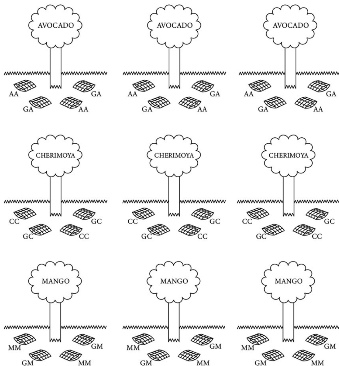
Fig. 2. General scheme of the placement of bagged pruning waste in the sample design.
