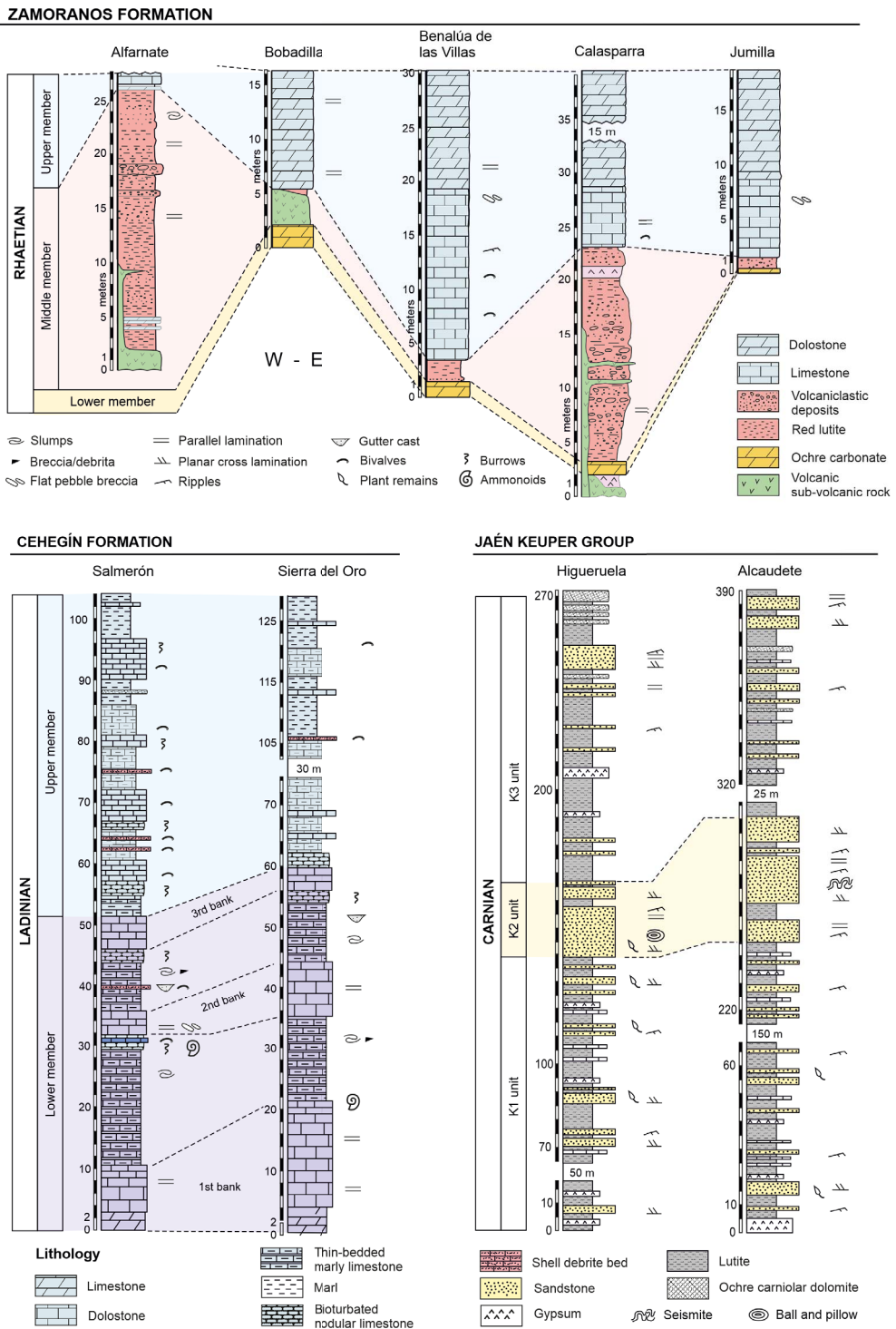
Figure 4. Stratigraphic sections studied representative of the Betic External Zone. See Figure 1 for locations. The sections of the Zamoranos Fm are modified from Pérez-López et al. [2021b].
