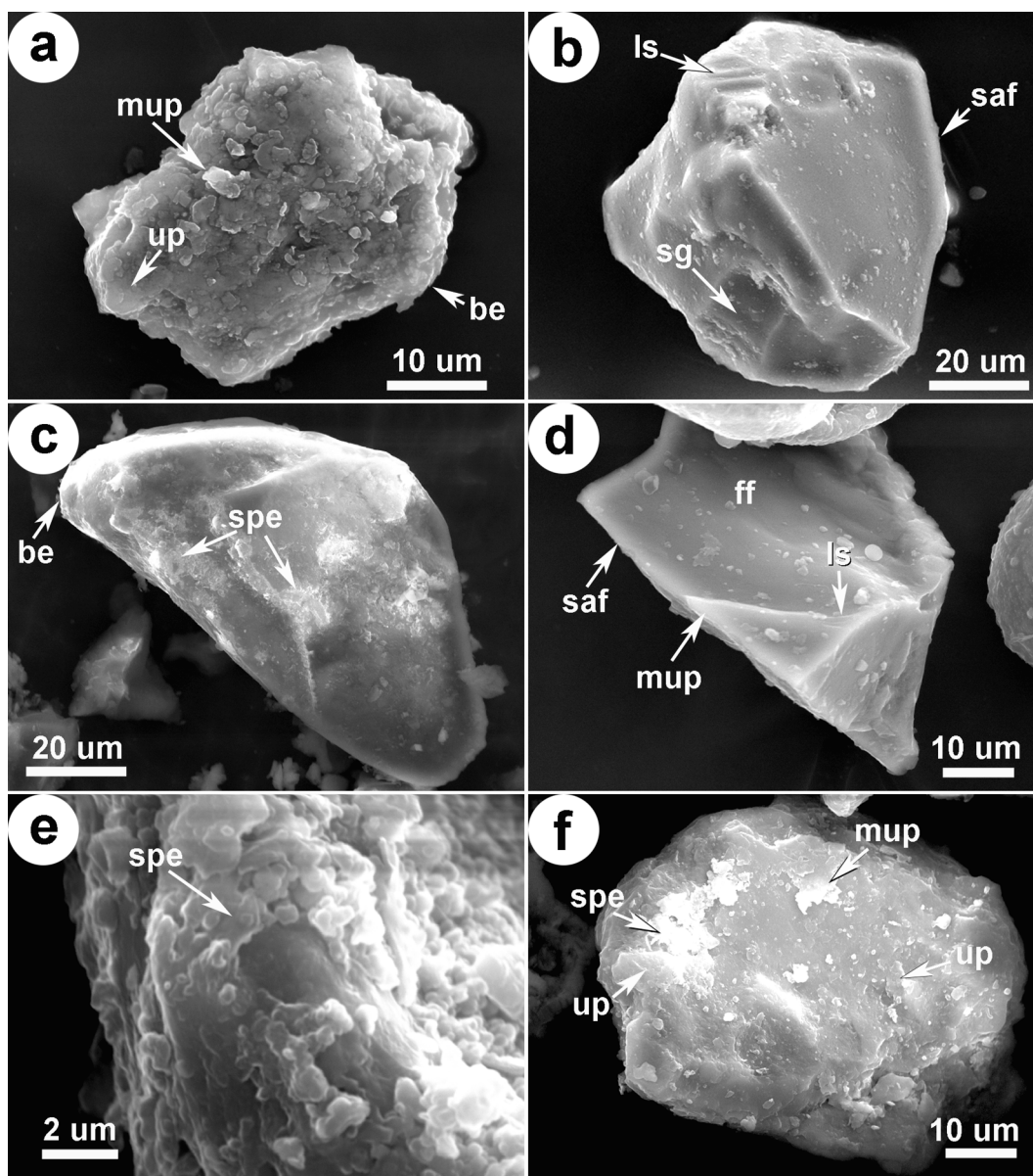
Fig. 4. SEM images of quartz grains: a) 4PA sample. Medium relief polycrystalline grain (43 \mu\text{m} maximum diameter), subrounded, whit typical aeolian microtextures, namely, upturned plates (up), bulbous edges (be), and mechanically upturned plates (mup); b) 4PA sample. Medium relief monocrystalline grain (59 \mu\text{m} long) in which crystal faces are recognised. Clear surface, subrounded perimeter with mechanical microtextures, namely, sharp angular features (saf), linear steps (ls), and straight grooves (sg); c) 16PA sample. Low relief polycrystalline grain (102 \mu\text{m} long). Typical aeolian microtextures, namely, rounding, bulbous edges (be), silica pellicle (spe), and polished surface, are observed; d) 4PA sample. Low relief monocrystalline grain (59 \mu\text{m} long). Mechanical microtextures, namely, saf, mup, ls, and fracture face (ff), are observed. All these mechanical microtextures denote a fresh-looking aspect (little aeolian evolution); e) 28PA sample. Enlargement of a surface quartz grain showing silica pellicle (spe); f) 28PA sample. Low relief polycrystalline grain (63 \mu\text{m} long) showing silica pellicle (spe) and typical mechanical aeolian microtextures, namely, upturned plates (up) and mechanically upturned plates (mup).
