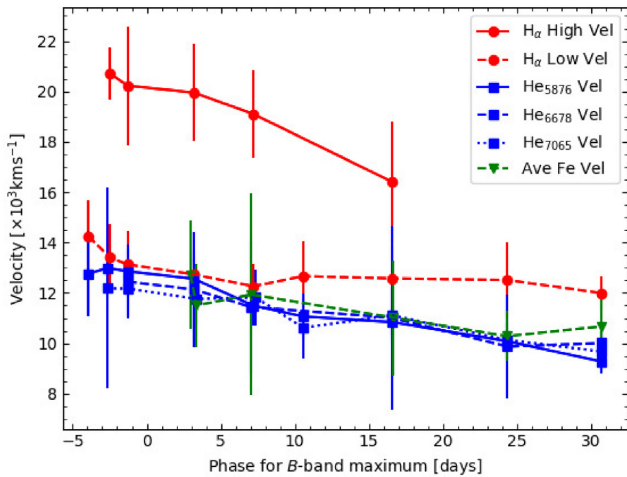
Figure 8. Line velocity evolution of H\alpha , He I, and Fe II from Gaussian fits to the spectra. The H\alpha (red) is split into a high-velocity component and a low-velocity component, shown as the solid line and dashed line, respectively. The evolution of a selection of individual He I spectral lines (blue) are shown as separate curves. Due to the uncertainty in the Fe II lines (green), as a result of the noise in that region of the spectrum, the average line velocity is displayed. The plot is cut-off at \sim 30 d due to the emergence of other lines around the H\alpha region.
