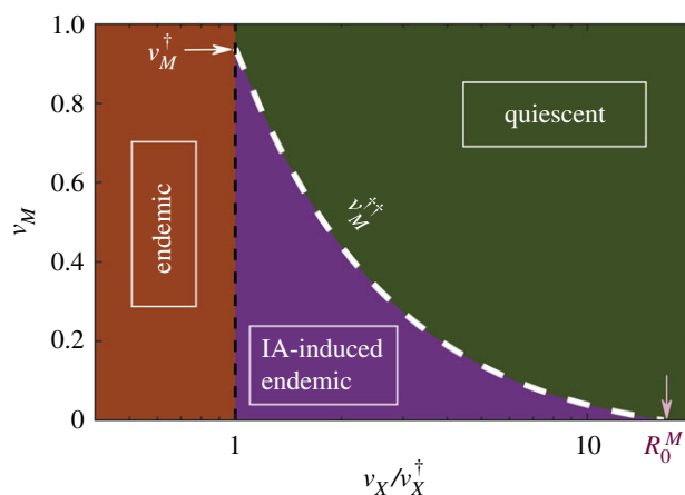
Figure 6. Analytically determined phases for disease X in the SIR-IA model with demography. The white-dashed line depicting the vaccination threshold under IA effects was determined through equation (3.10). The IA-induced endemic phase is bounded by v_X = v_X^{\dagger} , below which the disease is always endemic, independently of IA effects (black-dashed line) and v_X = v_X^{\dagger} R_0^M (marked by the pink arrow), above which the epidemics does not propagate despite the IA contribution. Note that a triple point appears for v_X = v_X^{\dagger} and v_M = v_M^{\dagger} (marked by the white arrow), at which the three phases collide.
