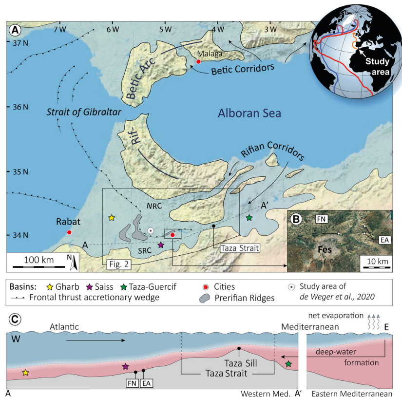
Fig. 1. (A) Satellite terrain image of the westernmost Mediterranean region, southern Spain and north-west Africa. The globe on the right-hand corner shows the location of the study area and depicts the thermohaline circulation pattern (red – shallow; blue – deep), the orange arrow indicates the pathway of the Mediterranean Outflow Water (MOW). In transparent blue a late Miocene palaeogeographic overlay of the Betic and Rifian corridors, NRC = North Rifian Corridor and SRC = South Rifian Corridor, after de Weger et al. (2020). The location of the main geological features, such as the Gharb, Saiss and Taza–Guercif basins, the Prerifian Ridges and the Taza Strait are indicated. (B) Satellite image showing the location of the study areas. The abbreviations stand for the section names; FN = Fes-north and EA = El Adergha. (C) Late Miocene reconstruction through the SRC, cross-section A–A', of which the location is indicated in (A). The SRC accommodated Atlantic–Mediterranean exchange of surficial Atlantic and Mediterranean Deep Water.
