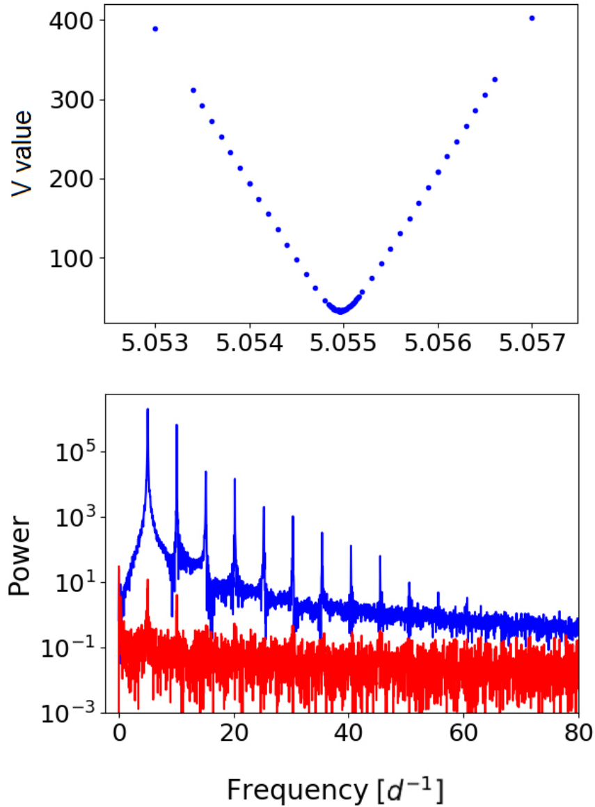
Figure 4.3 Application of the BPM to the light-curve of TIC 9632550. Upper panel: fundamental period found as a local minimum at 5.054963644 \text{ d}^{-1} . Lower panel: in blue, the FFT of the original light-curve; in red, the FFT of the residuals after fitting the fundamental frequency and 13 statistically significant harmonics. Units of power are [(e^-/s)^2] . Source: Lares-Martiz et al. (2020)
