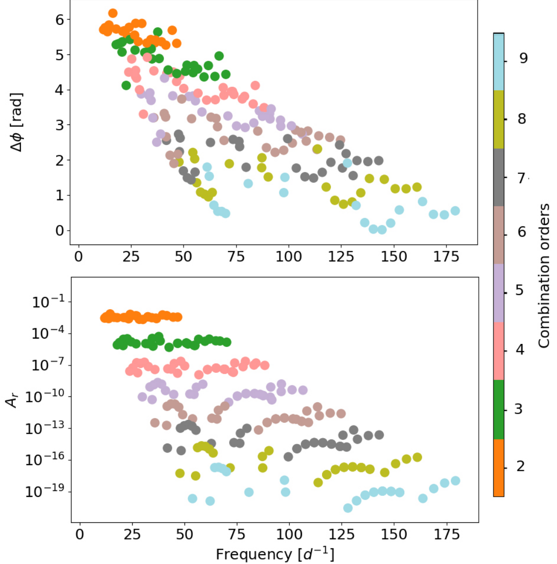
Figure 5.12 First phasor cycle of the relative phases (top panel) and amplitude ratios (bottom panel) plots of alleged NLDP non-linearities of 11 HADS stars (5 monoperiodic and 6 double-mode).
