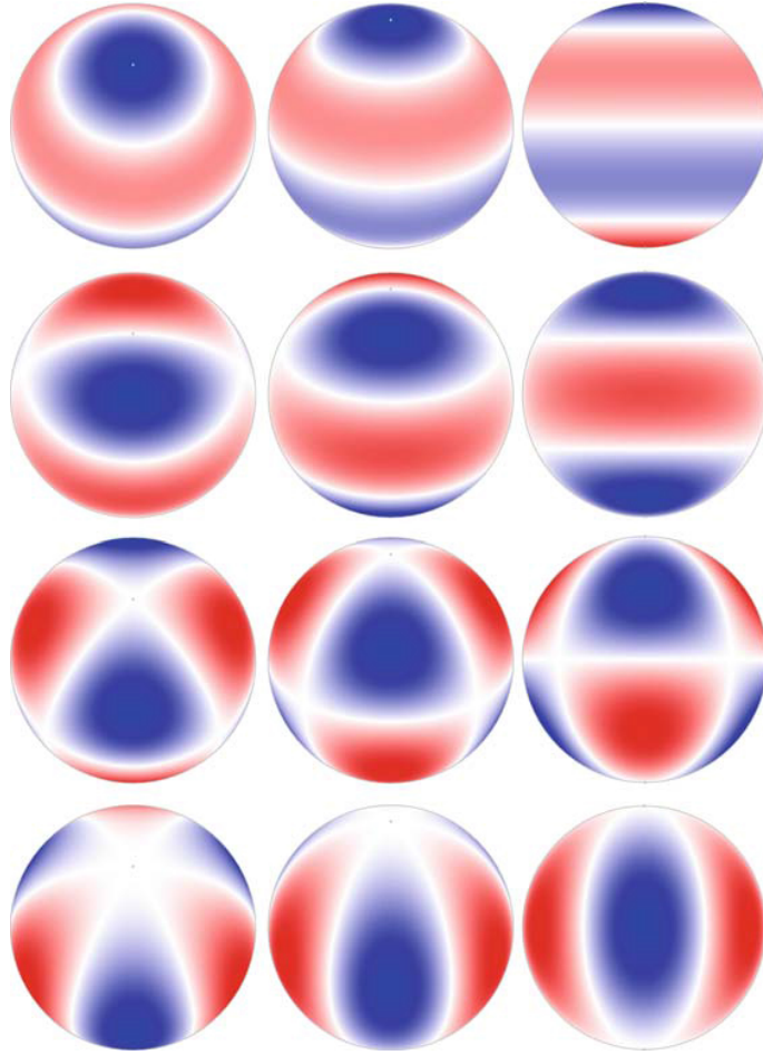
Figure 1.1 Radial and non-radial pulsation modes examples. The columns show the modes from different viewing angles; the left column is for an inclination of the pulsation pole of 30^\circ , the middle column is for 60^\circ , and the right column is for 90^\circ . The white bands represent the positions of the surface nodes; red and blue represent sections of the star that are moving in (out) and/or heating (cooling) at any given time, then vice versa. The top row shows the (l = 3, m = 0) mode, where the nodes lie at latitudes \pm 51^\circ and 0^\circ . The second row shows the (l = 3, m = \pm 1) mode, with two nodes that are lines of latitude and one that is a line of longitude. The third row is the (l = 3, m = \pm 2) mode, and the bottom row shows the (l = 3, m = \pm 3) mode. Rotation distinguishes the sign of m . Source: (Aerts et al., 2010)
