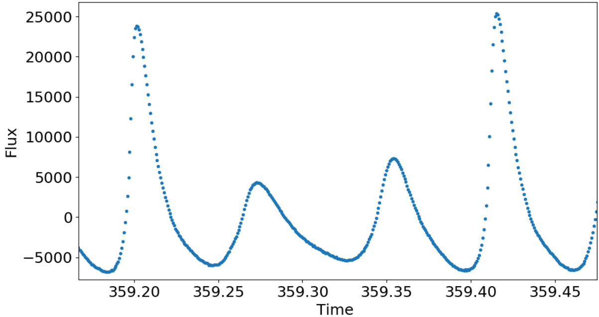
Figure 3.1 Extract of the GSC 00144-03031 light curve observed by CoRoT. Steep ascends and slow descends move away from the characteristic sinusoidal shape.
