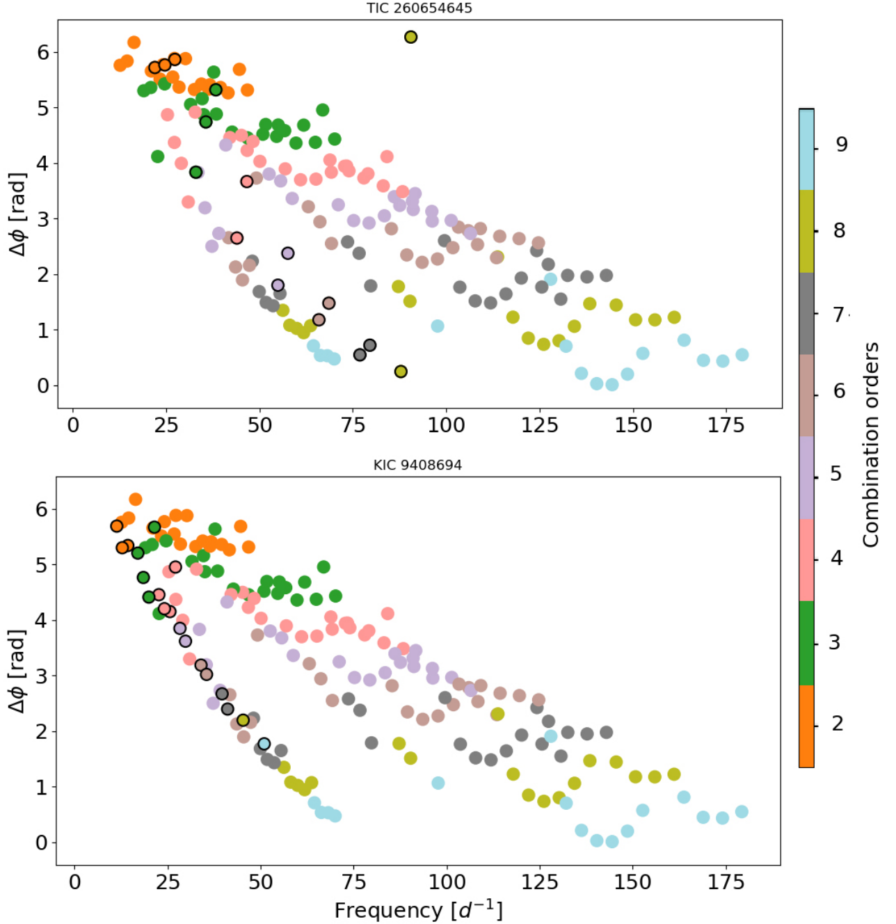
Figure 5.8 Relative phases of 2 peculiar double-mode HADS
