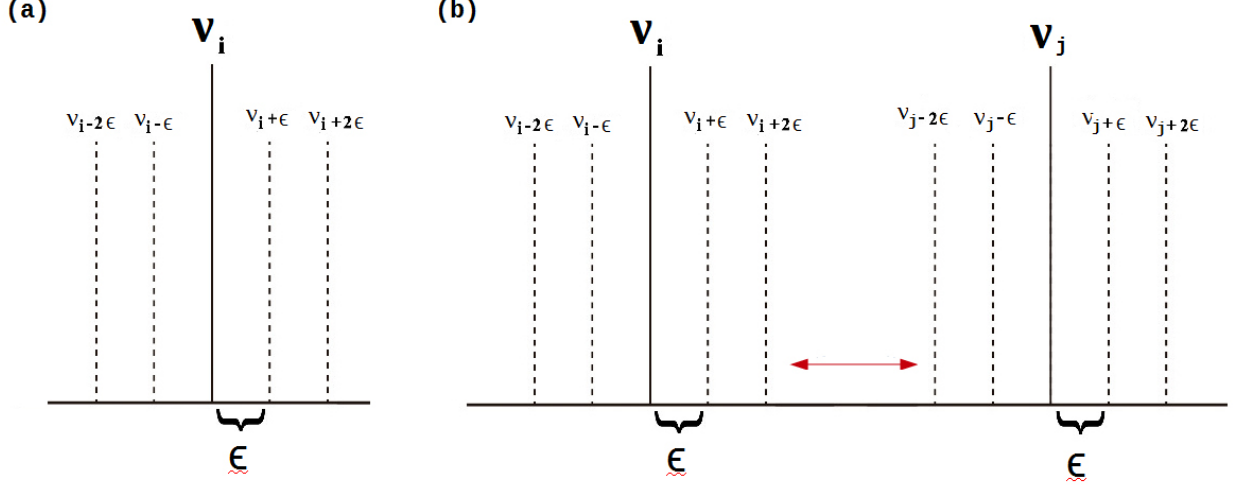
Figure 4.2 Schematic representation of best parent search with n\_exp = 2 . Panel (a) for one parent frequency \omega_i and panel (b) for two parent frequencies \omega_i and \omega_j . The search does not allow overlapping of the possible parents (red arrow)
