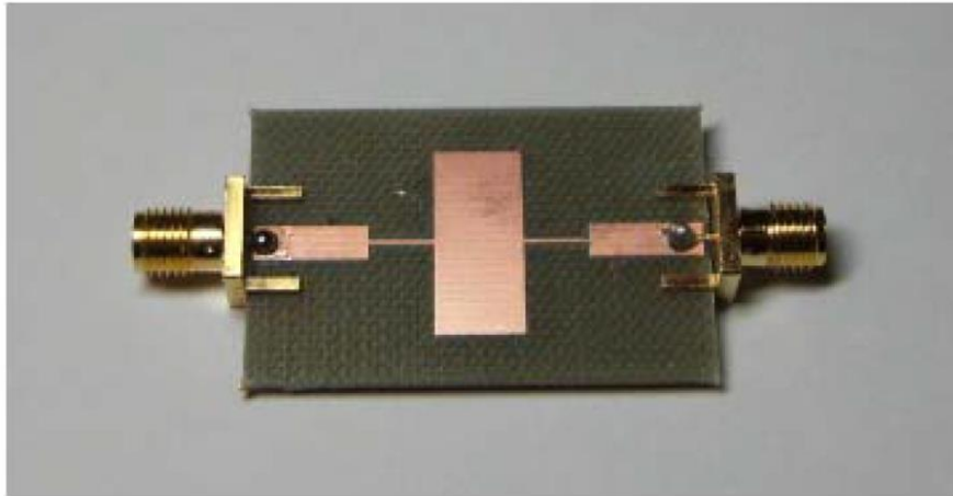
Figure 3. Low-pass filter fabricated from a design carried out with MWSim
