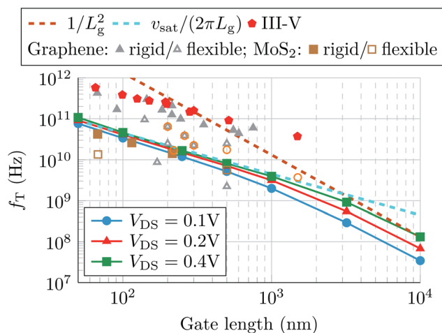
Fig. 5 Cut-off frequency f_{\text{T}} as a function of the gate length for different drain biases (solid lines with markers). The 1/L_g^2 trend and the physical limit (that also serves as a guideline for the 1/L_g scaling) are also depicted (dashed lines). Solid and hollow markers correspond to experimental works. 6,9,12,34-41
