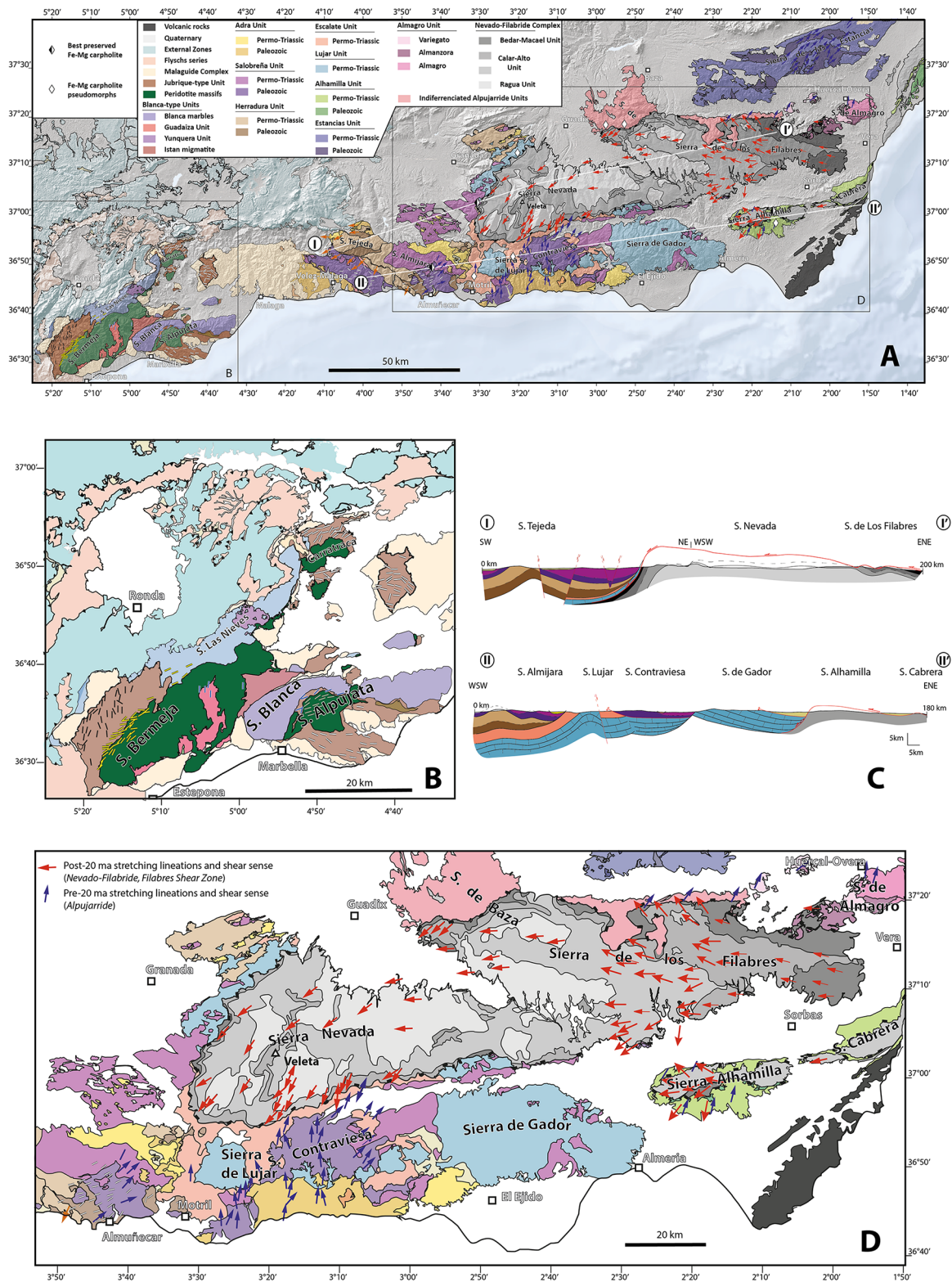
Fig. 4. Geology of the Internal Zones of the Betic Cordilleras. A: tectonic map showing the different units of the Alpuj rride and Nevado-Filabride complexes. White lines are the cross-sections of Figure 4C. The preservation of Fe-Mg-carpholite is shown. B: Detailed map of the western Alpuj rride complex with the directions of stretching lineations from Williams and Platt (2018) and Bessi re (2019). C: Two E-W cross-sections. D: Detailed map of the central and eastern Alpuj rride with lineations and sense of shear after Jabaloy et al. (1993), Augier et al. (2005b, 2013), Jolivet et al. (2008).
