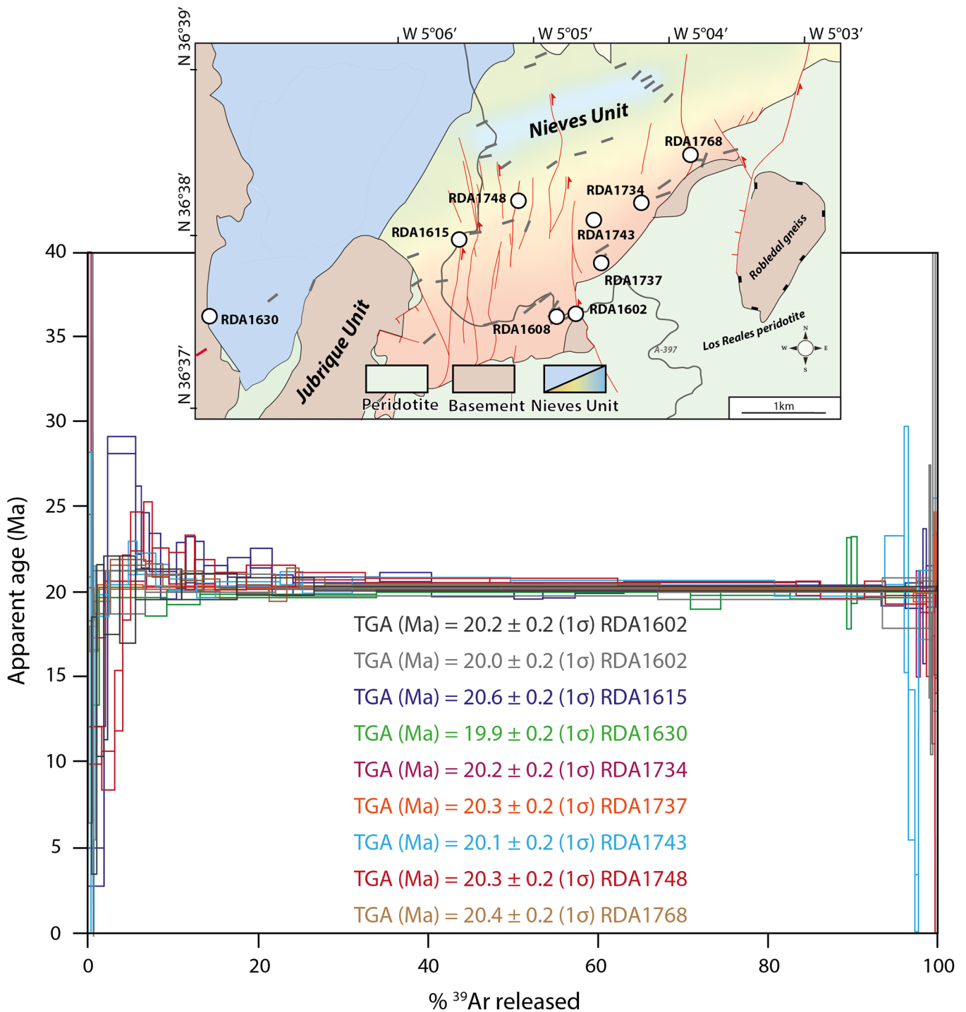
Fig. 13. New 40 Ar/ 39 Ar step-heating ages of phlogopites from marbles sampled near the contact with the peridotite. Data after Bessière (2019).
