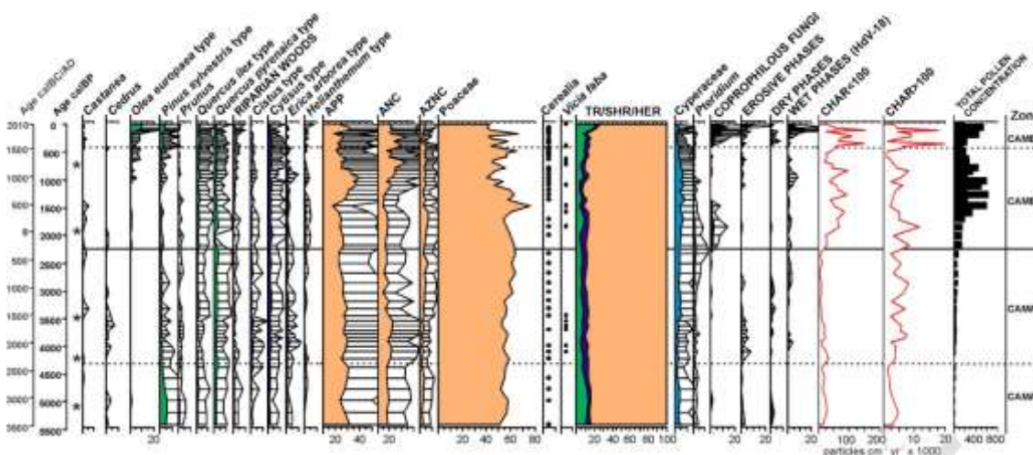
Figure 4. Summary diagram of Dehesa del Camarate (DC), including selected pollen types, NPPs, CHAR and Total Pollen Concentration. APP: Anthropogenic Perennial Pastures; ANC: Anthropogenous Nitrophilous Communities; AZNC: Anthropozoogenous Nitrophilous Communities; TR: Trees (= Arboreal Pollen –AP-); SHR: Shrubs; HER: Herbs; Stars indicate Radiocarbon datings.
