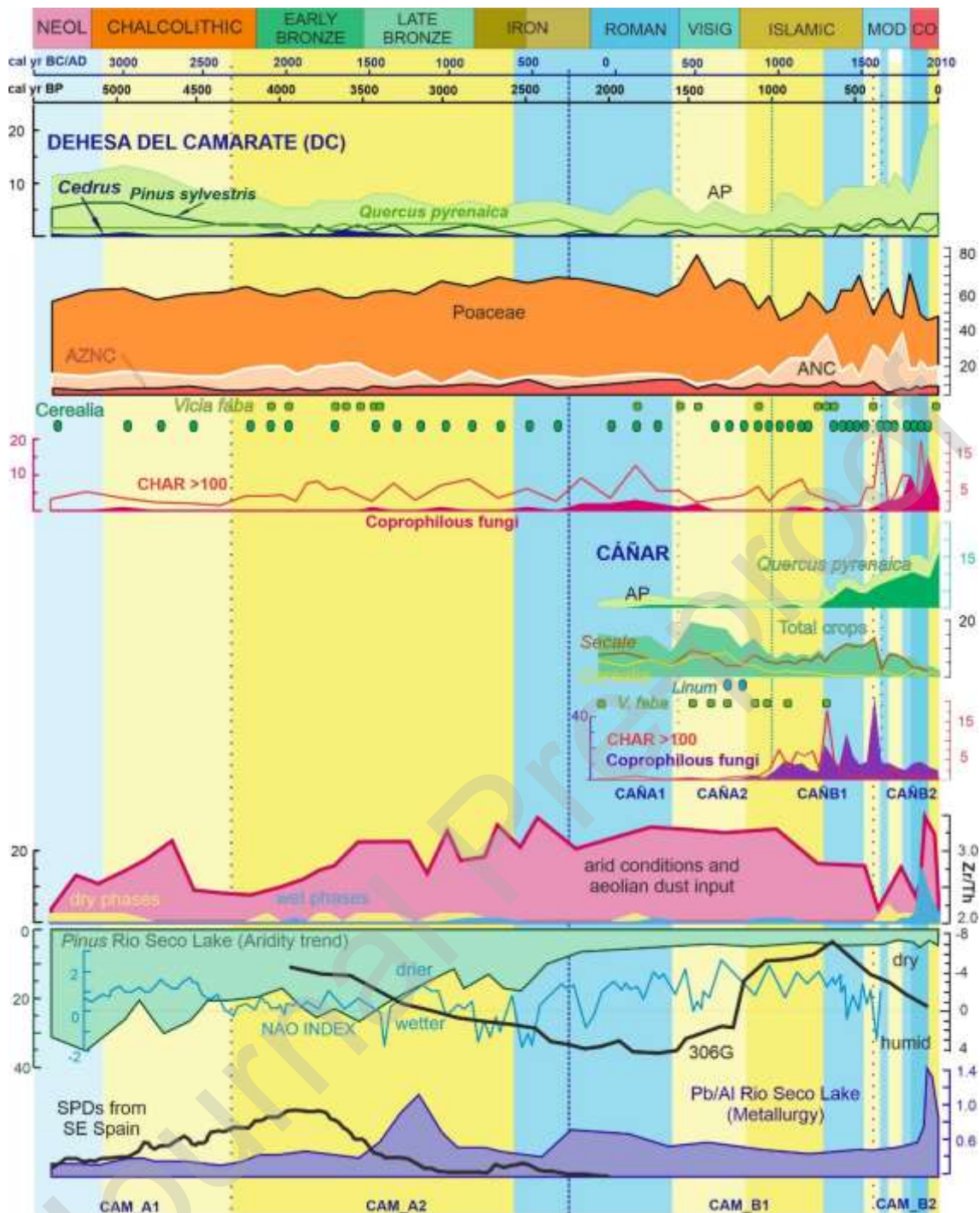
Figure 6. Main environmental changes in Sierra Nevada during the last 5300 years based on the analysis of Dehesa del Camarate (DC) and Cañar mires. (Aeolian dust input from Jiménez-Espejo et al., 2014; Aridity trend of Río Seco Lake from Anderson et al., 2011; Dry versus humid climate conditions of the west Balearic-Algerian Basin 306G core from Nieto-Moreno et al., 2011; NAO Index from Olsen et al., 2012; Palaeodemographic proxy (SPDs) for SE Spain from Fyfe et al., 2019; Pb/Al of Río Seco Lake from García-Alix et al., 2013). Humid (blue) and Dry (yellow) phases have been set based on Martín-Puertas et al., 2010; Nieto-Moreno 2011; 2013; and García-Alix et al., 2017. MOD: Modern Period; CO: Contemporary Period.
