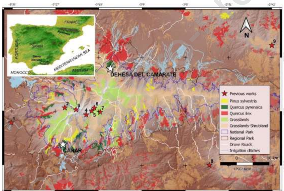
Figure 1. Location of Dehesa del Camarate and Cañar mires (white stars), showing the location of previous palynological works cited in the text (red stars): 1. Padul (Ramos-Román et al., 2018a, 2018b; Camuera et al., 2018, 2019); 2. Laguna de la Mula (Jiménez-Moreno et al., 2013); 3. Borreguiles de la Virgen (Jiménez Moreno and Anderson, 2012); 4. Laguna de Río Seco (Anderson et al., 2011); 5. Laguna de la Mosca (Manzano et al., 2019); 6. Borreguil de la Caldera (Ramos-Román et al., 2016); 7. Laguna Hondera (Mesa-Fernández et al., 2018); 8. Sierra de Gádor (Carrión et al., 2003); 9. Sierra de Baza (Carrión et al., 2007)
