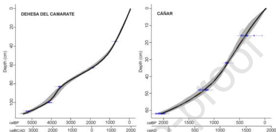
Figure 3. Age-depth models for Dehesa del Camarate and Cáñar mires
