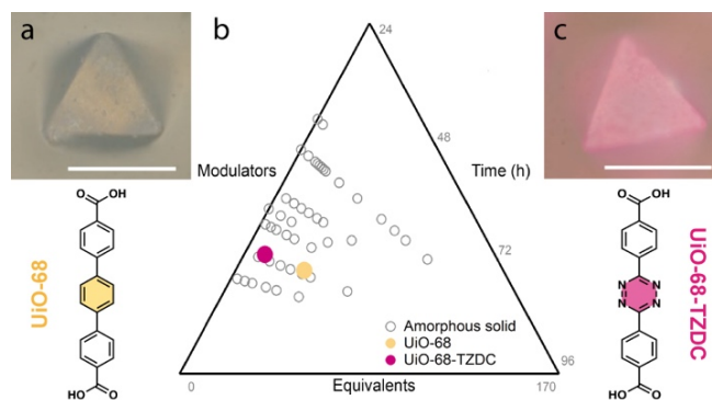
Figure 1. a) Size and morphology of UiO-68. Scale bars correspond to 50 \mu\text{m} . b) Summary of the synthetic conditions explored with automated HT synthesis to identify crystal
