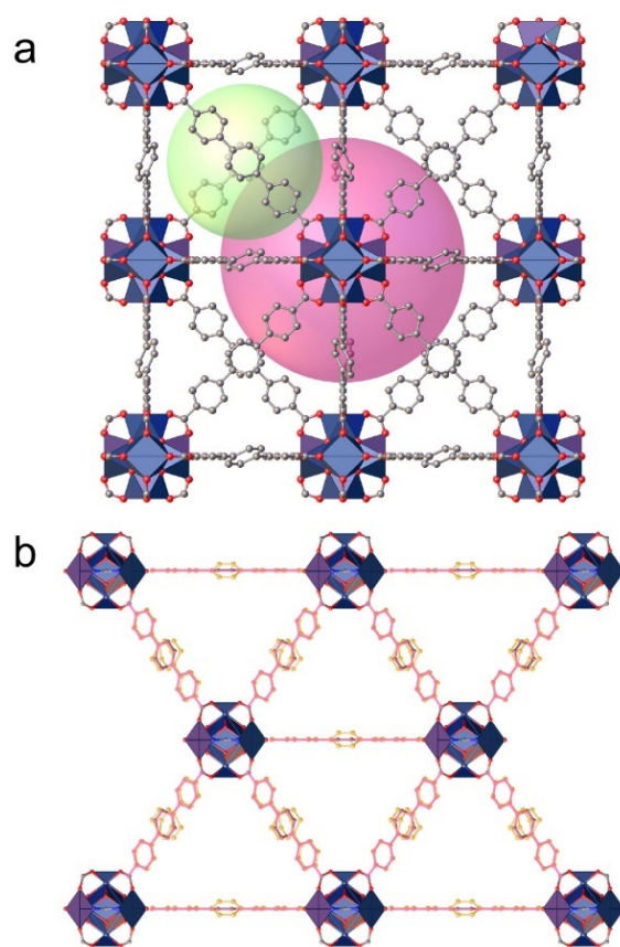
Figure 2. a) Structure of UiO-68 along the c axis showing the accessible volume corresponding to octahedral (purple sphere) and tetrahedral voids (green). b) Overlay of the two crystallographic-distinct linker structures in (011) showing the slight differences that result from the replacement of TPDC with TZDC.
