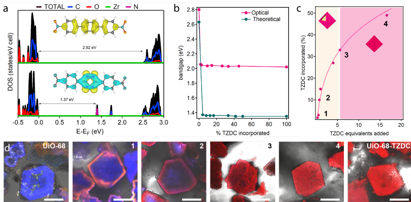
Figure 4. a) Total (DOS, black) and projected (PDOS for each atoms) density of states for pristine UiO-68 (top) and UiO-68-TZDC 4% , (bottom) calculated by using PBE functional, this is a qualitative approach; the electronic structures could not be computed at the HSE06 level because of the system size. Inset: orbitals contributing to the HOCO and LUCO localised on ligand. b) Match between the band gap values' trend described by experimental results and computer calculations. c) Spatial linker arrangement in UiO-68-TZDC x samples (deep orange area for core-shell distribution and pink area for random distribution). d) Fluorescence confocal microscope's
