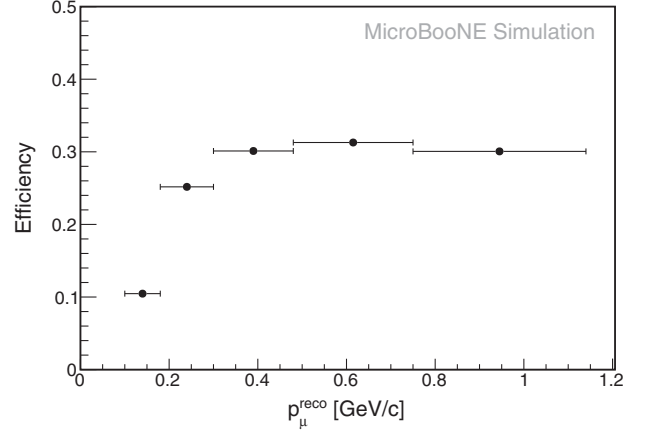
FIG. 14. Efficiency as a function of reconstructed p_\mu in simulated CC0\pi Np events. Statistical error bars are too small to be seen.
