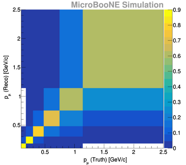
FIG. 15. Migration matrix between true and reconstructed bins for reconstructed muon momentum ( p_\mu ) in simulated CC0\pi Np events.
