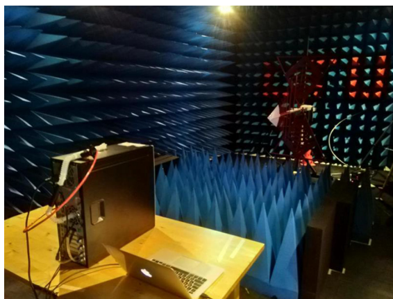
Fig. 23. ATMO-Vent undergoing EMC Testing in the Anechoic chamber at Luleå University of Technology, Sweden.
