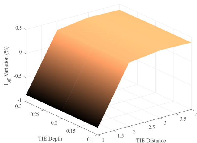
FIGURE 9. Relative leakage current vs the variation of the depth and distance of both ties (relative to the configuration without ties).
