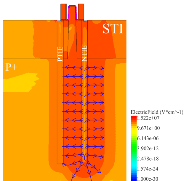
FIGURE 5. FinFET type N 2D cross section (A-A' of Fig. 2) with the well ties in both sides of the device. NTIE is the trench with N++ doping, and PTIE the P++ trench. Arrows point out the direction of the electric field.
