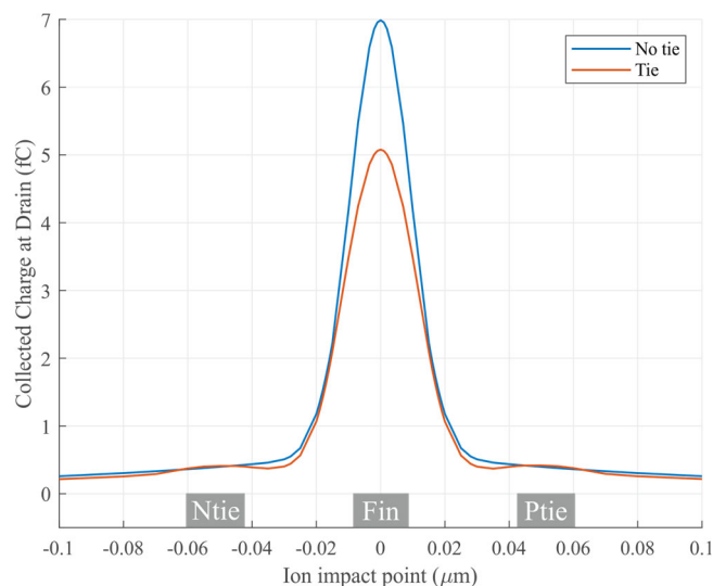
FIGURE 10. Collected charge by the drain vs ion impact point relative to the distance to the fin center, direction (A-A', Fig. 2), with a LET 10 MeV-cm 2 /mg, crossing over the middle of the gate, with and without tie trenches
