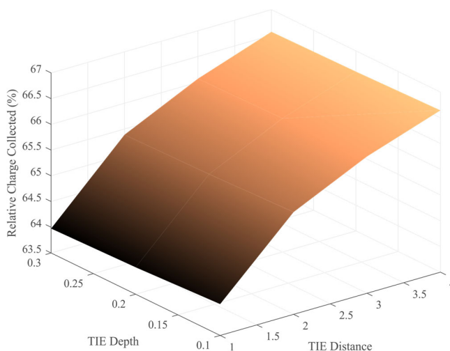
FIGURE 8. Relative charge collected by the drain terminal compared with the conventional design, changing the distance and the depth of the tie trenches
