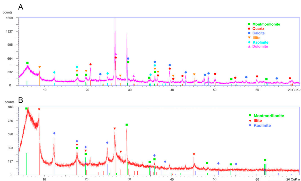
Figure 5. X-ray diffraction patterns of (A) powder samples and (B) oriented samples (<2 \mu\text{m} fraction) from the clay-rich layer of the Diezma landslide.
