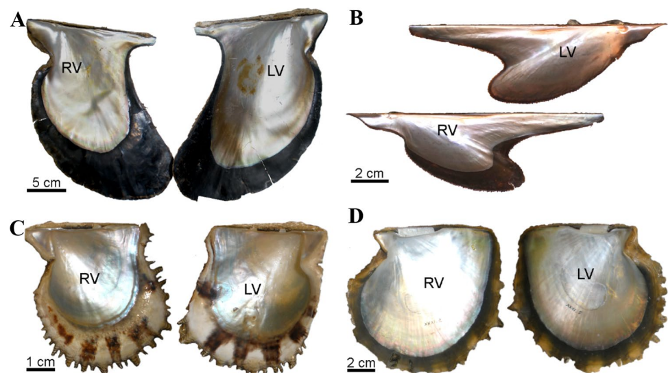
Fig. 1 Internal views of selected species of pterioids. a Pteria penguin (Noumea, New Caledonia), MNHN Paris. b Pteria crocea (Caubian Island, Philippines), UGR. c Pinctada fucata (Japan), MNHN Paris. d Pinctada margaritifera , original in Ranson (1961). (Mahé Island, Seychelles), MNHN Paris. LV left valve, RV right valve
