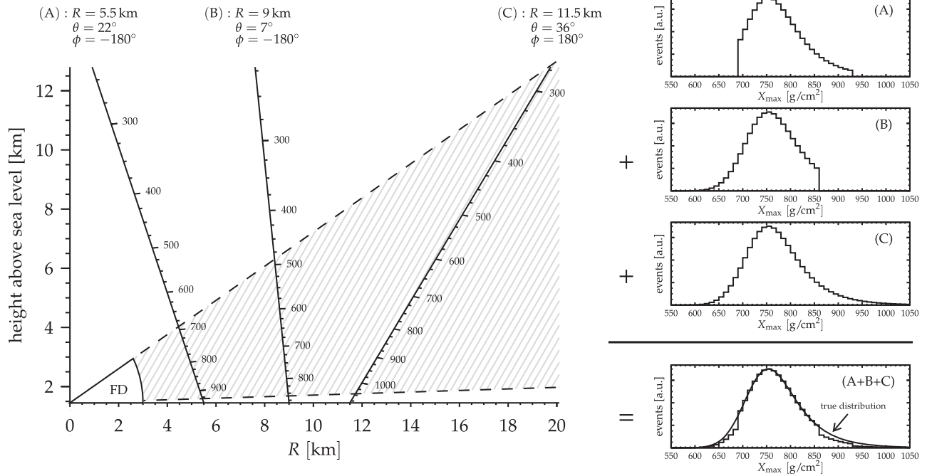
FIG. 2. Illustration of the influence of the FD field of view on the sampling of the X_{\text{max}} distribution. The slant-depth axes in \text{g/cm}^2 are shown on the left panel for three different examples of event geometries (A), (B) and (C) with different ground distances R , zenith angle \theta and azimuthal angle \phi . The FD field of view is indicated by the hatched area inside the dashed lines. Examples of correspondingly truncated X_{\text{max}} distributions are shown on the right panel together with their sum. For the purpose of this illustration, the same number of events for each geometry has been assumed.
