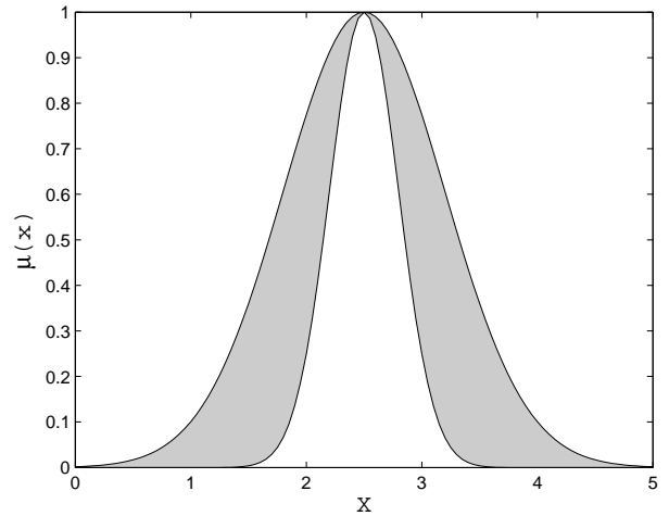
Fig. 4. Example of an interval-valued fuzzy set.
