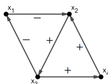
Figure 1. Signed digraph.
