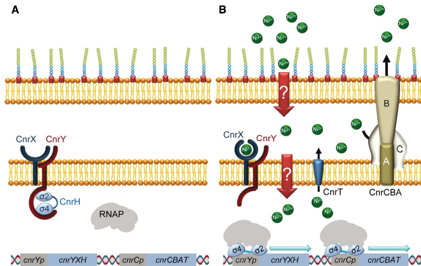
Fig. 3. Mechanism of action of the C. metallidurans CnrH sigma factor.
