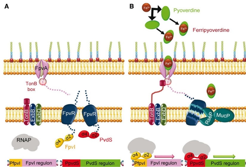
Fig. 2. The P. aeruginosa ferrityoverdine CSS is regulated by FpvR/FpvI/PvdS.
