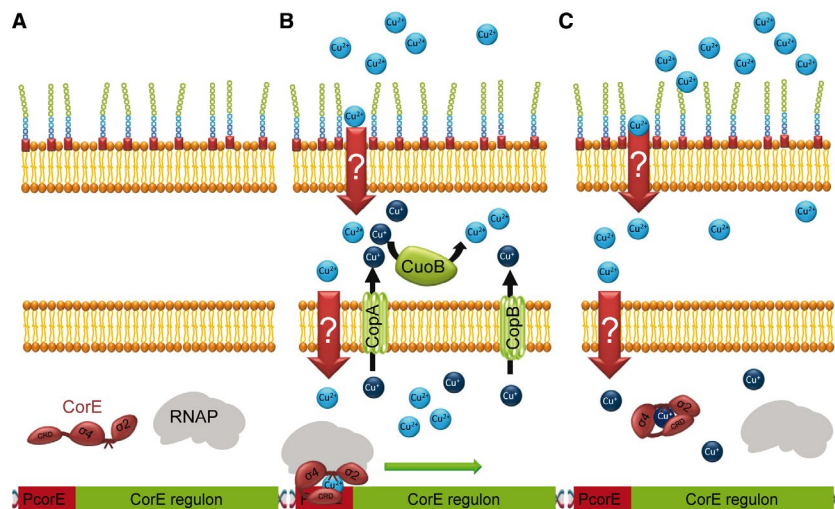
Fig. 5. Mechanism of action of the M. xanthus CorE sigma factor.
