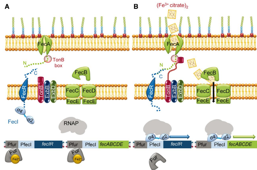
Fig. 1. The E. coli CSS \text{Fe}^{3+} -citrate transport is regulated by the FecR/FecI system.
