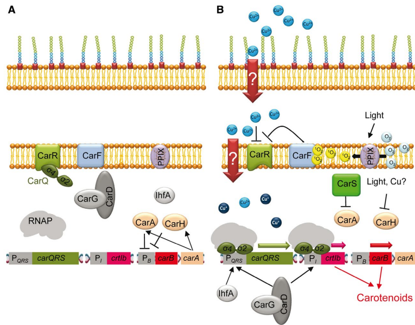
Fig. 4. Mechanism of action of the M. xanthus CarQ sigma factor.
