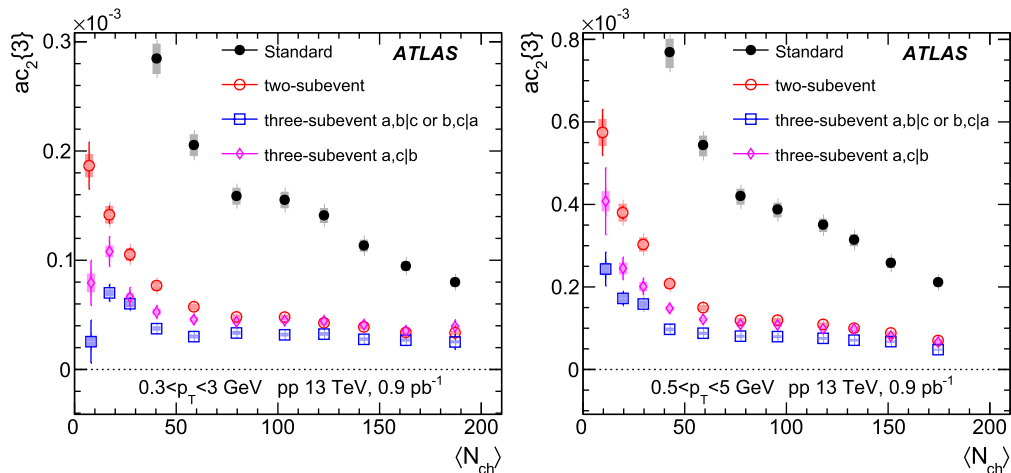
Fig. 10. The a_2\{3\} in 0.3 < p_T < 3 GeV (left panel) and 0.5 < p_T < 5 GeV (right panel) in pp collisions. In each panel, they are compared between standard method (solid circles), two-subevent method (open circles), three-subevent where V_4 is determined in subevent a or c (open boxes), and three-subevent where V_4 is determined in subevent b (diamonds) according to Eq. (8). The error bars and shaded boxes represent the statistical and systematic uncertainties, respectively.
