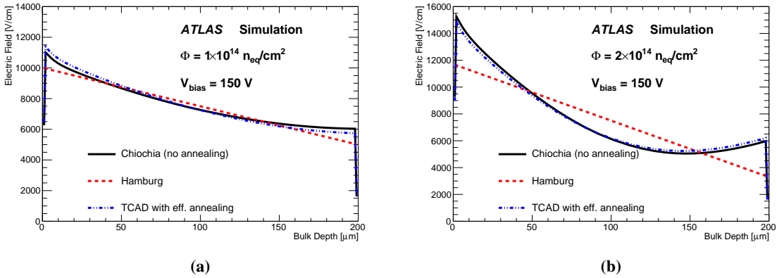
Figure 10. The z dependence of the electric field in a simulated ATLAS IBL planar sensor, averaged over x and y , for simulated fluences of (a) \Phi = 1 \times 10^{14} \text{n}_{\text{eq}}/\text{cm}^2 and (b) 2 \times 10^{14} \text{n}_{\text{eq}}/\text{cm}^2 . The bias voltage was set to 150 V in all cases. Three scenarios — Chiochia (no annealing), Hamburg and TCAD with effective annealing — to emulate annealing effects were simulated.
