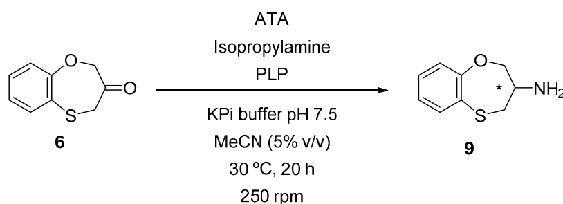
Scheme 2. Biotransamination of 3,4-dihydro-2H-1,5-benzoxathiepin-3-one ( 6 ) into amine 9 , using ATAs.
