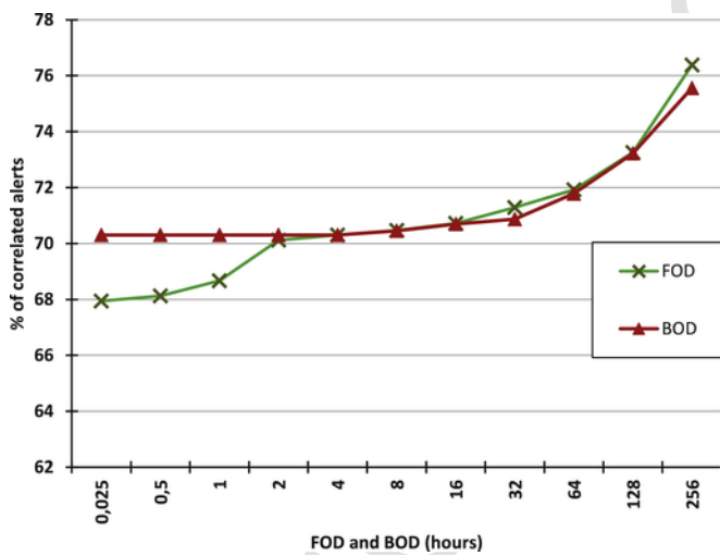
Fig. 11. Percentage of correlated alerts at different values for FOD and BOD.
