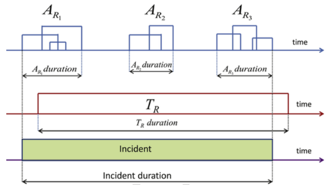
Fig. 3. Example of alert aggregation using the proposed model.
