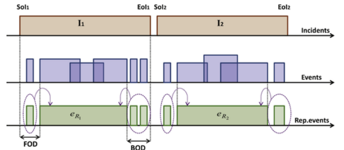
Fig. 8. Example showing the problem of directly applying the basic event correlation model to two consecutive incidents.
