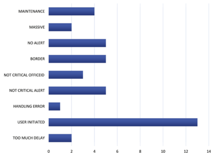
Fig. 15. Results from the analysis of the uncorrelated tickets.
