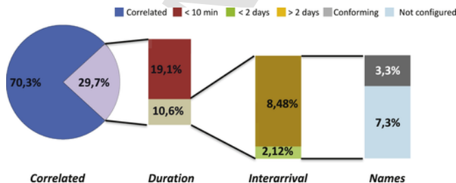
Fig. 14. Distribution of the number of raw alerts among the different assessment criteria.
