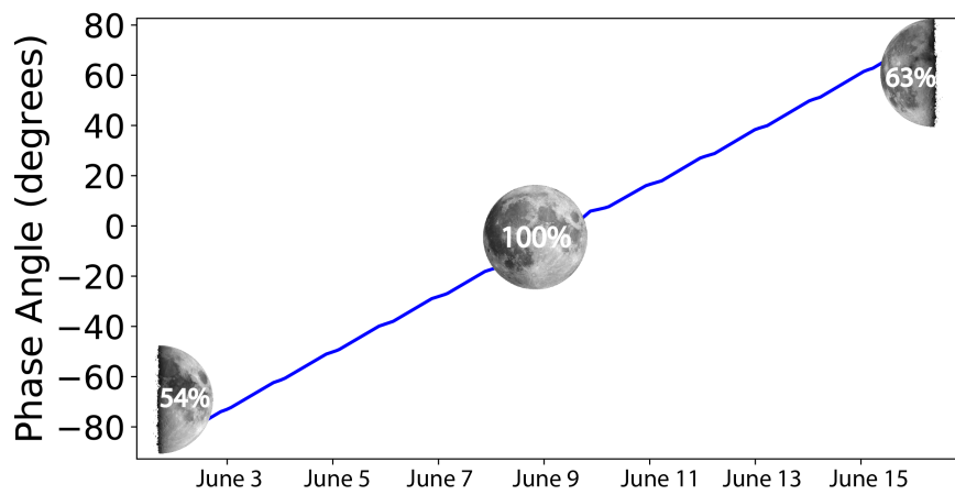
Figure 1: Phase angle evolution (in degrees) during the measurement period in the nocturnal field campaign.
