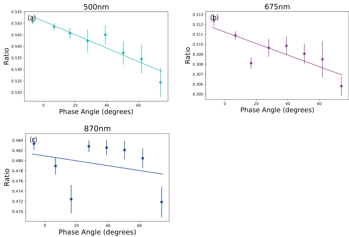
Figure 7: Ratios of raw signals (night-time only) with the Moon's phase angle (in degrees) between the LunarPFR and the master Cimel (CE#971) for the three near coincident spectral bands: (a) 500, (b) 675 and (c) 870 nm. Solid line represents the x-y linear fitting.
