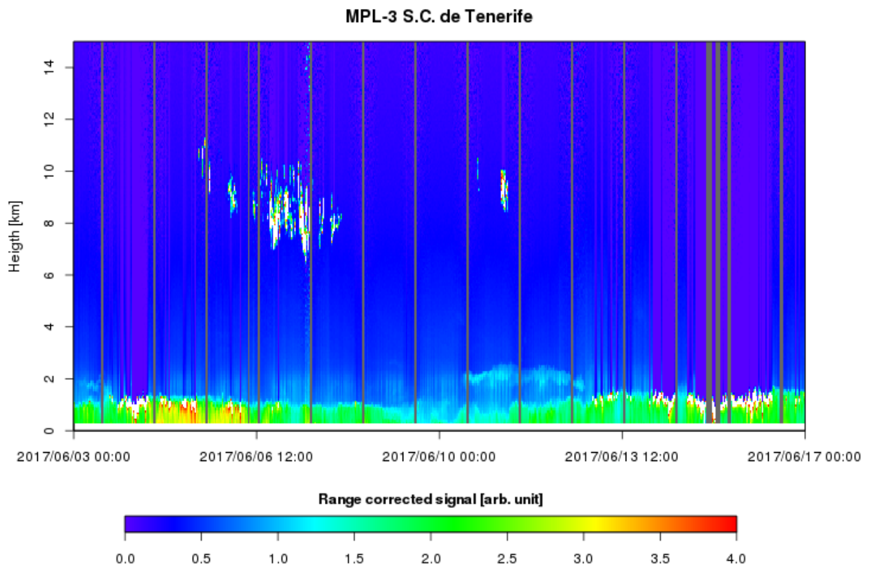
Figure 2: Micro-Pulse Lidar (MPL-3) range corrected signals at 523 nm obtained at Santa Cruz de Tenerife station (60 m a.s.l.). Grey vertical lines represent the absence of measurements due to rain or direct solar incidence in the detector at noon.
