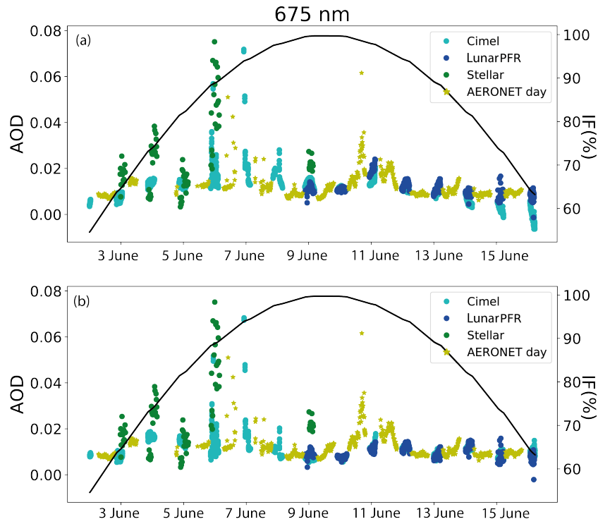
Figure 12: AOD time series for master Cimel CE#971 (at 674.8 nm), LunarPFR (at 675.6 nm), stellar (at 670.0 nm) and daytime AERONET (at 675.7 nm) in the period 2-17 June 2017. AOD from lunar photometers have been extracted by means of (a) Lunar-Langley calibration with the RIMO model, and (b) Langley-plot calibration with V_0^c values. The black line and right y axis correspond to the evolution of the Moon's illumination factor (IF, in %) in this period.
