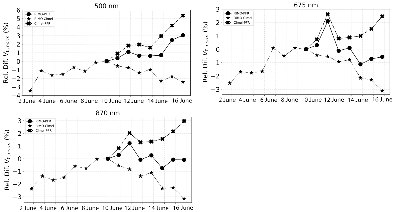
Figure 9: Relative difference of normalized V_0^c (in %) between Cimel and LunarPFR, as well as between these two instruments and the V_0 computed from the RIMO model, for 500, 675 and 870 nm spectral bands.
