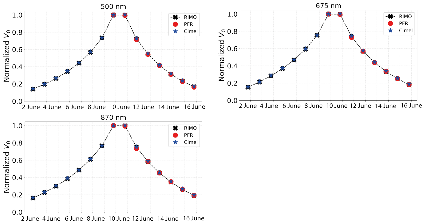
Figure 8: Evolution during the field campaign of the normalized V_0^c computed from Cimel, LunarPFR and RIMO data, for 500, 675 and 870 nm spectral bands.
