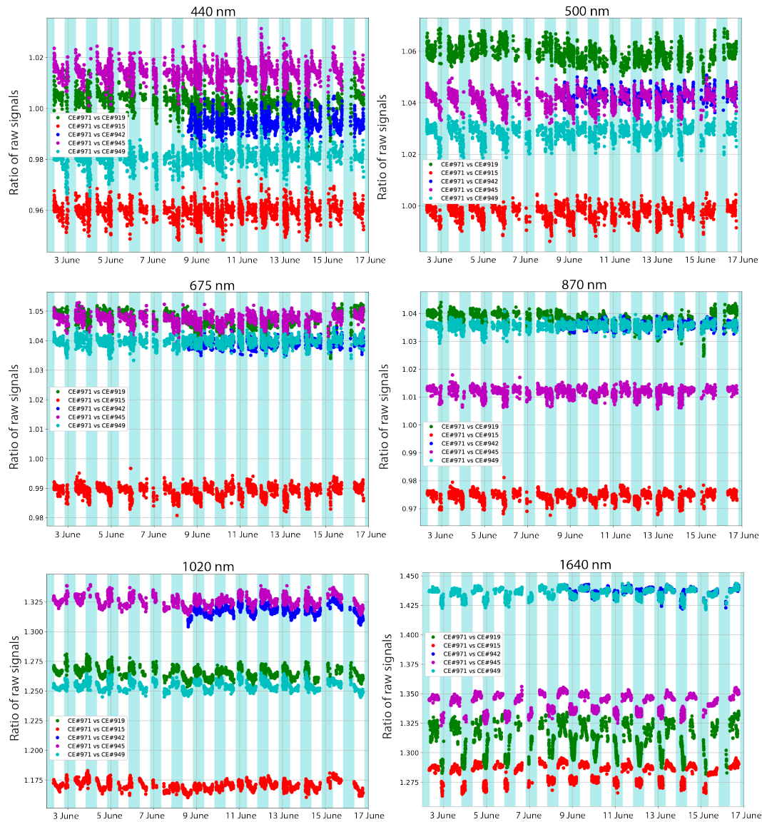
Figure 6: Ratios of digital counts (dark current corrected) between the master Cimel (CE#971) and the five secondaries for the six different Cimel spectral bands at Izaña, between June 2 and 17, 2017. Night-time data is shaded in blue.
