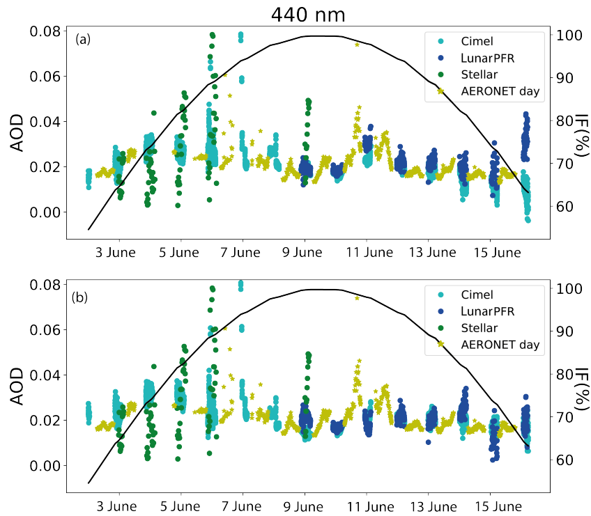
Figure 10: AOD time series for master Cimel CE#971 (at 439.5 nm), LunarPFR (at 412.4 nm), stellar (at 436.8 nm) and daytime AERONET (at 439.7 nm) in the period 2-17 June 2017. AOD from lunar photometers have been extracted by means of (a) Lunar-Langley calibration with the RIMO model, and (b) Langley-plot calibration with V_0^c values. The black line and right y axis correspond to the evolution of the Moon's illumination factor (IF, in %) in this period.
