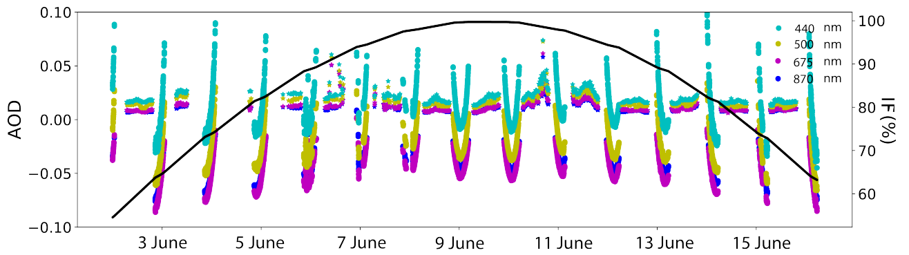
Figure 16: Nocturnal AOD time series for master Cimel CE#971 (displayed with circles) in the period 2-17 June 2017, for four spectral bands (870, 675, 500 and 440 nm). AODs have been extracted by means of the Sun-Moon Gain Factor calibration. Daytime AODs from AERONET are also displayed with asterisks. The black line and right y axis correspond to the evolution of the Moon's illumination factor (IF, in %) in this period.
