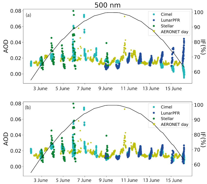
Figure 11: AOD time series for master Cimel CE#971 (at 500.6 nm), LunarPFR (at 500.7 nm), stellar (at 500.7 nm) and daytime AERONET (at 500.8 nm) in the period 2-17 June 2017. AOD from lunar photometers have been extracted by means of (a) Lunar-Langley calibration with the RIMO model, and (b) Langley-plot calibration with V_0^c values. The black line and right y axis correspond to the evolution of the Moon's illumination factor (IF, in %) in this period.
