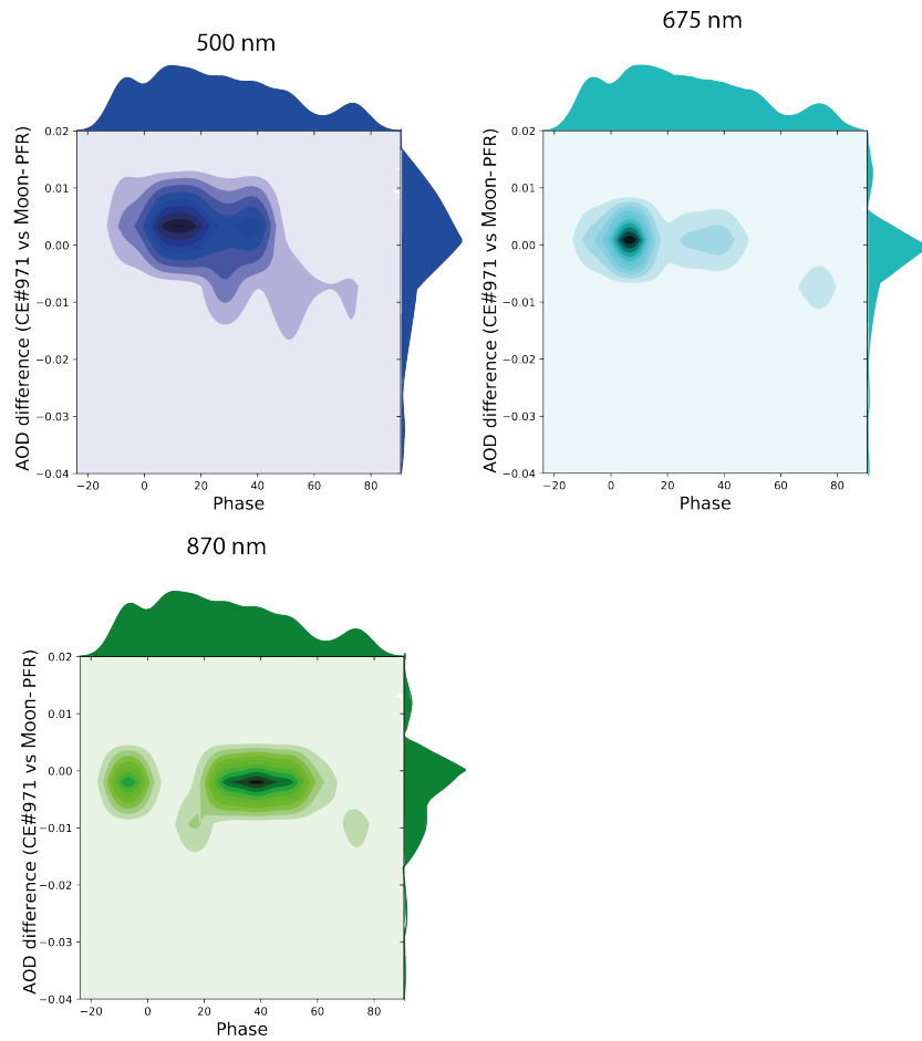
Figure 14: Bivariate kernel density estimate plots of AOD difference (between CE#971 and LunarPFR) and the Moon's phase angle, calculated with RIMO, for the three coincident spectral bands. Univariate density distribution of each variable is displayed on separate axes.
