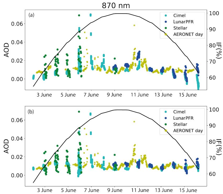
Figure 13: AOD time series for master Cimel CE#971 (at 870.4 nm), LunarPFR (at 861.3 nm), stellar (at 879.5 nm) and daytime AERONET (at 869.8 nm) in the period 2-17 June 2017. AOD from lunar photometers have been extracted by means of (a) Lunar-Langley calibration with the RIMO model, and (b) Langley-plot calibration with V_0^c values. The black line and right y axis correspond to the evolution of the Moon's illumination factor (IF, in %) in this period.
