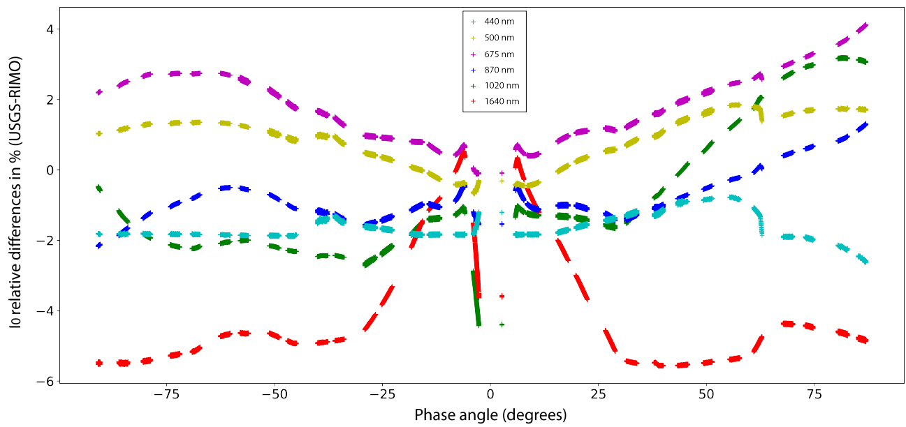
Figure 3: Relative differences between I_0 from USGS/ROLO and RIMO in June-July 2017 at Izaña for the Cimel wavelengths.
