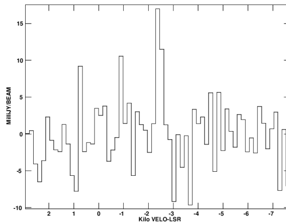
Figure 4.15: Spectrum taken at the peak of the CCS emission from our GF9-2 map.
