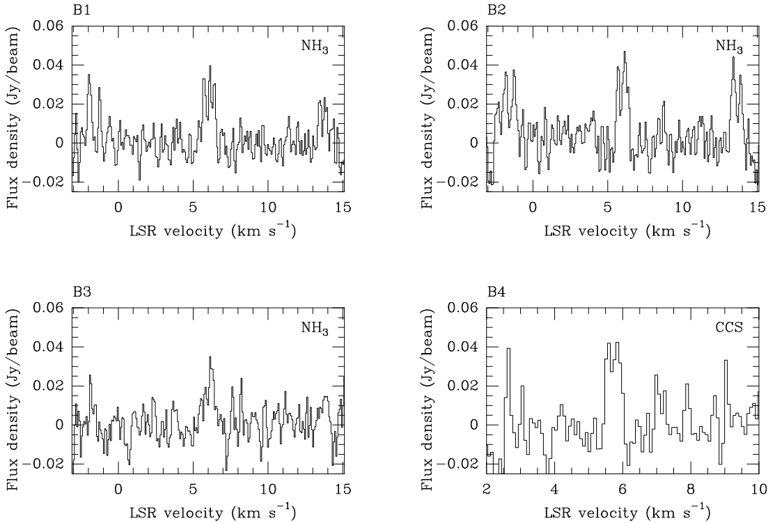
Figure 3.3: Spectra of the \text{NH}_3 (1,1) transition for fields B1, B2 and B3 and CCS transitions (field B4) integrating over an area of about 10'' around the peak emission of each field.
