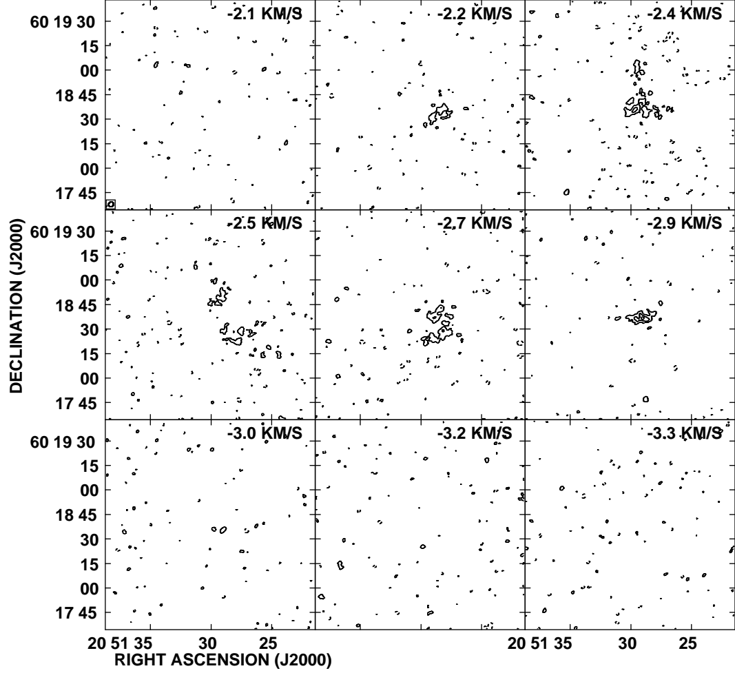
Figure 4.12: Velocity channels for the \text{NH}_3 (2,2) transition in the GF9-2 region. The beam is shown at the bottom left corner of the first panel. Contours are -3, 3, 6, 9 and 12 times 2.5 \text{ mJy beam}^{-1} (the r.m.s. of our map).
