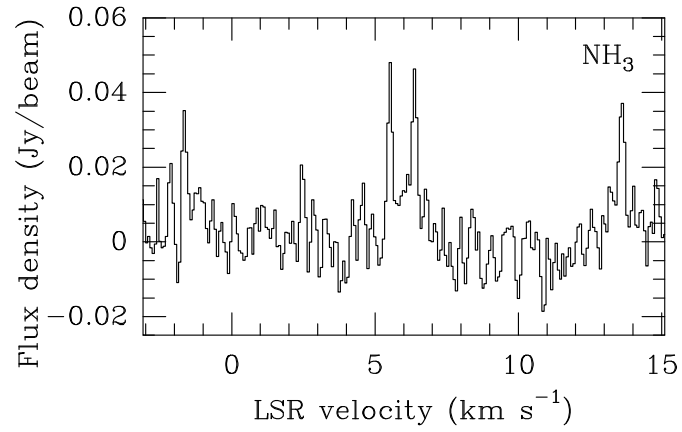
Figure 3.7: Spectra at the position of the highest value of velocity dispersion.
