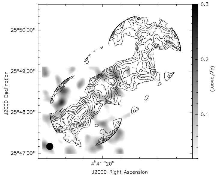
Figure 3.8: Overlay of our \text{NH}_3 (1,1) mosaic (contours) and CCS J_N = 2_1 - 1_0 map (greyscale) of TMC1 B. Contours are the same as Fig. 3.5. The greyscale is shown at the right side of the map.
