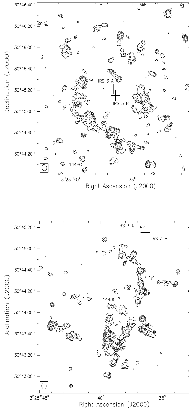
Figure 6.5: Integrated velocity map for the CCS ( J_N = 2_1 - 1_0 ) transition in the regions L1448-IR3 (top) and L1448C (bottom). Contours are -6, -3, 3, 4, 5, 6, 7, 8, 9, 10 and 11 times 17.24 \text{ Jy beam}^{-1} \text{ Hz} (the r.m.s. of our map). For L1448C map, Contours are -6, -3, 3, 4, 5, 6, 7, 8, 9, 10 and 11 times 23.34 \text{ Jy beam}^{-1} \text{ Hz} (the r.m.s. of our map). Crosses mark the position of sources IRS 3 A, IRS 3 B and L1448C. The beam is shown at the bottom left corner of each map.
