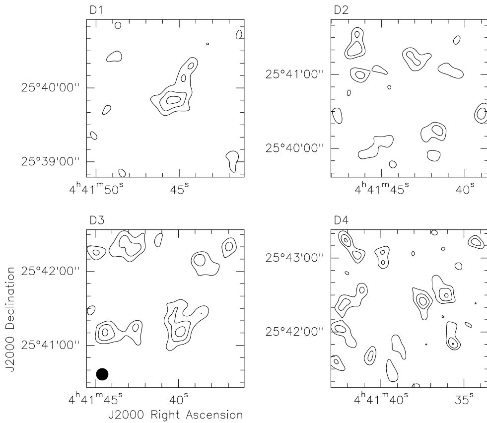
Figure 3.11: Integrated intensity maps of the CCS J_N = 2_1 - 1_0 transition in the fields of core D of TMC-1. Contours are 3, 5 and 7 times the r.m.s. of each map ( 2.1 , 2.6 , 2.0 and 2.0 \text{mJy beam}^{-1} \text{ km s}^{-1} for D1, D2, D3 and D4 respectively). The velocity of integration is 5.5 - 6.3 \text{km s}^{-1} for D1 and 5.5 - 6.2 \text{km s}^{-1} for D2, D3 and D4. The beam size is 10'' , shown at the bottom left corner of D3 map.
