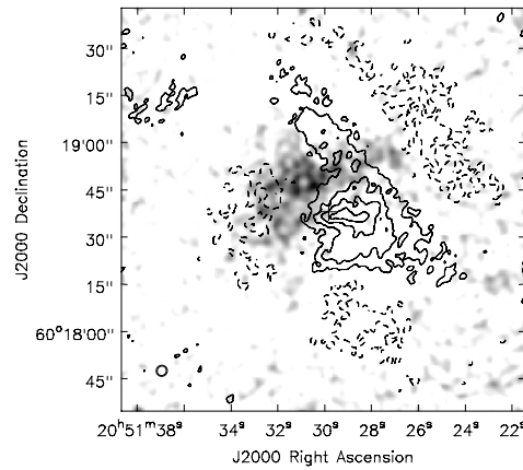
Figure 4.18: Overlay of the integrated velocity map for the CCS ( J_N = 2_1 - 1_0 ) transition (greyscale) and the \text{NH}_3 (1,1) transition (contours) in the GF9-2 region. \text{NH}_3 (1,1) contours are -3, 3, 6, and 9 times 12 \text{ mJy beam}^{-1} \text{ km s}^{-1} .
