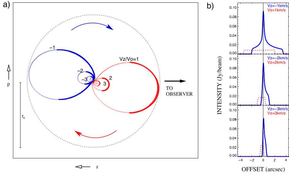
Figure 4.21: (a) Contours of equal l.o.s. velocity for a collapsing and rotating protostellar envelope in a plane close to the equator. (b) Intensity as a function of angular offset from the source center, in equatorial direction, for channel maps of different l.o.s. velocity. Taken from Mayén-Gijón et al. (2014).
