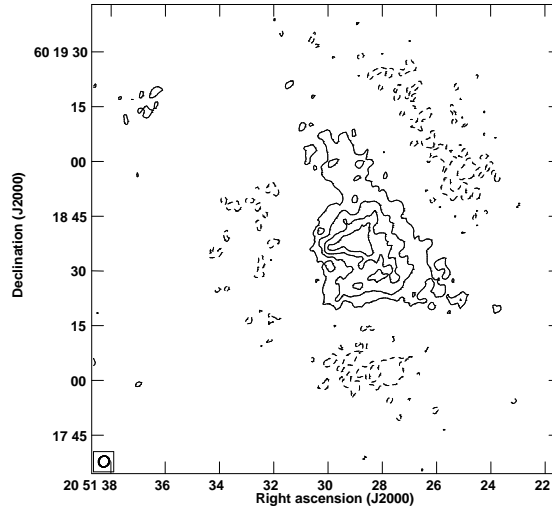
Figure 4.7: Integrated intensity map of the inner satellite components of the \text{NH}_3 (1,1) transition. \text{NH}_3 contours are -3, 3, 6, 9, and 12 times 8 \text{ mJy beam}^{-1} \text{ km s}^{-1} (the r.m.s. of our map).
