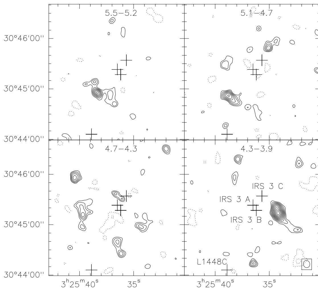
Figure 6.7: Integrated intensity of CCS emission in the IRS 3 region over different velocity ranges (shown at the top of each panel in \text{km s}^{-1} ). Contours are -6, -3, 3, 4, 5, 6, 7, 8, 9, 10, 11, 12 y 13 times 2.7 \text{ mJy beam}^{-1} (the r.m.s. of our map). The ellipse in the bottom right panel is the full width at half maximum of the synthesized beam. Crosses mark the position of sources IRS 3A, 3B and L1448C.
