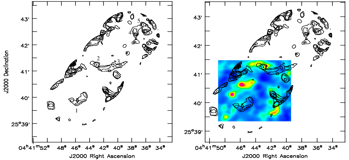
Figure 3.12: . Mosaic of CCS fields of core D (left) and overlay of the mosaic with the NH 3 field of core D (right). First contour and contour level are 10% of the peak.
