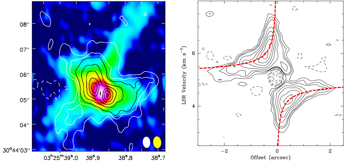
Figure 7.2: Left: Contour map of the integrated intensity of C 18 O(2-1) line emission, superimposed on a color map of the continuum emission (Fig. 7.1). Contour levels are -3, 3, 6 (white) and 9 to 54 at steps of 9 (black) times 2.5 mJy beam -1 km s -1 (the rms of the map). The white and yellow ellipses at the bottom right corner represent the synthesized beams of the continuum and line emission images, respectively (the beam size of the C 18 O(2-1) line map is 0.46'' × 0.30'', P.A. = 4.4°). Right: Position velocity diagram of C 18 O(2-1) emission, along the major axis of the projected disk (position angle = 60°). Contour levels are (in units of mJy beam -1 ): -6 to -18 with increment step -6, -36 to -72 with increment step -18, 6 to 18 with increment step 6, and 36 to 108 with increment step 18. The rms of the map is 2 mJy beam -1 .
