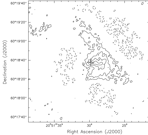
Figure 4.5: Integrated intensity map of the main line of the \text{NH}_3 (1,1) transition in the GF9-2 region. Contours are -3, 3, 6, 9, and 12 times 12 \text{ mJy beam}^{-1} \text{ km s}^{-1} (the r.m.s. of our map). The cross marks the position of GF9-2 mm.
