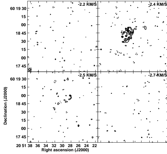
Figure 4.17: Velocity channels for the CCS ( J_N = 2_1 - 1_0 ) in GF9-2 region. The beam is shown at the bottom left corner of the first panel. Contours are -3, 3, 4, 5 and 6 times 2.9 \text{ mJy beam}^{-1} (the r.m.s. of our map).
