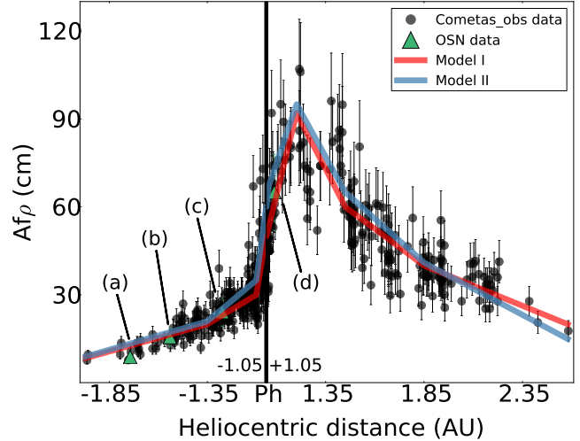
Fig. 8. Comparison between observational data and the models proposed for the comet 103P/Hartley 2. Af\rho measurements have been corrected using Eq. (1). Black dots are the data from Cometas-Obs , and green triangles marked from (a) to (d) are the observations at OSN telescope. The red line corresponds to Model I or Hyperactive model , which fits the observations in Fig. 9. The blue line is the Model II or Standard model , and its fits with observations can be checked in Fig. 10. All the Af\rho values are referred to \rho = 10^4 km.
