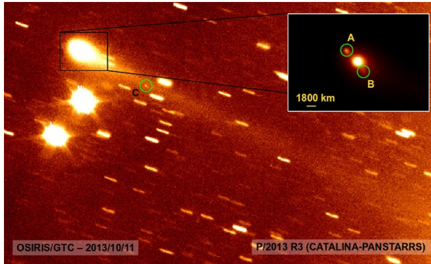
Figure 5.1: The MBC P/2013 R3 (Catalina-Panstarrs) obtained at GTC telescope on October 11th, 2013. The green circles mark the three fragments detected: A, B and C.
