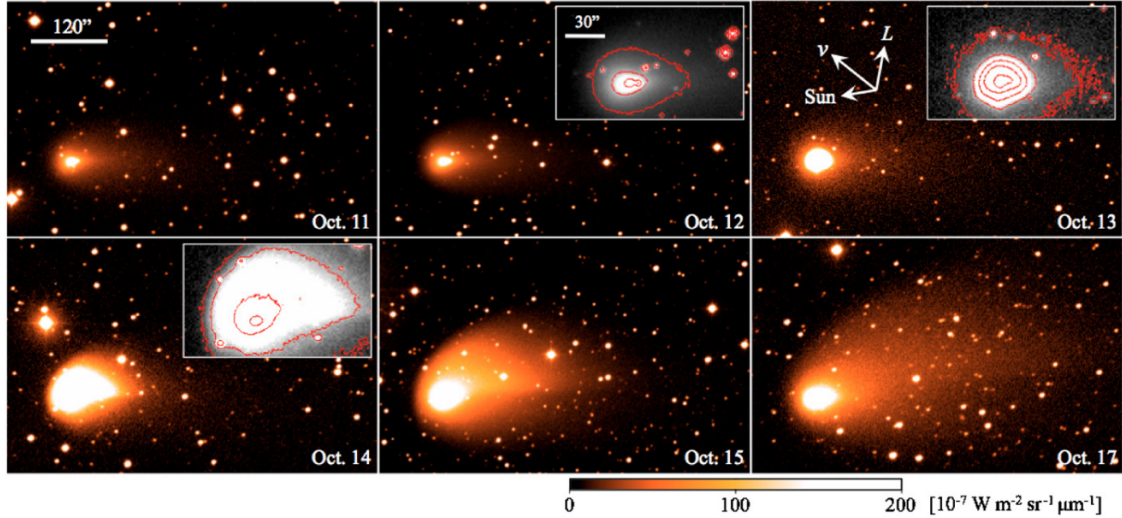
Figure 1.7: Outburst of the comet 217P/Linear, extracted from Sarugaku et al. (2010) . The images were taken with the Kiso 105 cm Schmidt Telescope (Japan), from 11 to 17 October 2010. The images revealed a significant day-to-day expansion of the dust tail, indicating the occurrence of an outburst event.
