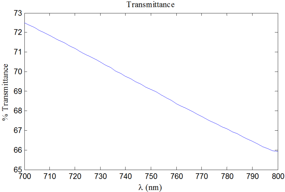
Figure 2.14: GRASSP window transmittance curve
