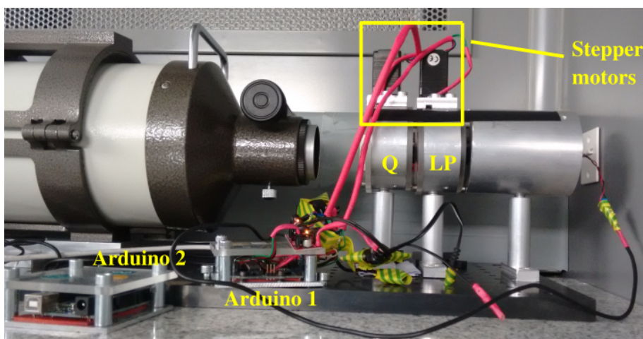
Figure 4.18: Calibration unit formed by a linear polarizer LP (right) and a quarter-wave plate Q (left). Source light goes through the linear polarizer first. LP and Q are embedded within a rotating frame moved by stepper motors controlled by Arduino boards and software.
