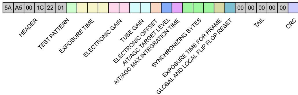
Figure 5.4: Structure of a L'Heritier camera frame
