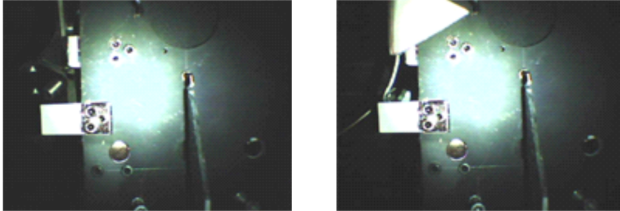
Figure 5.13: Rear part of the spectrograph installed on the telescope mount. Left image shows park position. Right image shows horizontal position. These images were recorded by a webcam which allows the final user to track the telescope mount movements
