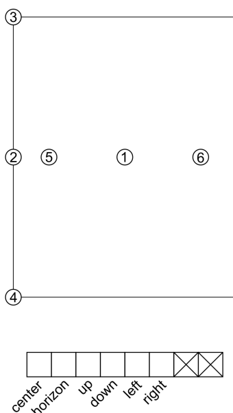
Figure 5.11: Limit switches numbered from 1 to 6 and limit switches status register
