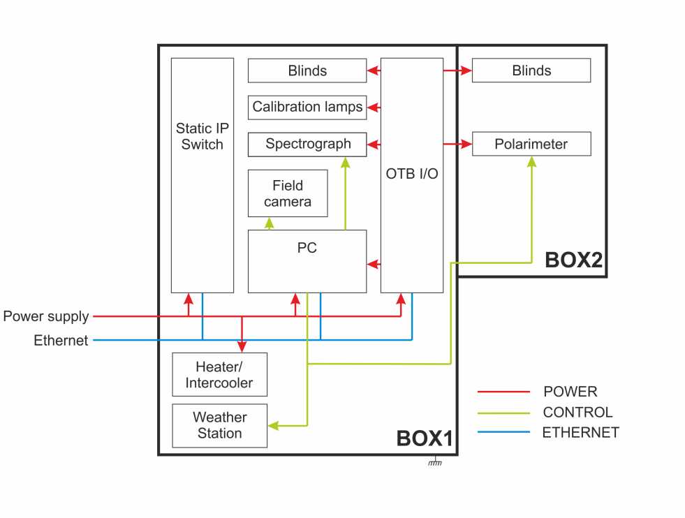
Figure 2.21: Schematic of GRASSP v2.x hardware
