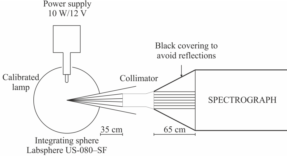
Figure 3.17: Flux calibration setup of GRASSP spectrographs
