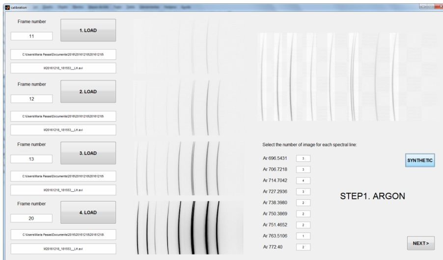
Figure 5.27: calibration.m GUI. Synthetic argon spectrum with all spectral lines with similar intensity (right). The synthetic spectrum can be built only when the four spectral images are loaded
