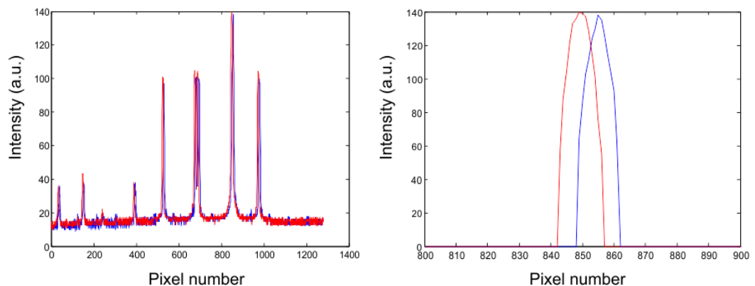
Figure 5.47: Drift calculation. Blue spectrum was recorded at the beginning of the night. Red spectrum was recorded at the end of the night. Right figure is a zoom of the left figure
