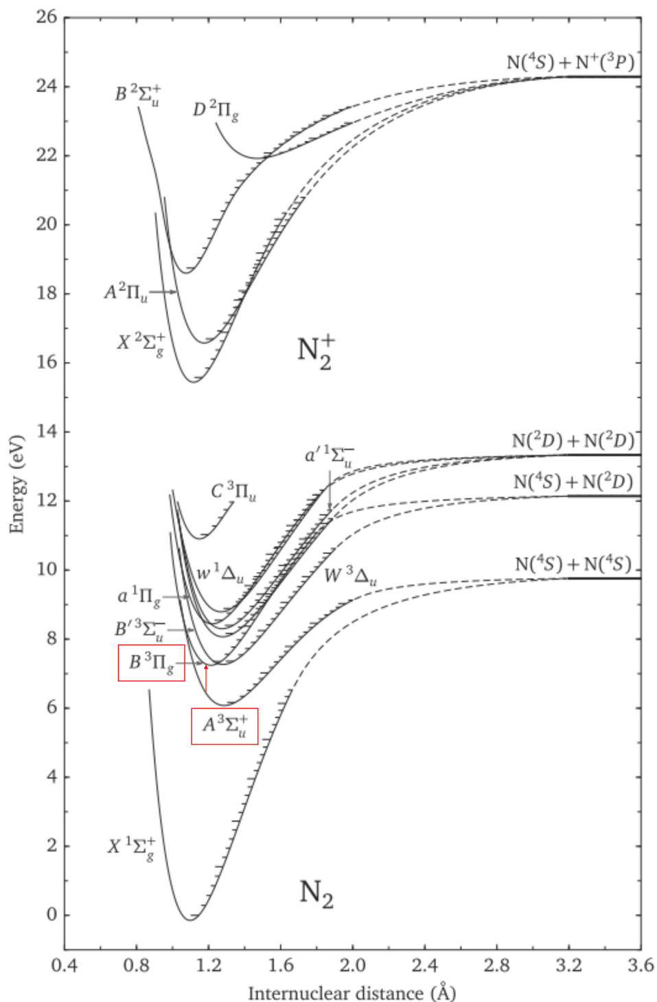
Figure 3.1: Simplified potential-energy diagram of the N_2 molecule and N_2^+ ion. Each curve represents the sum of the electrostatic potential energy of the nuclei and the electronic energies as a function of the internuclear distance, and defines the potential energy for vibrational motion of the nuclei. The vibrational energy levels are shown as tick marks within the respective curves ( Kanmae, 2014 )
