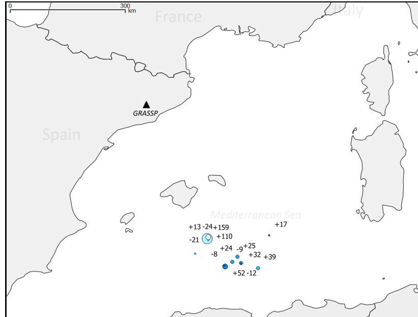
Figure 6.30: Location of the parent lightning of detected sprites on the 16th of November, 2016 over southeastern Balearic islands with the parent strokes as received by METEORAGE are shown (circles and numbers indicate the parent lightning position and corresponding peak intensities, respectively). The location of GRASSP in Castelgallí is indicated with a black triangle
