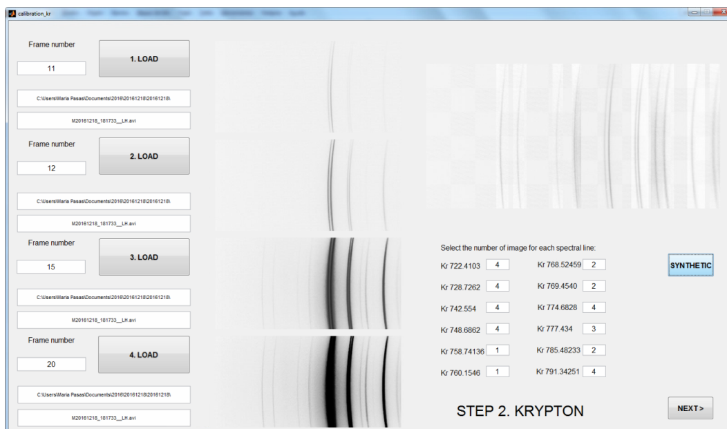
Figure 5.28: calibration.m GUI. Synthetic krypton spectrum with all spectral lines with similar intensity (right)
