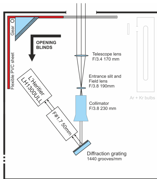
Figure 2.24: Schematic of the GRASSP 2.0 spectrum acquisition system
