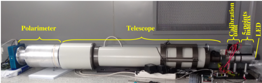
Figure 4.16: The whole chain of optical elements in the optical path of light for calibration. Light goes from right to left. In order: led source, five points matrix, calibration unit, convergent lens of a diffractive telescope, polarimeter.
