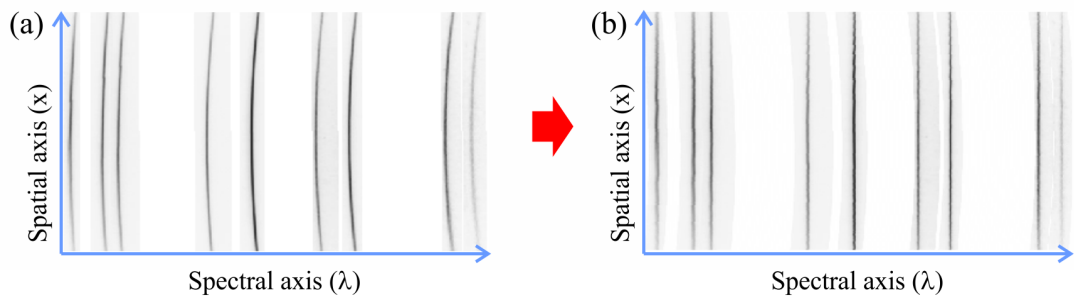
Figure 3.16: Curvature correction for the Ne spectral pattern
