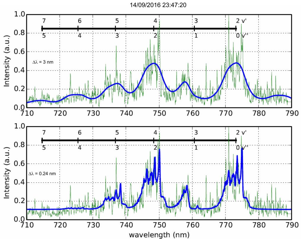
Figure 6.24: Spectral fitting (blue line) between 710 nm and 790 nm of the halo spectrum (green line) recorded at 23:47:20 UTC on the 14th of September, 2016. The top and bottom panels show the recorded spectra fitted with, respectively, 3 nm and 0.24 nm spectral resolutions. The different rovibronic bands ( v' , v'' ) of the N_2(B^3\Pi_g \rightarrow A^3\Sigma_u^+) system are marked. All plots use T_{rot} = 129 K extracted from previous rotational fitting of the (2, 0) band (see figure 6.23)
