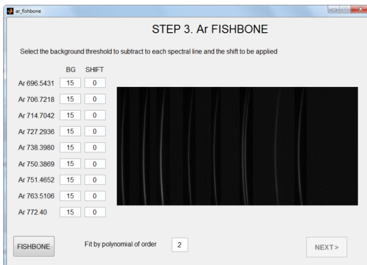
Figure 5.29: calibration.m GUI. Synthetic argon spectrum and editable threshold and shift levels
