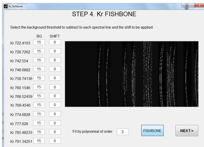
Figure 5.36: calibration.m GUI. Cloud of pixels over the krypton synthetic spectrum maxima. Background threshold should be increased
