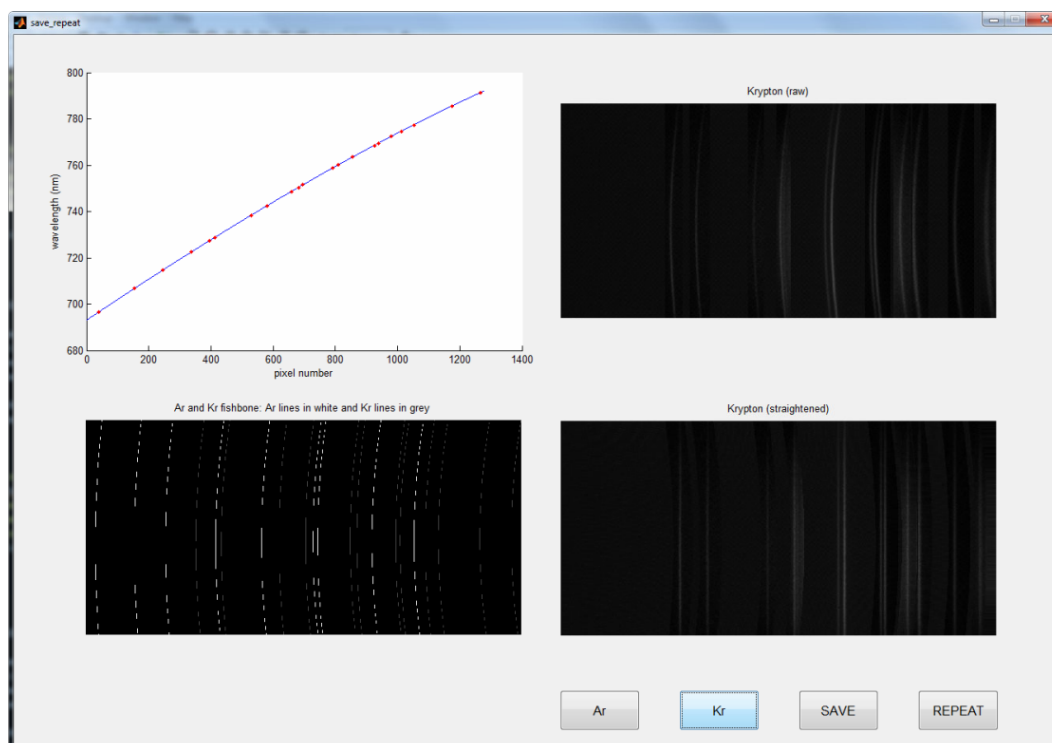
Figure 5.39: calibration.m GUI. From left to right and from up to down: (1) pixel number – wavelength fitting for row number 100 (2) krypton synthetic spectral image (raw) (3) argon and krypton fishbone from the synthetic spectral images (4) krypton synthetic spectral image (straightened)
