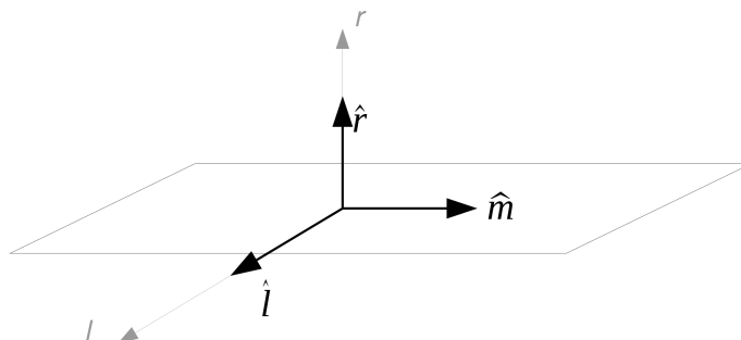
Figure 4.1: Unit vector \hat{m} defines the direction of propagation of light. Vectors \hat{r} and \hat{l} are perpendicular and parallel to the optical plane, respectively. \hat{n} = \hat{r} \times \hat{l}
