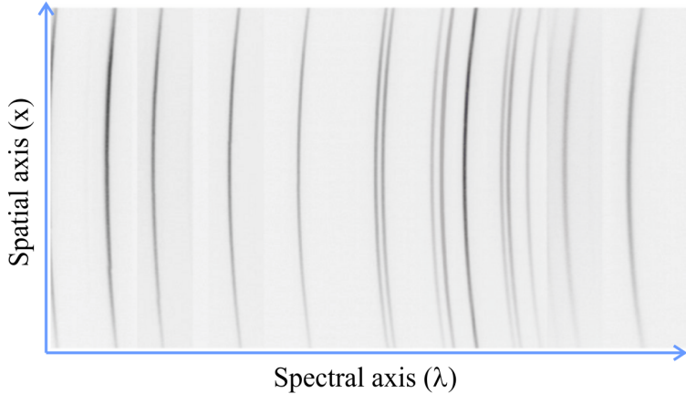
Figure 3.32: Synthetic spectrum of Ar and Kr
