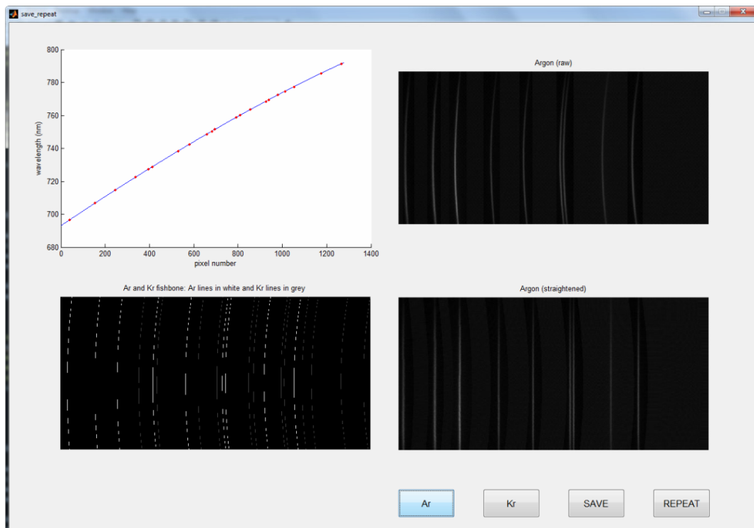
Figure 5.38: calibration.m GUI. From left to right and from up to down: (1) pixel number – wavelength fitting for row number 100 (2) argon synthetic spectral image (raw) (3) argon and krypton fishbone from the synthetic spectral images (4) argon synthetic spectral image (straightened)
