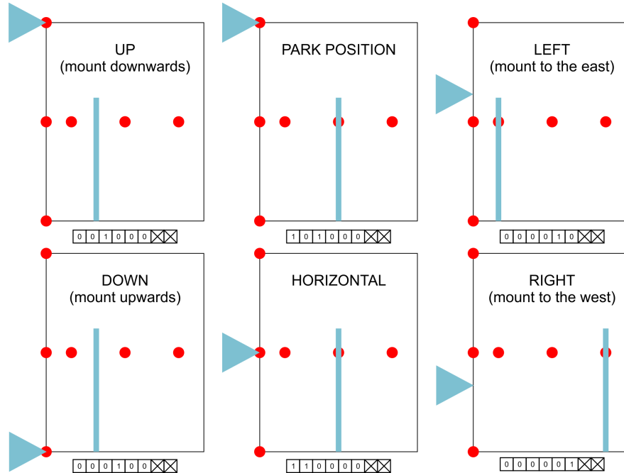
Figure 5.12: Limit switches (red circles) and mount positions (blue graphics). Blue triangle is the aluminum plate installed on the elevation plane of the telescope mount. Blue rectangle is the aluminum plate installed on the azimuth plane of the telescope mount
