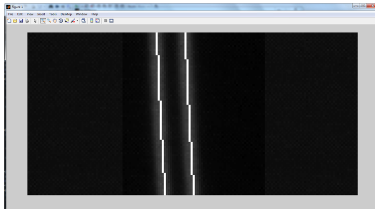
Figure 5.35: Zoom of the fitting of the cloud pixels of the argon synthetic spectrum peaks. We set a shift of one pixel in calibration.m GUI and the fitting curve overlaps the synthetic spectrum
