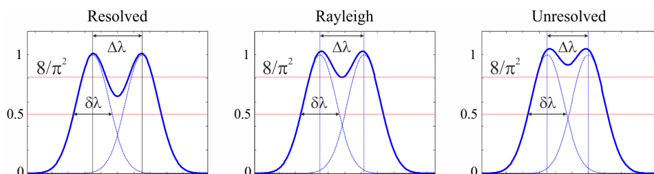
Figure 3.21: Rayleigh criterion to discern among spectral lines
