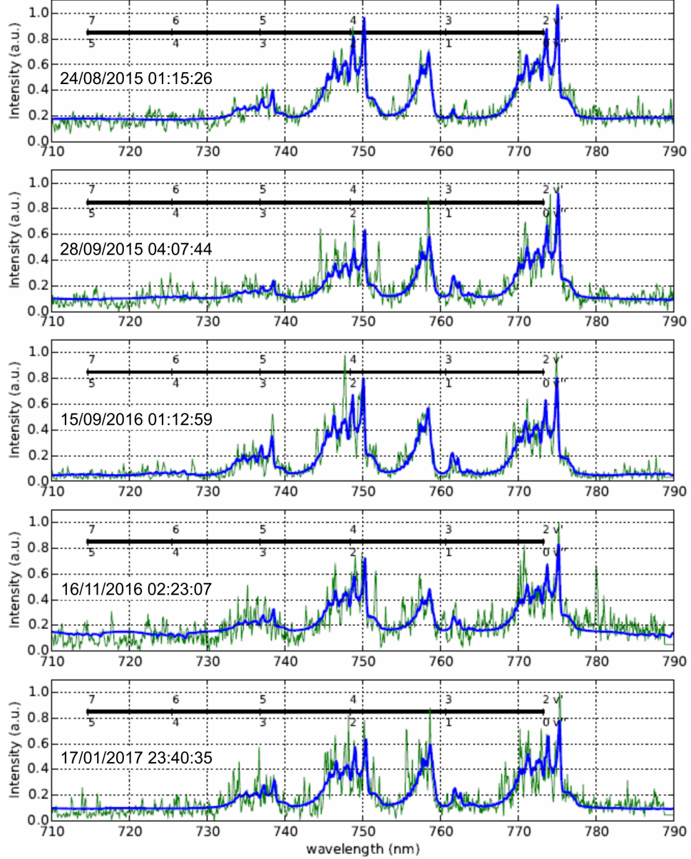
Figure 6.41: Spectral fitting (blue line) between 710 nm and 790 nm of the recorded (green line) spectra which images are shown in, respectively, 1st row-left (carrot sprite, T_{rot} = 185 \text{ K} \pm 10 \text{ K} ), 2nd row left (multi-column sprite, T_{rot} = 149 \text{ K} \pm 10 \text{ K} ), 3rd row left (carrot sprite, T_{rot} = 178 \text{ K} \pm 10 \text{ K} ), 3rd row right (multi-column sprite, T_{rot} = 164 \text{ K} \pm 18 \text{ K} ) and 4th row right (multi-column sprite, T_{rot} = 201 \text{ K} \pm 20 \text{ K} ) of figure 6.38. The synthetic (fitted) spectra are generated using a spectral resolution of 0.24 nm. The different rovibronic bands ( v', v'' ) of the \text{N}_2(\text{B}^3\Pi_g \rightarrow \text{A}^3\Sigma_u^+) system are marked. The used T_{rot} are extracted from previous rotational fitting of the (2, 0) band (see figure 6.39). The original recorded spectra is normalized to the (2, 0) band head peak (774.8 nm - 775.4 nm)
