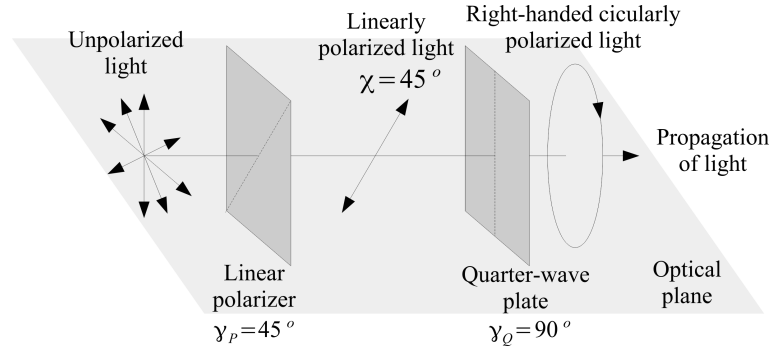
Figure 4.5: A circular polarizer consists of a linear polarizer plus a quarter-wave plate. In the first place, light is linearly polarized at 45^\circ or -45^\circ . Then, it is converted into right- or left-handed, respectively, when passing through the quarter-wave plate.
