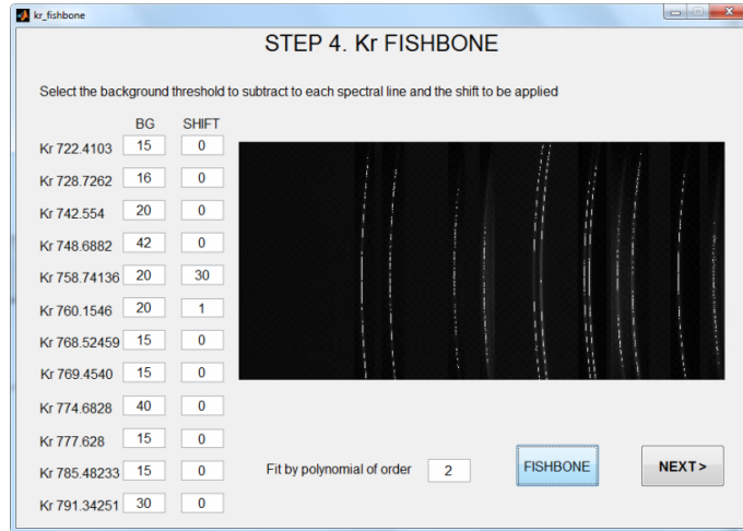
Figure 5.37: calibration.m GUI. Cloud of pixels over the krypton synthetic spectrum maxima. We have set shifts and background thresholds to fit the spectral pattern
