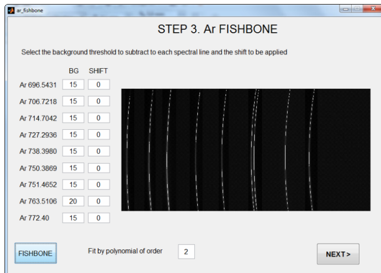
Figure 5.31: calibration.m GUI. Cloud of pixels over the synthetic spectrum maxima. The background threshold level is set to 20 for the spectral line 763.5106 nm of argon. No dispersion is detected and fitting is possible now
