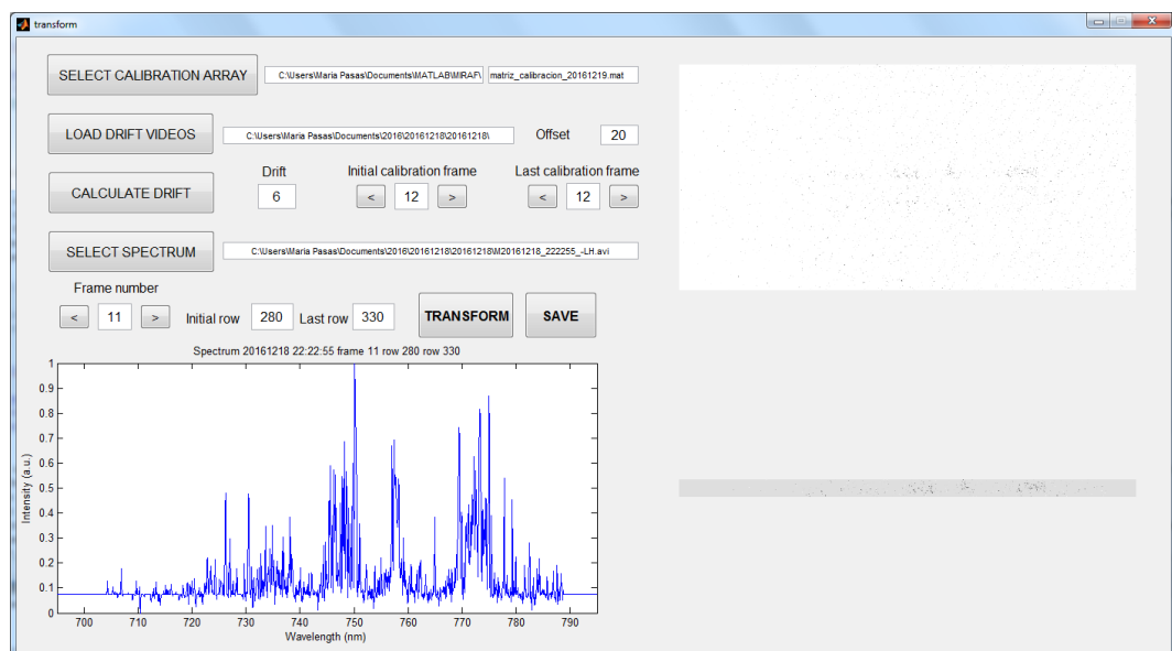
Figure 5.49: transform.m GUI. Left-bottom figure shows the trimmed and corrected spectrum of the video frame number 11 for rows between 280 and 330. Right-bottom figure shows the trimmed and corrected spectrum image
