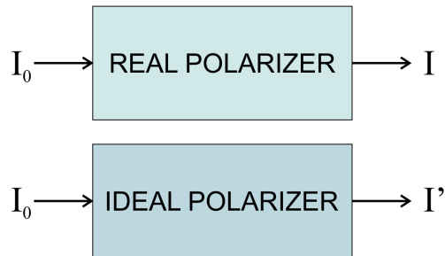
Figure 4.13: Stokes vectors of light coming from the source before it goes through any of the polarizers of the polarimeter ( I_0 ), and after ( I if the polarizer is real and I' if the polarizer is ideal)
