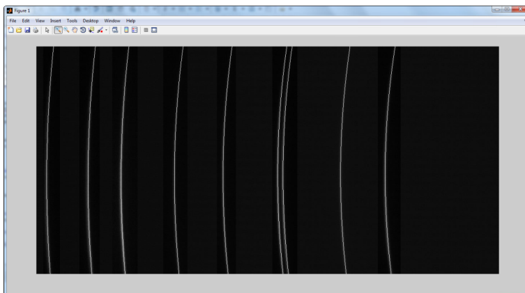
Figure 5.32: Fitting of the cloud pixels of the argon synthetic spectrum peaks
