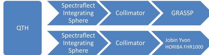
Figure 3.36: Different ways to obtain the spectral response of the QTH spectral lamp
