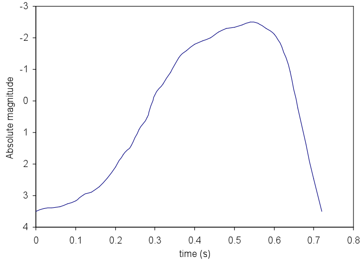
Figure 6.12: Lightcurve (absolute magnitude vs. time) of the Orionid meteor analyzed in the text
