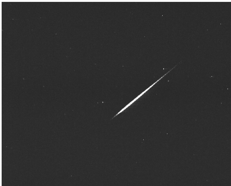
Figure 6.8: Sum pixel intensity image of the Orionid meteor imaged from CAHA
