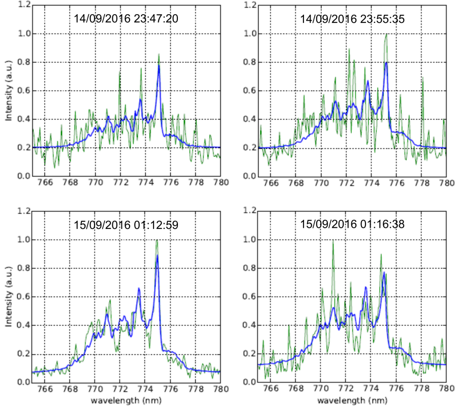
Figure 6.23: Spectral fitting (blue line) of recorded spectra (green line) of sprites and sprite halos on 14-15 September, 2016. The spectra correspond to the (2, 0) rovibronic transition of the N_2(B^3\Pi_g \rightarrow A^3\Sigma_u^+) system using spectral resolutions of 0.24 nm (for sprites) and 0.18 nm (for halo - top left).
