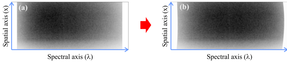
Figure 3.18: Curvature and wavelength correction of a QTH lamp spectrum. (a) QTH lamp curved spectrum from SPEC1. Notice that this image does not seem to be curved because the spectral pattern is flat and covers the whole iCCD (b) QTH lamp curved-corrected spectrum. When curvature-correcting a flat spectral image that covers the whole iCCD, the corrected spectral pattern is curved
