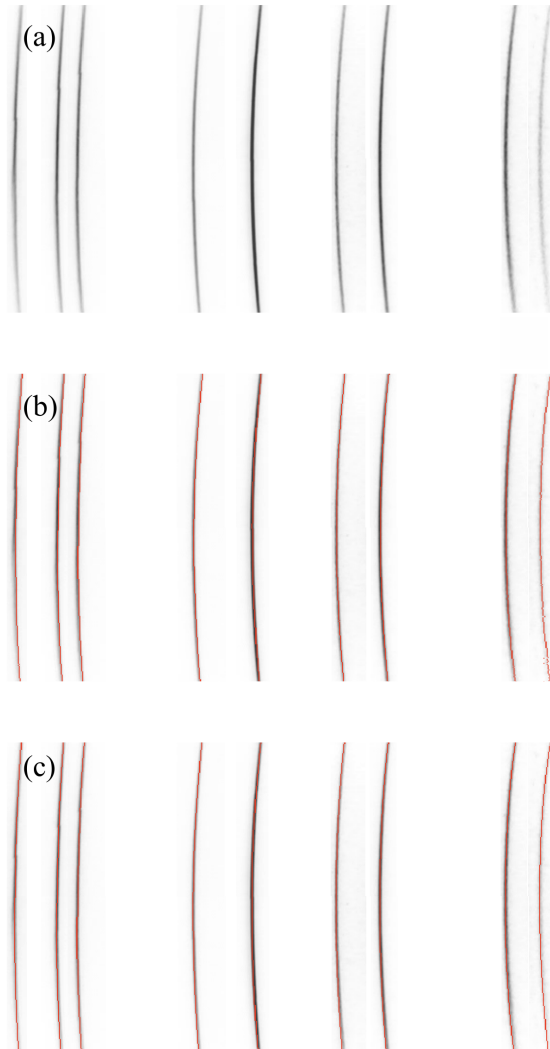
Figure 3.14: a) Synthetic spectrum of Ne. b) Cloud of pixels over the maximum intensity in spectral lines of Ne. c) Fitting curves overlapping Ne spectrum
