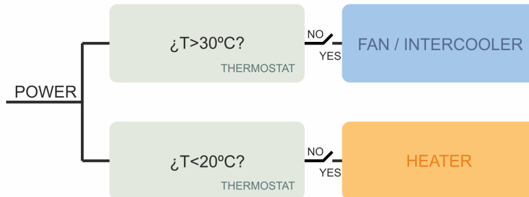
Figure 2.9: Block diagram of GRASSP thermal system
