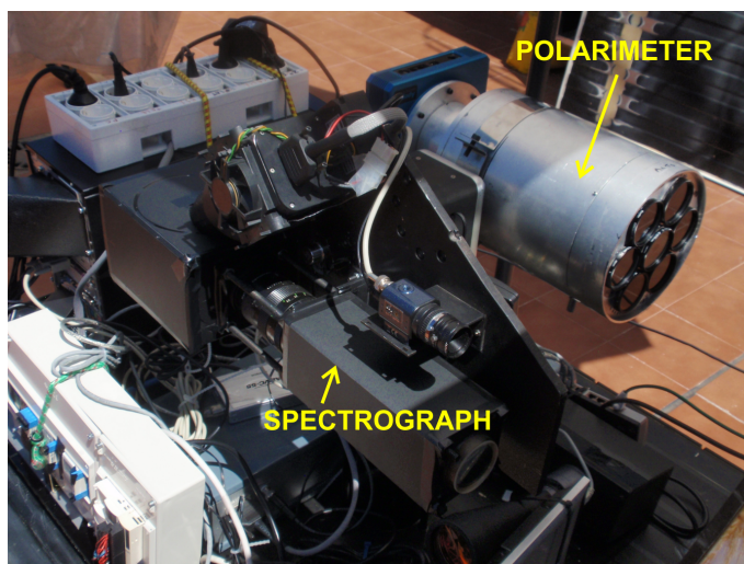
Figure 4.9: GRASSP polarimeter and spectrograph installed within GRASSP v1.0
