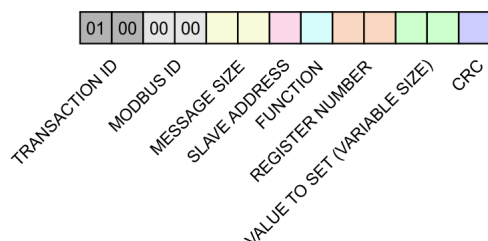
Figure 5.7: Structure of a Modbus frame
