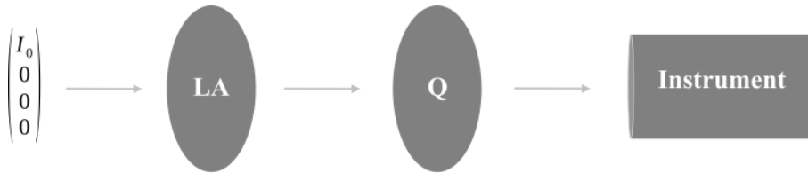
Figure 4.15: A linear polarizer and a quarter-wave plate placed between the light source and the instrument as a calibration unit in complete mode.
