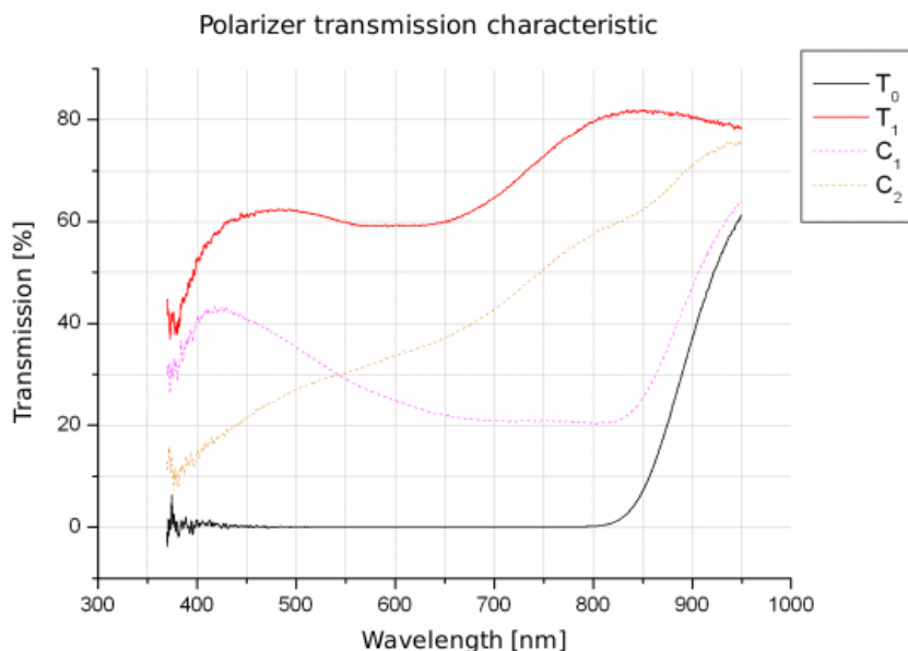
Figure 4.10: Real transmission test for a polarized linear filter illuminated by polarized light
