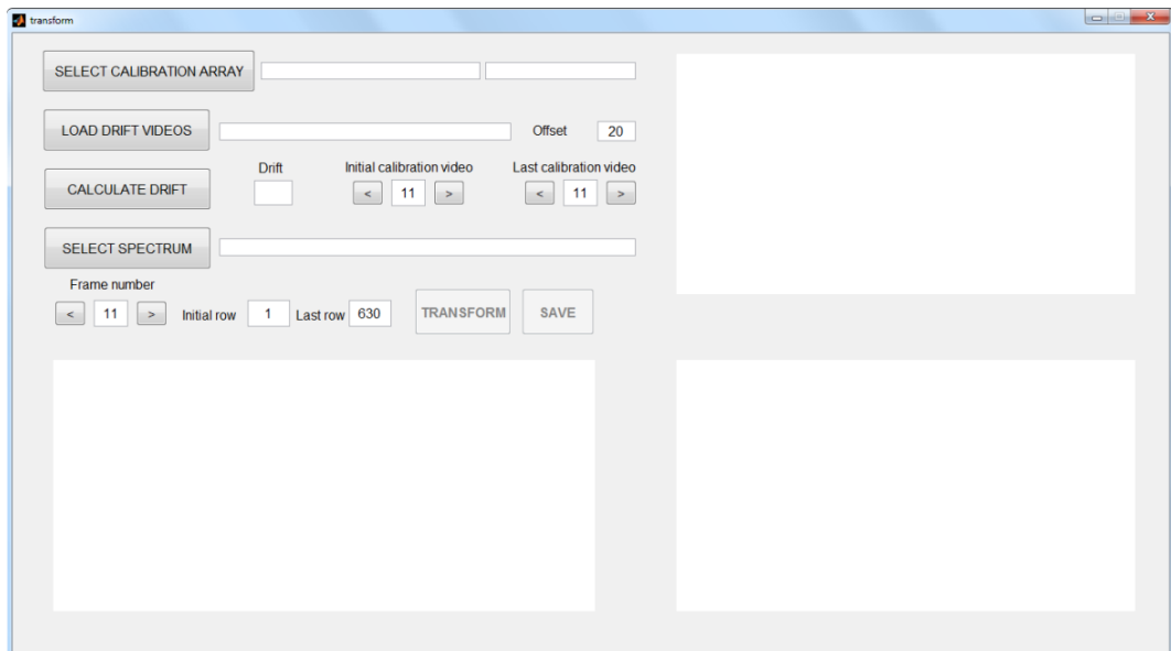
Figure 5.44: transform.m GUI
