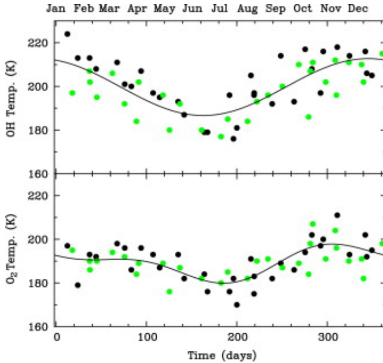
Figure 6.40: SATI monthly rotational temperatures. Black solid circles: from Oct 1998 to March 2002; grey solid circles: from April 2002 to July 2006; solid lines: numerical fitting for the whole set of data ( López-González et al. , 2007)
