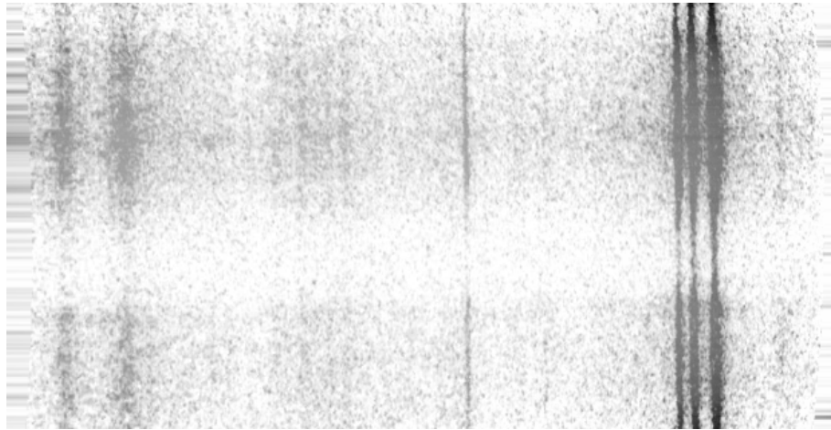
Figure 6.4: iCCD image of the spectrum of light from lightning scattered on clouds, trimmed, flipped, corrected, straightened and corrected by SPEC1 instrument function. It was recorded on the 10th of July 2013 at 03:21:36 UTC
