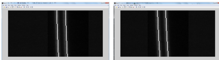
Figure 5.33: Zoom of the fitting of the cloud pixels of the argon synthetic spectrum peaks. Notice that there is a shift in the fitting
