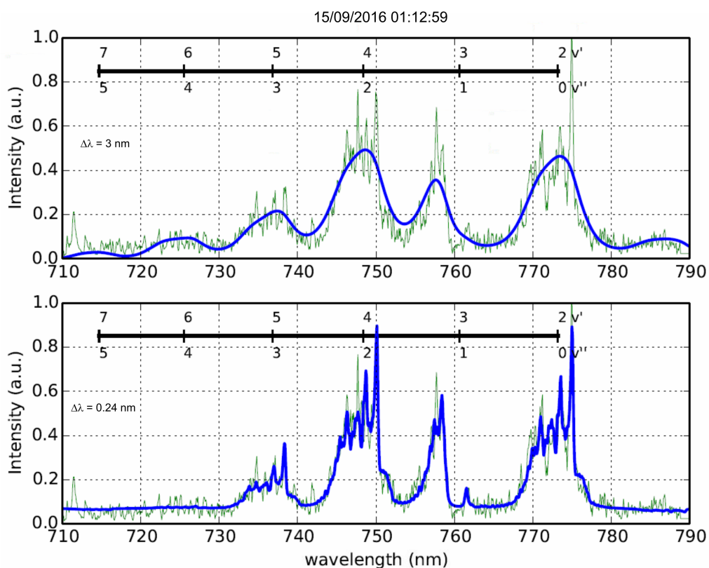
Figure 6.26: Spectral fitting (blue line) between 710 nm and 790 nm of the carrot sprite spectrum (green line) recorded at 01:12:59 UTC on the 15th of September, 2016. The top and bottom panels show the recorded spectra fitted with, respectively, 3 nm and 0.24 nm spectral resolutions. The different rovibronic bands ( v' , v'' ) of the N_2(B^3\Pi_g \rightarrow A^3\Sigma_u^+) system are marked. All plots use T_{rot} = 154 K extracted from previous rotational fitting of the (2, 0) band (see figure 6.23)
