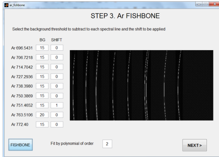
Figure 5.34: calibration.m GUI. Cloud of pixels over the argon synthetic spectrum maxima. We have set a shift of one pixel to the spectral line 751.4652 nm of argon
