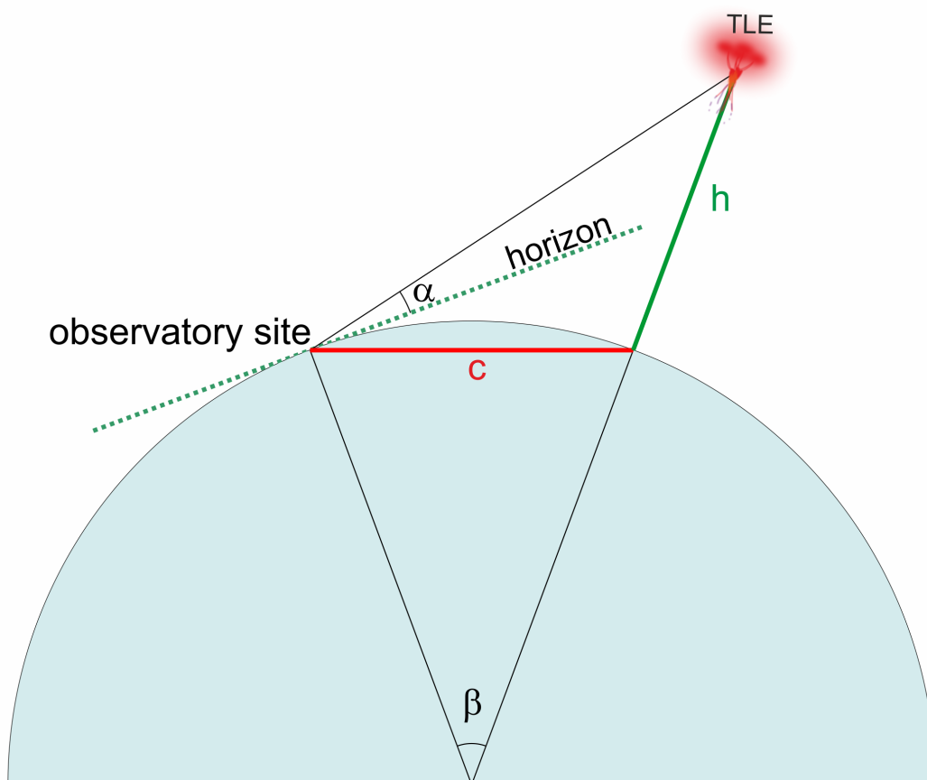
Figure 6.45: Geometry for the calculation of event altitude h based on great circle \beta and observed elevation angle \alpha ( van der Velde and Montanyà, 2016 )
