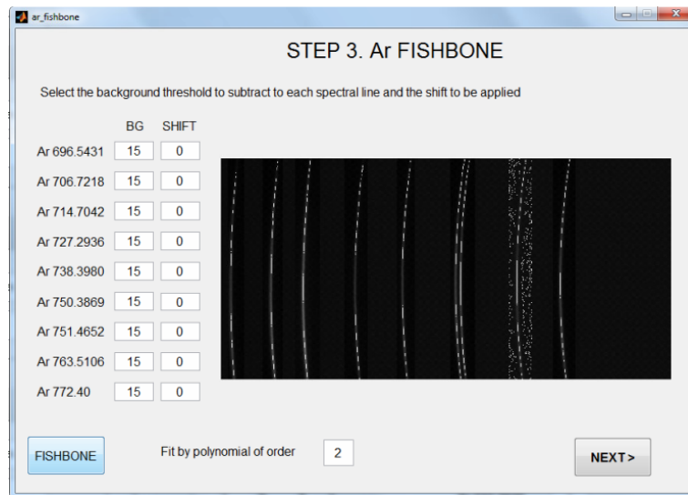
Figure 5.30: calibration.m GUI. Cloud of pixels over the synthetic spectrum maxima. Notice that the spectral line 763.5106 nm of argon shows a very dispersed cloud of pixels around it, resulting impossible to fit. The background threshold is 15
