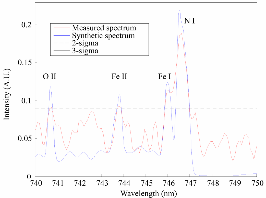
Figure 6.10: Details of a meteor spectrum (red line) from 740 to 750 nm, obtained with GRASSP v1.1 spectrograph on 2014 October 16th at 01:19:40 UT. Flux is dimensionless. The blue line is a composition of a N_2 first positive system synthetic spectrum at T_{rot} = T_{vib} = T = 1500 K, at an altitude between 99 and 108 km, combined with a synthetic spectrum of N I, N II, O I, Ti I, Cr I, Fe I, Fe II, Zr I and W I atomic lines convolved with a gaussian curve of sigma 0.10 nm. Notice that the strongest features of N I at 742.364 and 744.229 nm can not be found, although atomic lines of Fe have been identified
