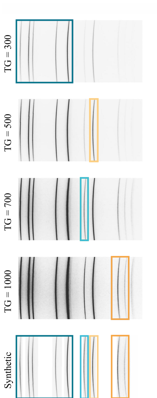
Figure 3.13: Synthetic spectrum of Ne
