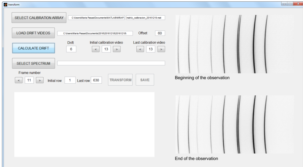
Figure 5.46: transform.m GUI. When pressing the LOAD DRIFT VIDEOS button, a dialog box shows up and the user selects two calibration spectra videos: one at the beginning and one at the end of the observation night. Then the final user selects—with the naked eye—the video frames so all spectral lines show up with similar intensity level in both videos
