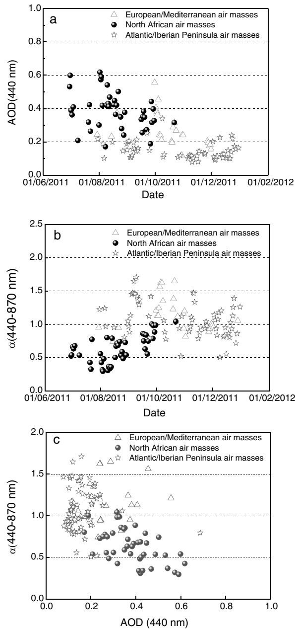
Figure 3. Temporal evolution of daily mean: (a) AOD (440 nm) and (b) \alpha(440\text{--}870\text{ nm}) values over Alborán Island according to the aerosol origin classification. (c) Correlation between AOD (440 nm) and \alpha(440\text{--}870\text{ nm}) for each origin sector.
