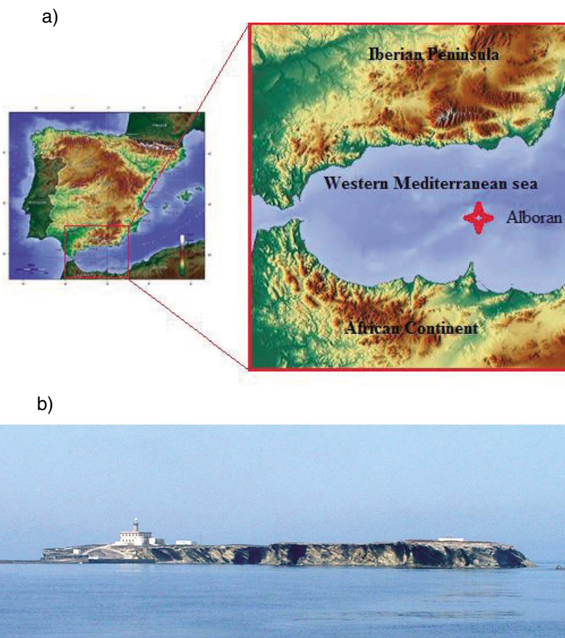
Figure 1. (a) Geographic location and (b) image of Alborán Island.
