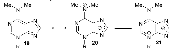
Scheme 7. Resonance hybrid 20 can explain the alkylation at the N -3 atom of the purine moiety, as suggested by non-equivalent -NMe 2 signals in the ^1\text{H} NMR spectrum of ( RS )- 17 .
