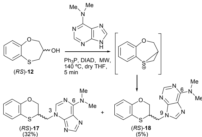
Scheme 4. Preparation of the ( RS )-(3-alkylated- N,N -dimethyl)adenine [( RS )- 17 ] and ( RS )-(9-alkylated- N,N -dimethyl)adenine [( RS )- 18 ].
