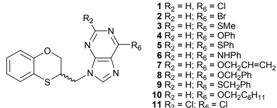
Fig. 1. 2- and 6-substituted ( RS )-9-(2,3-dihydro-1,4-benzoxathiin-3-ylmethyl)-9 H -purine derivatives obtained by the Mitsunobu reaction.
