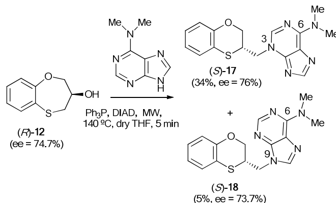
Scheme 6. Reactivity between ( R )- 12 and N,N -dimethyladenine.
