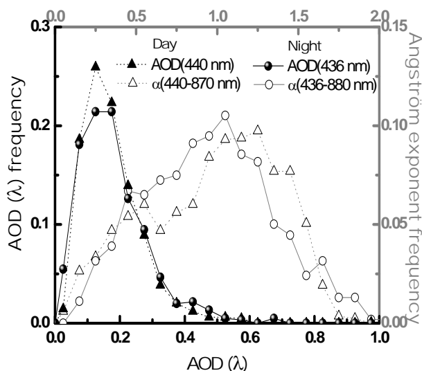
Fig. 3. Frequency histograms of AOD(440 nm) and \alpha(440\text{--}870\text{ nm}) obtained at daytime and of AOD(436 nm) and \alpha(436\text{--}880\text{ nm}) obtained at nighttime for the period 2007–2010.
