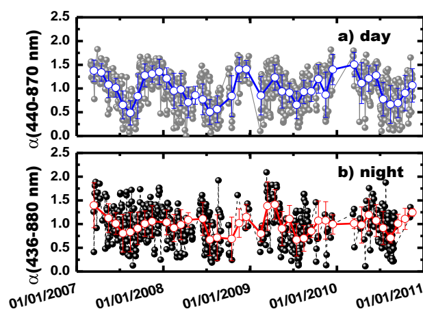
Fig. 2. (a) Temporal evolutions of daytime Angstrom exponent \alpha(440-870 \text{ nm}) and (b) nighttime Angstrom exponent \alpha(436-880 \text{ nm}) . Fully circles linked by dash lines corresponds to day/night mean values, while open circles linked by solid lines represents monthly day/night values and their standard deviations. All the data were acquired at Granada from 2007 to 2010.
