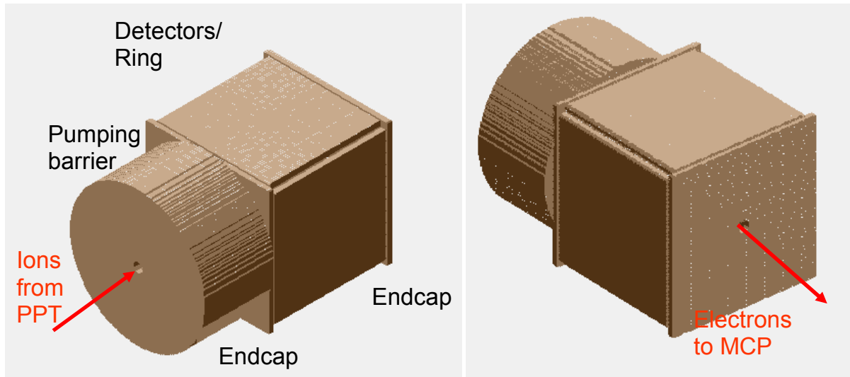
Figure 67: Pictures from SIMION of the detector trap plus associate elements.
