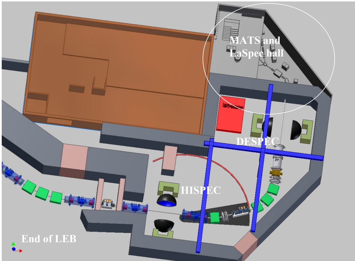
Figure 1: End of the Low Energy Beam line of the Super FRS at the future FAIR facility.
