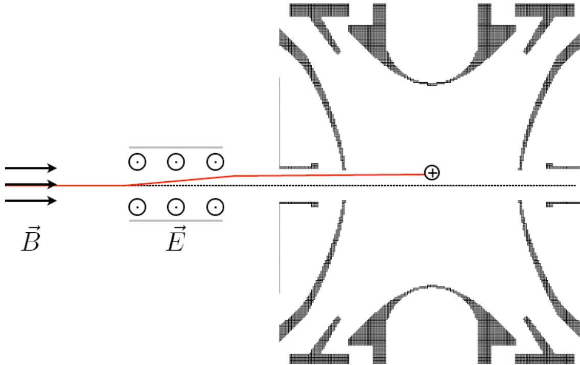
Figure 57: Simulation of ion injection in the hyperbolic Penning trap preceded by the Lorentz steerer.
