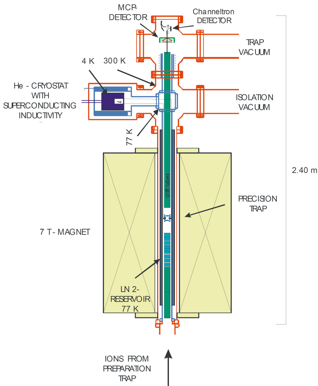
Figure 56: Proposed high-accuracy measurement Penning trap for mass spectrometry at the MATS project. The trap system is installed in a 7 T superconducting magnet. For mass spectrometry either a destructive time-of-flight cyclotron resonance or a non-destructive Fourier transform ion cyclotron resonance detection will be used.
