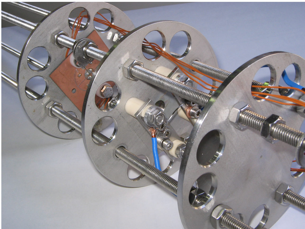
Figure 53: picture of an electron gun plus segmented Faraday cup to align a Penning trap with the magnetic field from a superconducting magnet.
