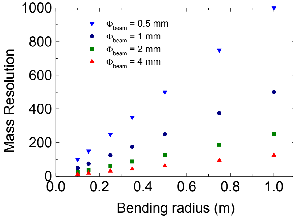
Figure 42: Mass resolution ( M/\Delta M ) versus bending radius for a dipole magnet. The magnetic rigidity B\rho is 9,1 \times 10^2 for ions with mass A=40 and 10 keV kinetic energy. The parameter M_x in Eq. (2) has been chosen equal to 1.
