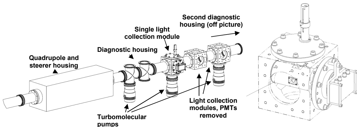
Figure 82: Technical illustration of the ionic spectroscopy beamline showing an expanded view of a light collection module.
