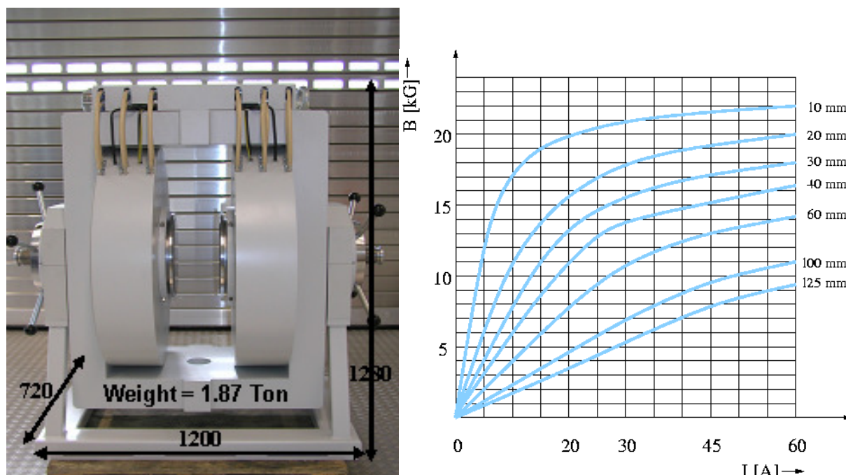
Figure 88: Left: typical \beta -NMR magnet. Right: magnetic field depending on magnet current and pole gap
