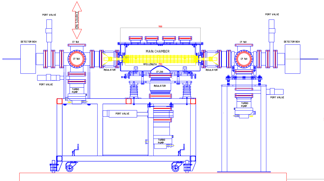
Figure 20: Schematic of the complete vacuum system including the RFQ structure. The dimensions and main components are indicated in the figure. The trolley shown in the drawing might be needed for easy removal of the whole RFQ apparatus. It will be replaced by a fixed support if it is not required.
