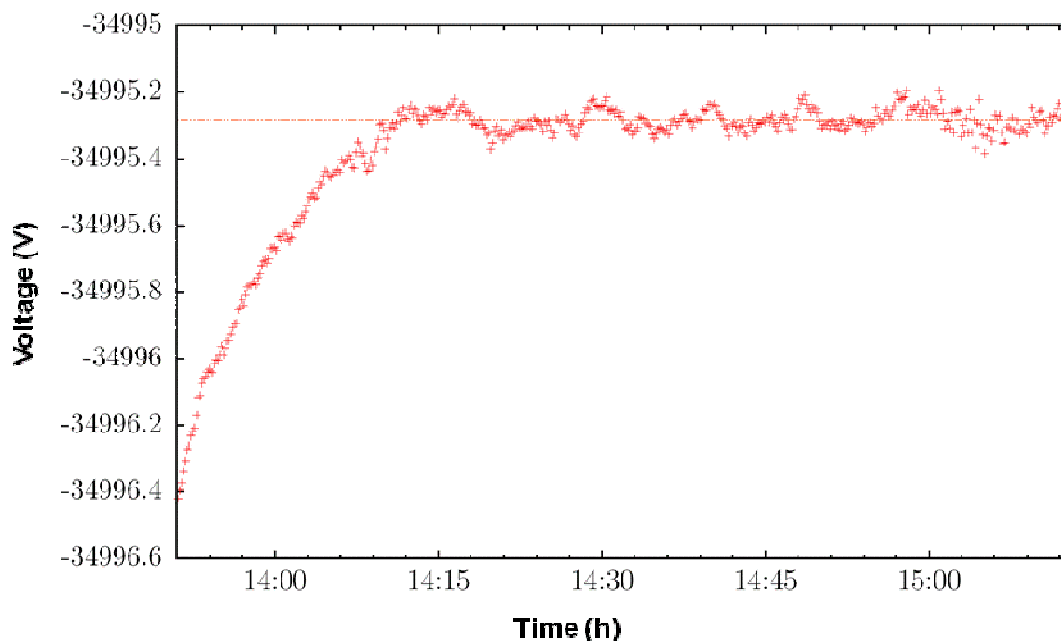
Figure 91: High voltage of the ISOLDE frontend after turning on the HV supply measured with the KATRIN high voltage divider.
