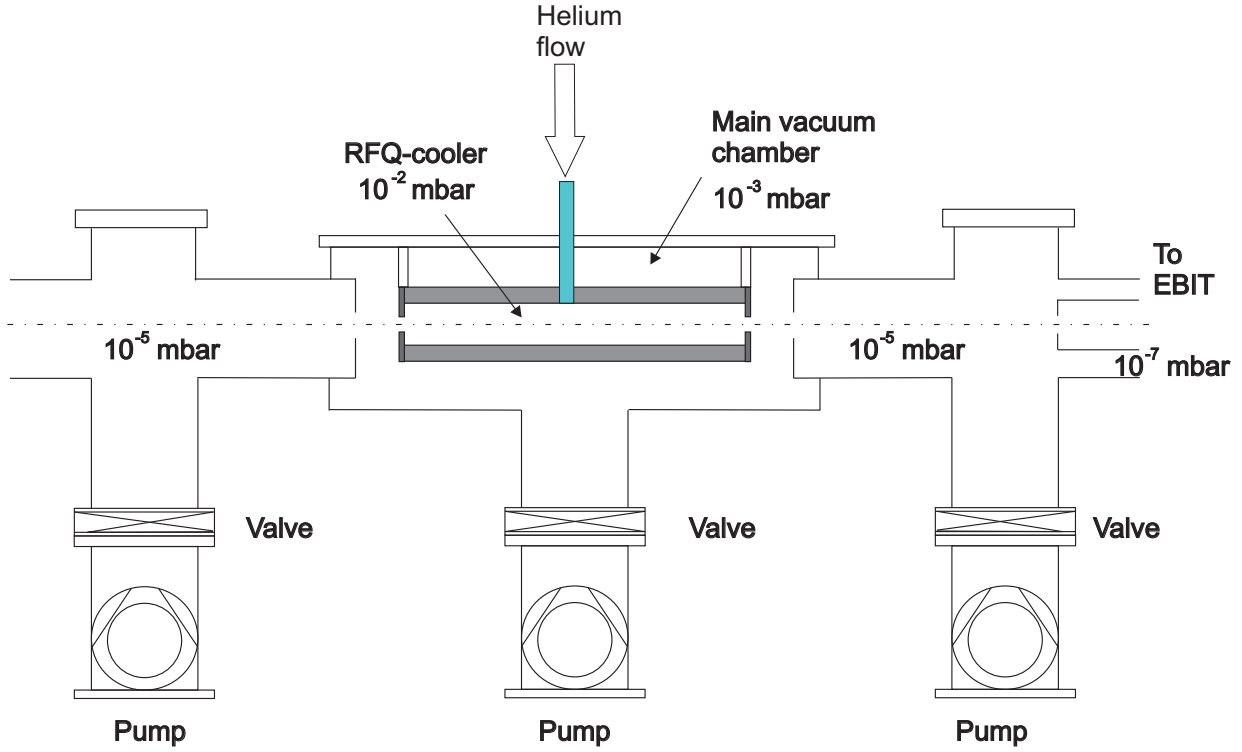
Figure 17: A schematic drawing of the vacuum system for the RFQ system. The beam enters from the left.
