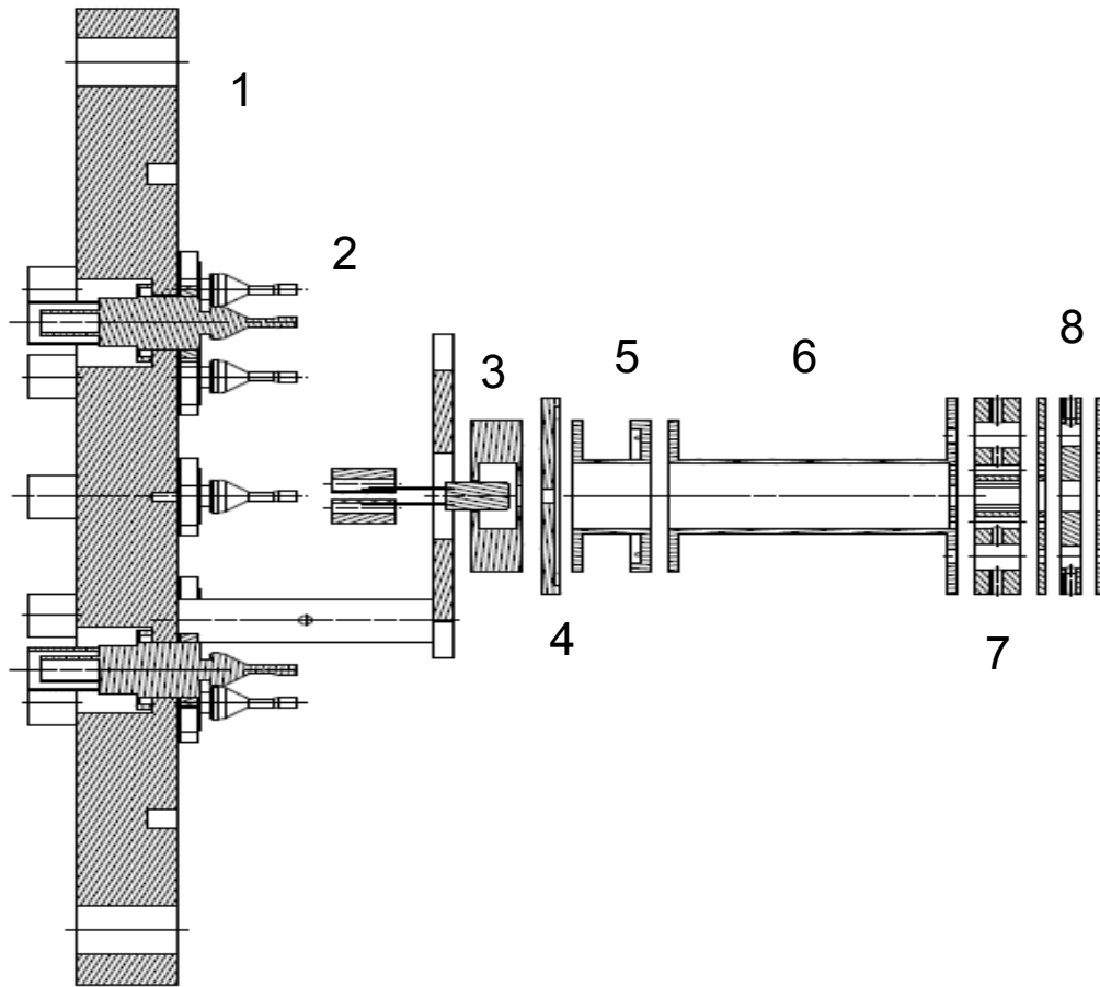
Figure 15: technical drawing of an alkali ion source used for off-line measurements [Flech2009]. The different components are marked by: 1) CF-160 flange; 2) SHV connectors; 3) pellet housing; 4) extraction plate; 5) and 6) lenses, 7) X-Y deflector and 8) diaphragms. The total length of the source is about 15 cm.
