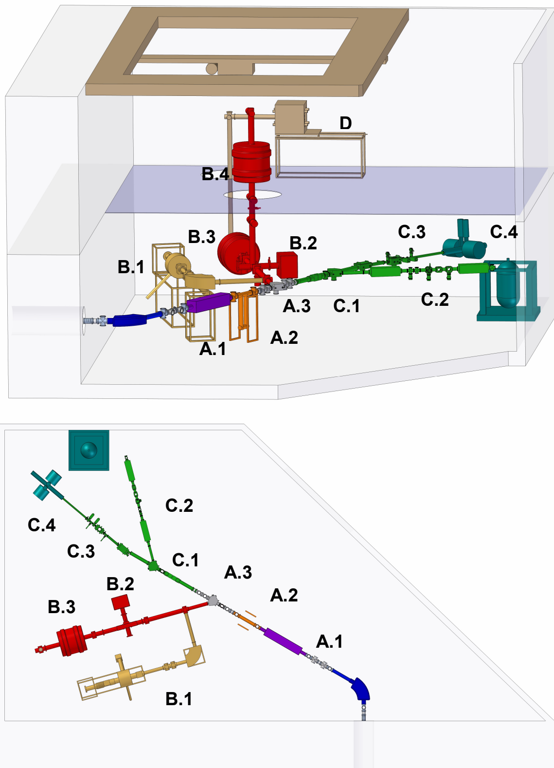
Figure 12: Top: Overview of the MATS and LaSpec experiments at the end of the low-energy beamline of the Super-FRS. Bottom: top view of the setups including the gas-filled stopping chamber. The Buncher section (A.1), the multi-reflection time-of-flight mass spectrometer (A.2), and the switchyard (A.3) are the common components. The MATS beamline is shown schematically in red: (B.1) is the EBIT junction, (B.2) the off-line ion source, (B.3) the Preparation Penning trap section, and (B.4) the Measurement Penning Trap section. The LaSpec beamline is represented by the green components: (C.1) is the common supply line, (C.2) the ion beam line, (C.3) is the atom beam line with beta-NMR (C.4). D is a setup for neutron decay and total absorption spectroscopy.
