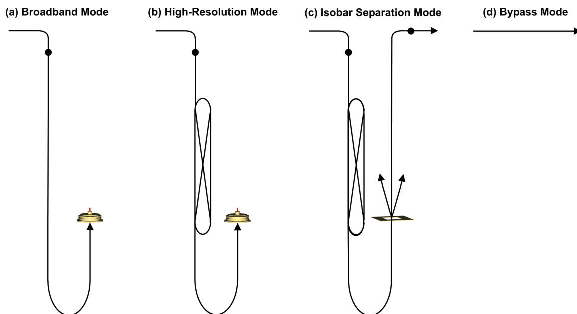
Figure 23: Illustration of the four operation modes of the MR-TOF-MS (compare with Fig. 22): (a) broadband mass spectrometer for ion identification, (b) high-resolution mass spectrometer, (c) isobar separator, and (d) ion guide. The black dots indicate points where ions are trapped, cooled and accumulated. For (a) and (b) a detector is located in the time focus of the device, for (c) the ion gate is moved into the time focus.
