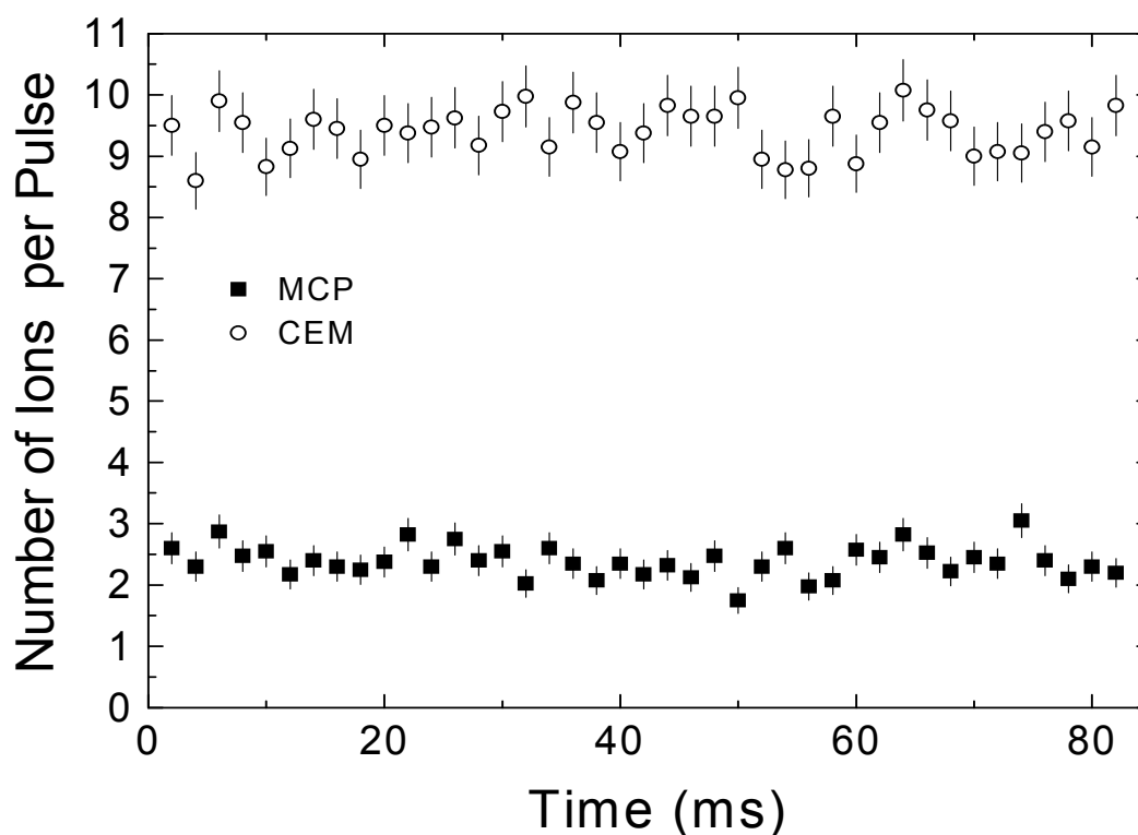
Figure 61: Relative detection efficiency of MCP and CEM detectors using a pulsed singly-charged ion beam. Each measurement represents the mean value of the number of ions detected in 40 pulses.
