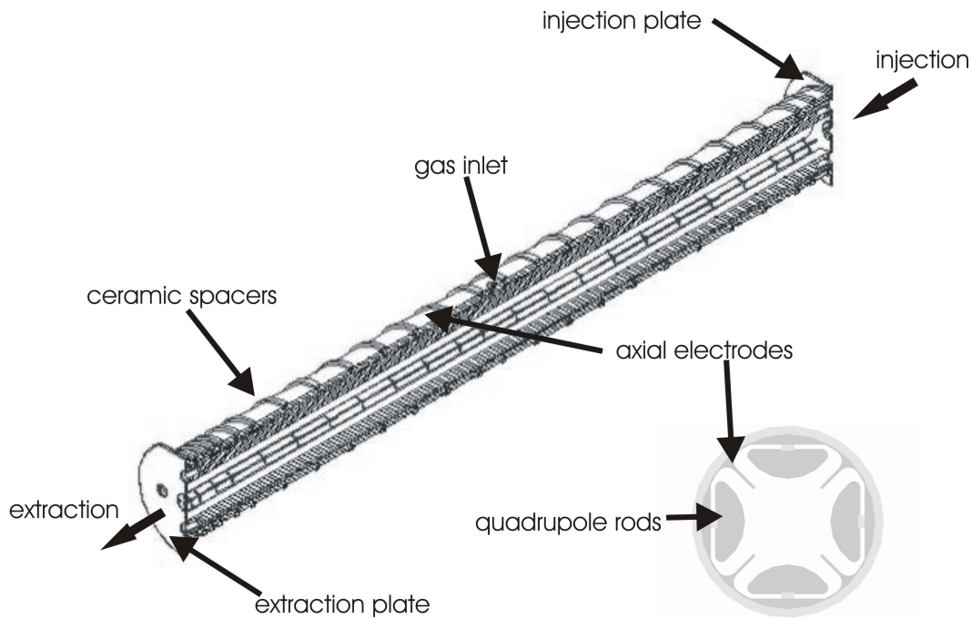
Figure 16: Left: Half cut view of the ISOLDE RFQ structure. Right: Cross section perpendicular to the optical axis.
