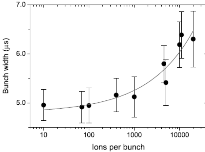
Figure 18: Dependence of the bunch width on the number of ions in the bunch. The bunch widths were determined by measuring the TOF distribution of the ions. The continuous beam intensity was kept at 1-2 \times 10^5 \text{ s}^{-1} . The solid line represents a N^{1/3} dependence, compatible with a linear increase in the ion cloud volume [Niem2001].
