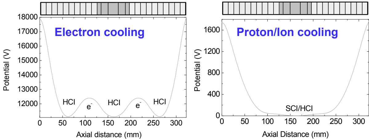
Figure 46: Trapping configuration for electron (left) and ion/proton cooling (right). The maximum and minimum potential for the electron-cooling configuration are taken from Ref. [Maer2008].
