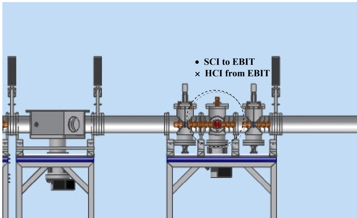
Figure 37: Section of the MATS beamline extracted from Figure 28. The ions are first deflected in the horizontal plane and transferred into an EBIT for charge breeding, or transferred to the PPT or MPT using an electrostatic quadrupole deflector. After charge breeding, the ions, in the proposed scheme are separated using a dipole magnet or a Wien filter.
