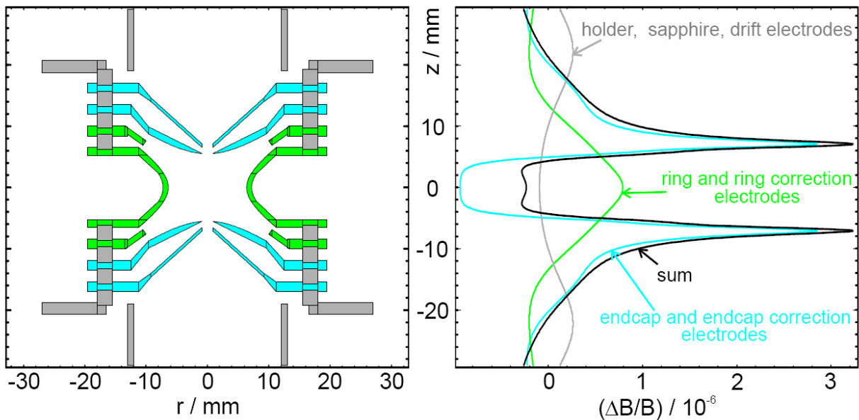
Figure 55: Left: Cut of the precision trap. Right: Magnetic field change due to the magnetization of the trap materials. The contributions of the individual electrodes are shown together with the sum.
