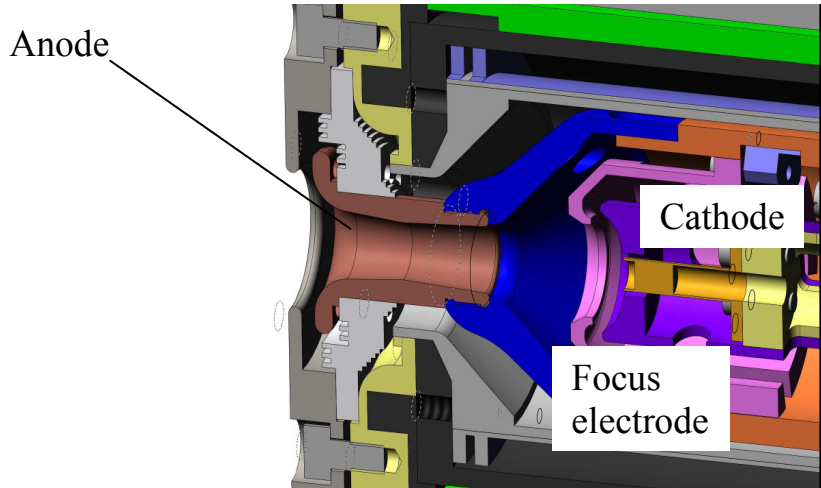
Figure 35: The new high current electron beam design will reach currents in excess of 2 A.
