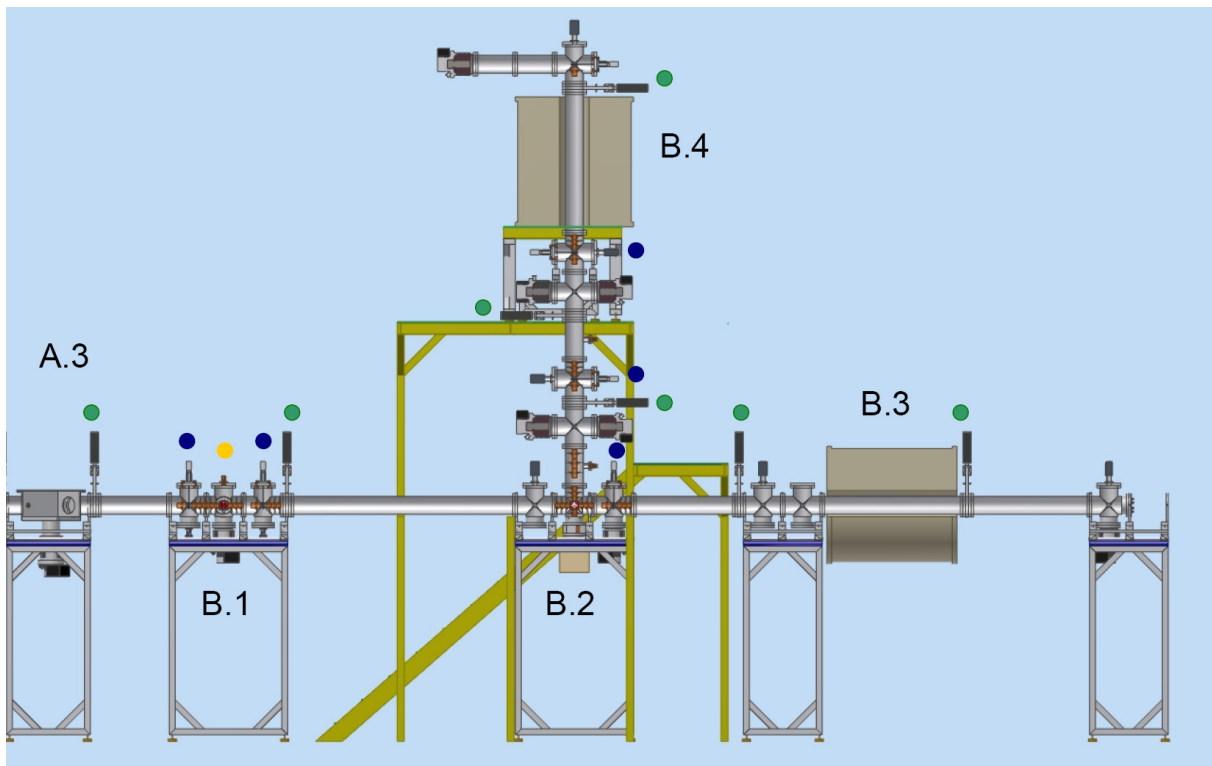
Figure 28: Overview of the MATS beamline. The different parts are named as in Figure 12. (A.3) the switchyard, (B.1) the EBIT junction, (B.2) the carbon cluster off-line ion source section, (B.3) the PPT section, and (B.4) the MPT section. In addition to the main components, Einzel lenses, and the location of beam detectors and the surface ion source are also shown. Einzel lenses are indicated in brown. The solid circles mark the location for different components. The color code stands for: blue MCP and FC detectors, green shutter valves and orange surface ion source plus quadrupole bender.
