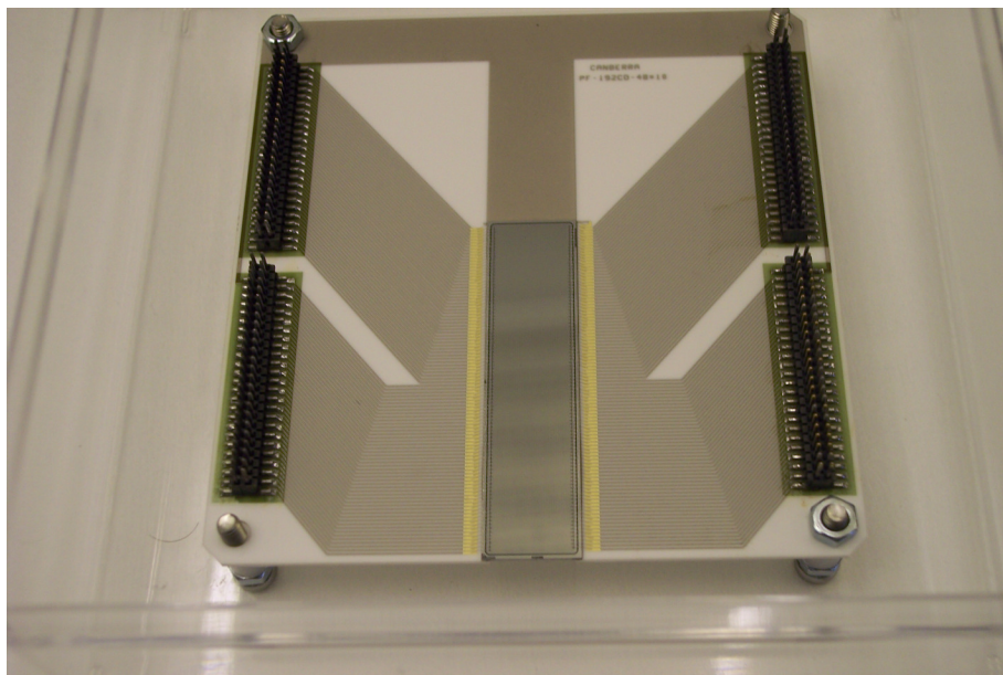
Figure 70: Picture of a silicon strip detector with a ceramic PCB currently available in the market and provided by the company CANBERRA.
