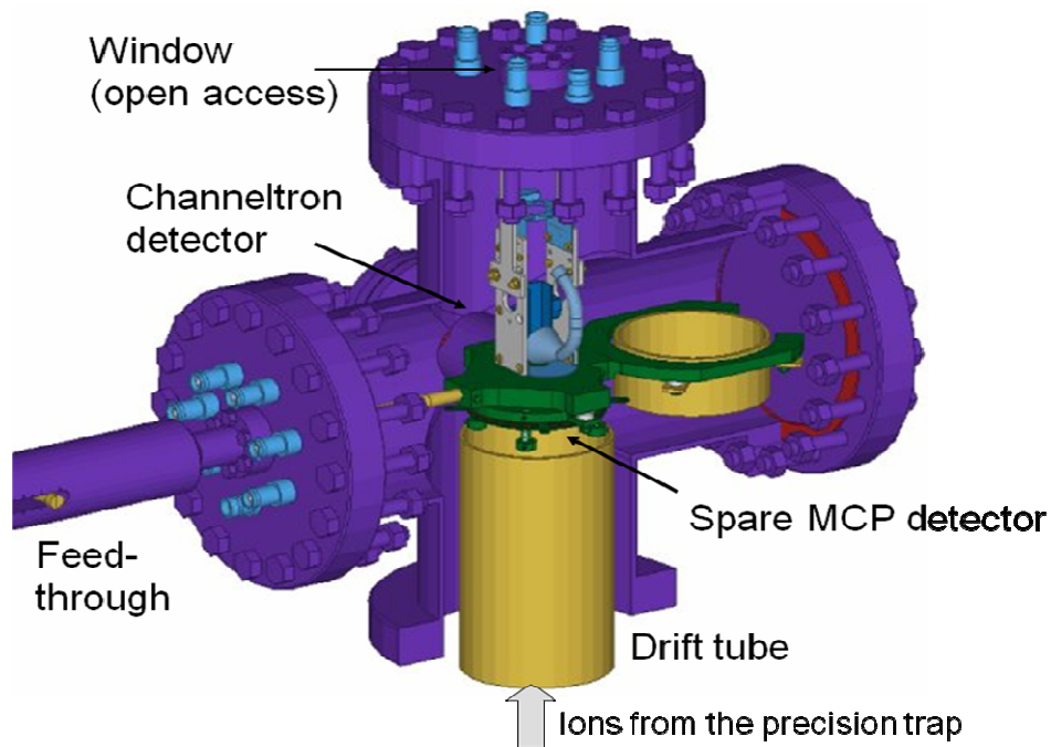
Figure 59: The ISOLTRAP design of a detector chamber with a flange-mounted CEM and linear feedthrough mounted MCP.
