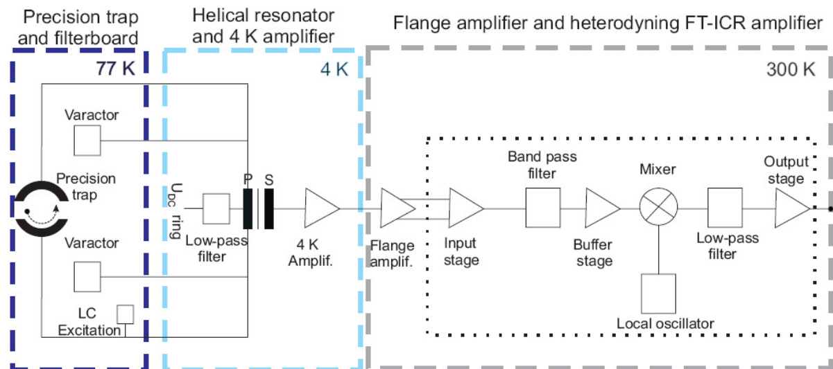
Figure 62: The narrow-band FT-ICR detection circuit [Ferr2007]. The ions induce an image current in the segments of the ring electrode of the precision trap. This current is guided to a helical resonator filter circuit, which creates a voltage drop corresponding to the current. The voltage is amplified in several stages prior to a discrete Fourier transformation revealing the frequencies of the ion motion in the trap.
