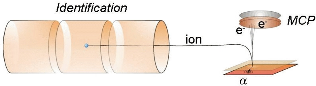
Figure 73: Schematics of the experimental setup envisaged for studies of \alpha decays from high-spin isomeric states.
