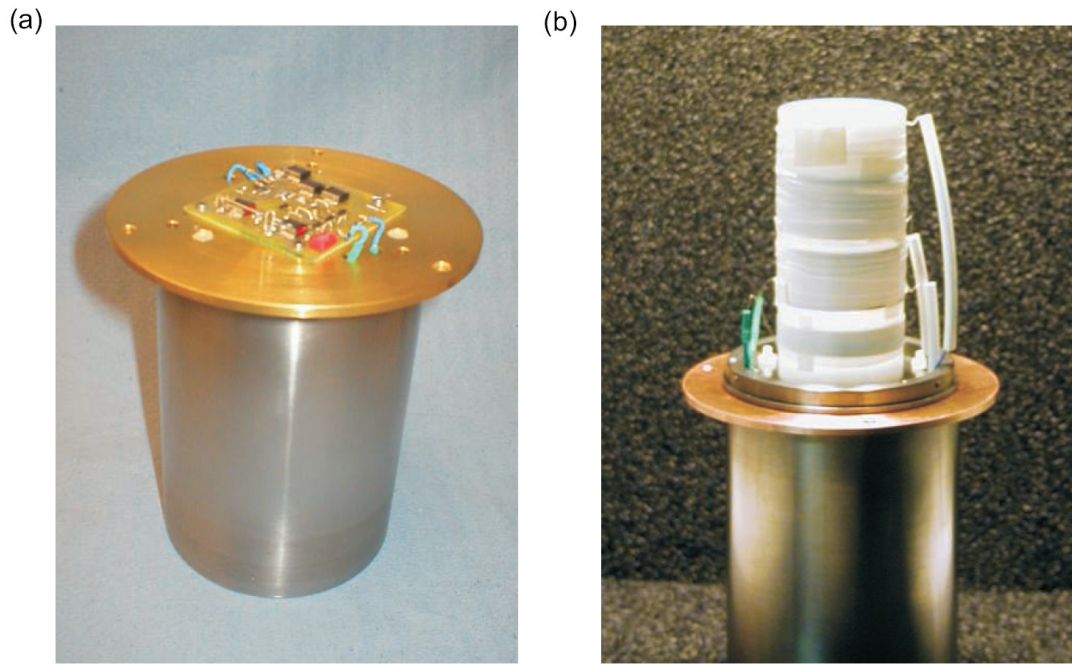
Figure 63: (a) Photograph of the NbTi shield to form a helical resonator. (b) Photograph of the NbTi coil transformer.
