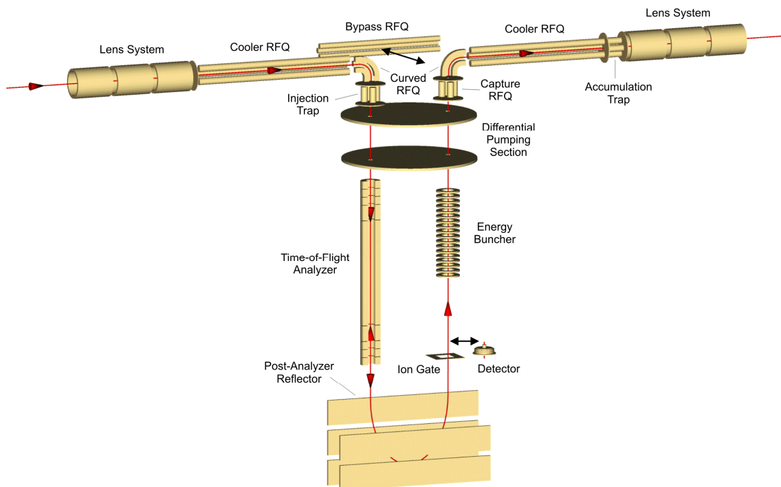
Figure 22: Schematic figure of the MR-TOF-MS system. The main functional elements are shown only, without focusing and deflection electrodes. The overall height of the device is about 2 m, the kinetic energy of the ions amounts to 1.5 keV.
