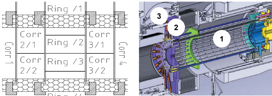
Figure 49: Left: technical drawing for the central electrodes of the preparation Penning trap. The separation between adjacent electrodes is 0.5 mm. The ring electrode is four-fold segmented. Right: technical drawing of the electrical connections for the preparation Penning trap [Maer2008]: 1) Wires, 2) radial connector rings, and 3) external feedthroughs.
