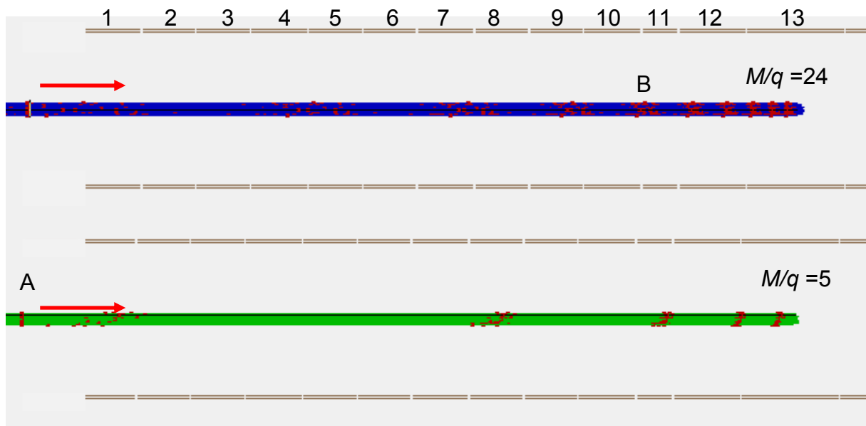
Figure 48: SIMION simulation of extraction of the ions from the trap. When the ions with lower mass-to-charge ratio reach position A (out of the trap), the ions with higher mass-to-charge ratios are still in position B close to the center of the trap (middle of segment number 13). Switching back the potential to the trapping configuration (shown in Figure 46) will confine the ions with higher mass-to-charge ratio (laser-cooled ions) in the trap. The red arrows represent the direction of the laser beam.
