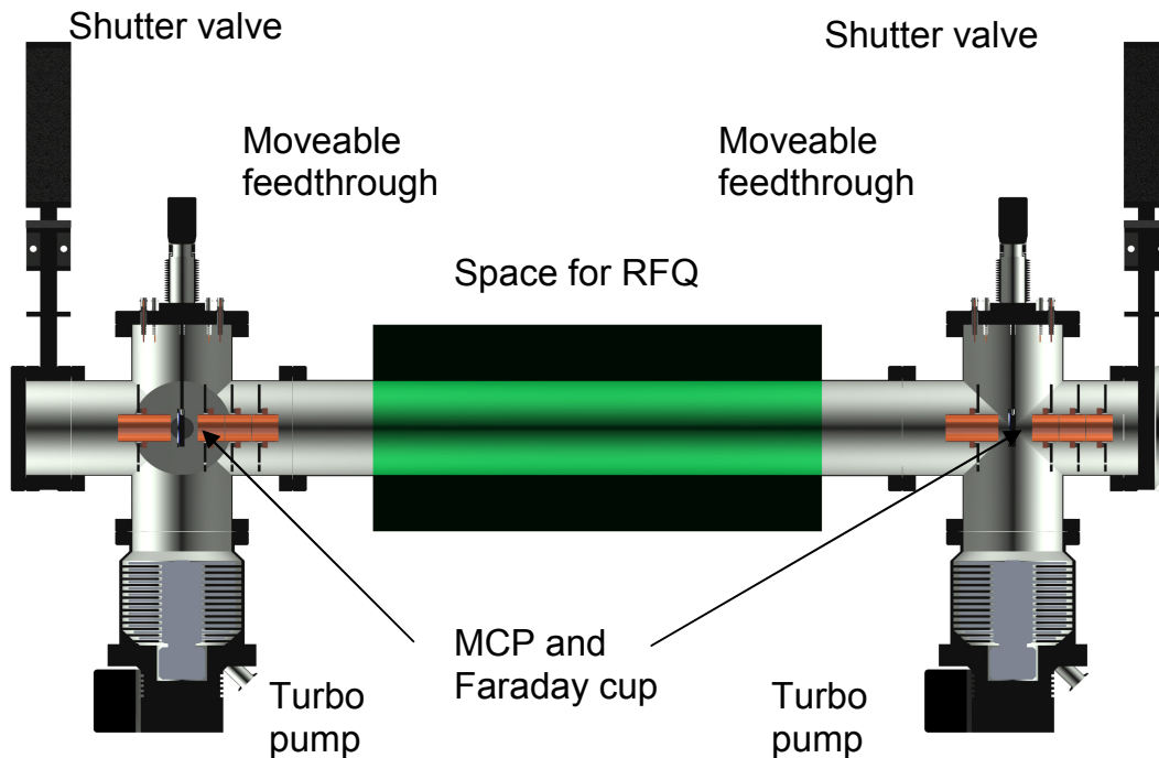
Figure 14: Location of detectors for buncher section: the incoming beam and the extracted bunches can be probed by detectors: an MCP or Faraday cup (in front) and an MCP behind.
