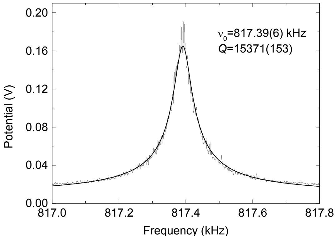
Figure 65: Resonance spectrum of the unloaded circuit. The quality factor is measured to be Q=15370\pm150 and \nu_0=817.39\pm0.06 kHz.
