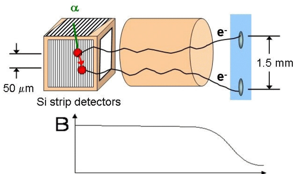
Figure 66: Schematics illustration of the proposed setup of a ‘detector trap’ for coincident in-trap \alpha and electron spectroscopy aiming at the measurement of nuclear lifetimes of 2^+ states via a measurement of the flight distance between the position of the populating \alpha decay and the subsequent conversion decay. The decay will be measured in a cubic structure of 4 silicon strip detectors, acting simultaneously as the central electrode of a Penning trap, while conversion and ‘shake-off’ electrons will be guided by the magnetic field to electron detectors at the exit of the trap magnet. The entrance endcap and exit electrodes of the detector trap will consist of an annular electrode plate (not visible here). A cylindrical electrode will be used to accelerate or decelerate electrons. Position-sensitive detection of the electron clouds from alpha and conversion decay will be achieved via a conventional MCP detector with delay line readout (see Sec. 3.6.1 INSTRUMENTATION FOR MASS SPECTROMETRY).
