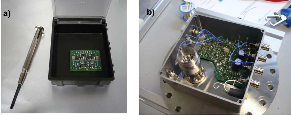
Figure 50: Left: cryogenic pre-amplifier to detect the induced image current. This amplifier is attached to the trap electrodes and is designed to be operated at cryogenic temperatures. Right: Amplifier located outside the trap. The system has been tested at the MPI-K and has given a noise signal of 2 \text{ nV}/\sqrt{\text{Hz}} [Ubie2009].
