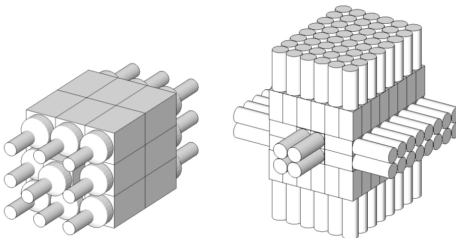
Figure 75: The DESPEC Total Absorption Spectrometer. Left) NaI(Tl) option; right) LaBr 3 :Ce option.
