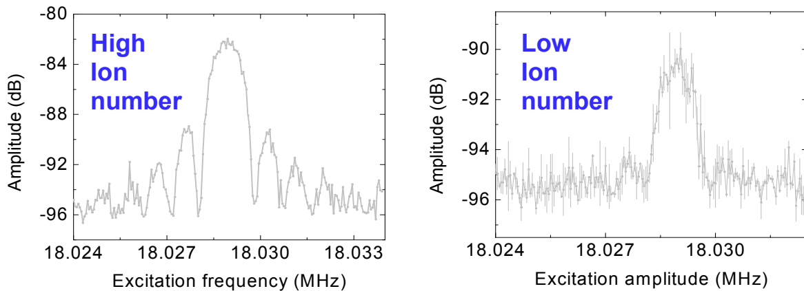
Figure 51: Reduced-cyclotron frequency resonance for \text{He}^+ ions. The difference between the two plots is the number of ions stored in the trap. In both cases the duty cycle was 100 ms. After trapping, a waiting time of 70 ms was applied before excitation. The excitation time was 1 ms. The side bands observed comes from the finite excitation time (square pulse). The mass resolving power M/\Delta M is 1.6 \times 10^4 . The calibration between ion number and amplitude of the FT-ICR signal was measured for water ions. Based on those measurements, the left panel of the figure arises from 18,000 ions stored in the trap while the second panel is produced by less than 6,000 ions.
