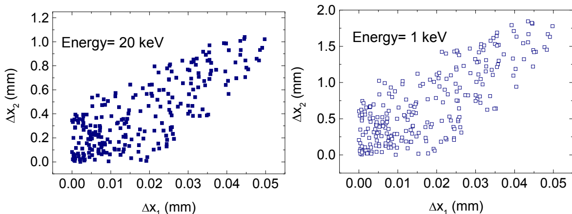
Figure 68: Comparison from SIMION simulations showing the differences in the x direction between the two electron clouds emitted after the alpha decay and after electron conversion. The picture is similar for the y direction. The beam axis coincides with the z direction. The subscripts 1 and 2 represent ions in the trap and ions at the detector plate, respectively. The ions were created assuming a magnetron radius of 0.5 mm and a cyclotron radius of 25 \mu\text{m} . The electron cloud was moved 50 \mu\text{m} in the radial direction to account for the motion of the recoil ions after the alpha decay. The energy spread is 5 %.
