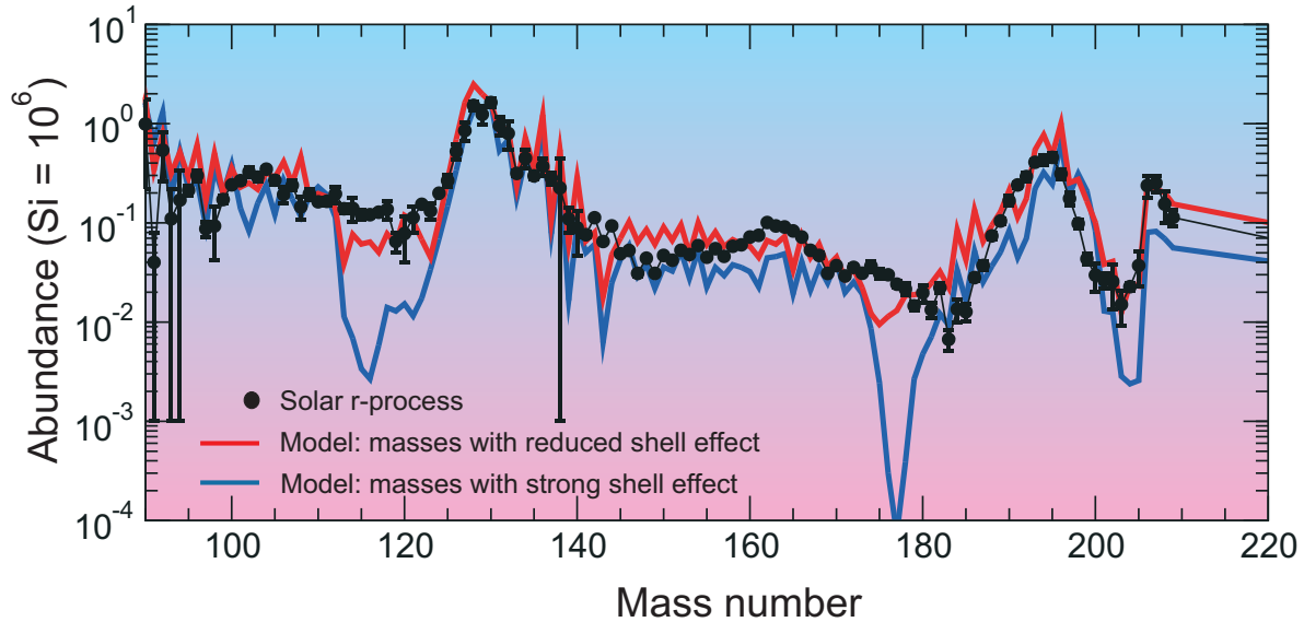
Figure 6: (Color online) Contribution of the r -process to the isotopic abundances of the chemical elements in the Solar System as a function of the mass number ("solar r -process"). This distribution is obtained by subtracting calculated contributions from the s -process and other, less important, processes from the observed solar abundance distribution. The abundances are given in usual units relative to one million silicon nuclei. The importance of reliable nuclear masses and nuclear structure information is demonstrated by showing the calculated abundances produced in two r -process models using different theoretical models to predict the nuclear masses (Data from K.-L. Kratz and B. Pfeiffer, University of Mainz, Germany [Pfei2001]).
