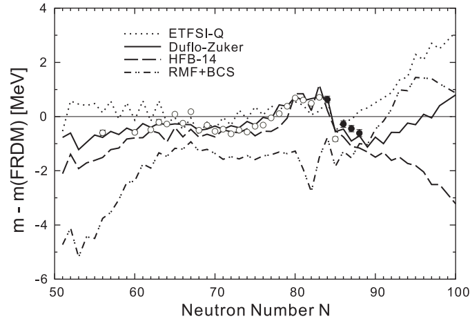
Figure 7: Mass comparison between model predictions and experimental data of iodine isotopes (from Ref. [Sun2008a])
