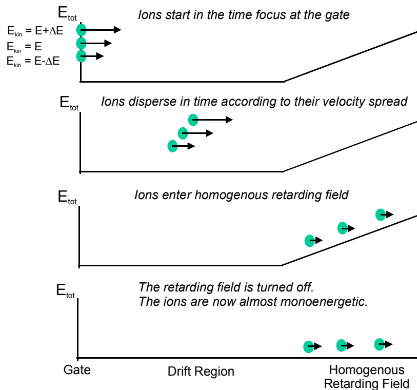
Figure 27: Schematic figure illustrating the technique of the dynamic energy buncher. A homogenous retarding field removes kinetic energy from the ions. After turning off the retarding field, the ions are almost monoenergetic.
