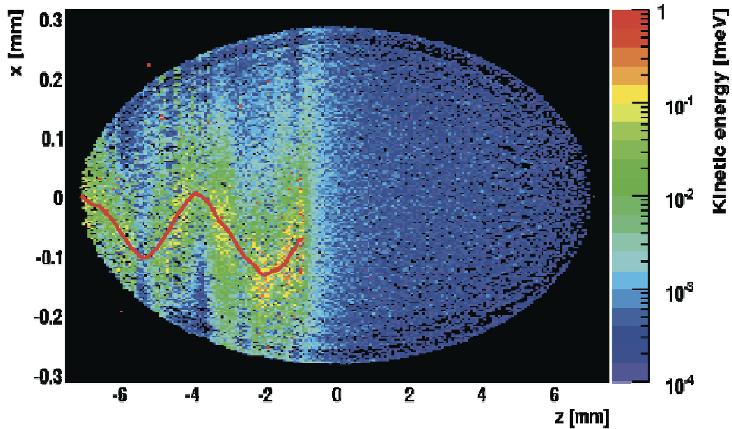
Figure 47: Energy evolution of a HCI as a function of axial distance in a \text{Mg}^+ Coulomb crystal. The picture is taken from Ref. [Buss2006].
