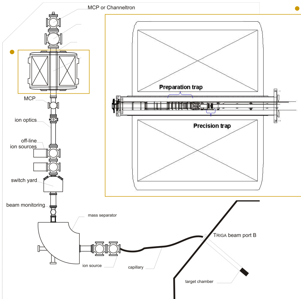
Figure 43: Top view of the TRIGA-TRAP system. The double Penning trap system housed in one superconducting magnet is shown in detail in the right part of the figure. The system is currently under commissioning at the TRIGA reactor at Mainz. This system will be installed at MATS in the first stage to prepare ions and to perform high-precision mass measurements using singly-charged ions.
