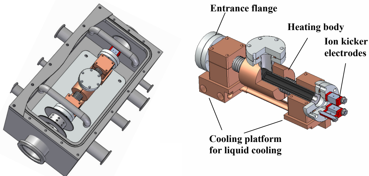
Figure 87: Left: Charge exchange cell on the high voltage platform of the LaSpec atom beam line housed in the vacuum chamber. Right: Cut view of the charge exchange cell.
