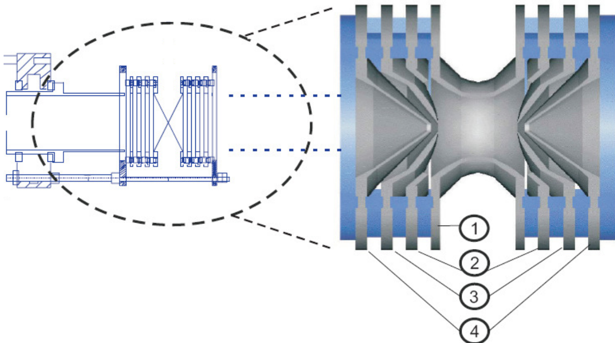
Figure 52: Technical drawing and cutaway zoomed view of the precision trap. In addition to the hyperbolical ring (1) and endcap (2) electrodes, the respective correction electrodes (3 and 4) can be seen. Sapphire pieces are used as insulators. (Technical drawings of the different parts are shown in Figure 54).
