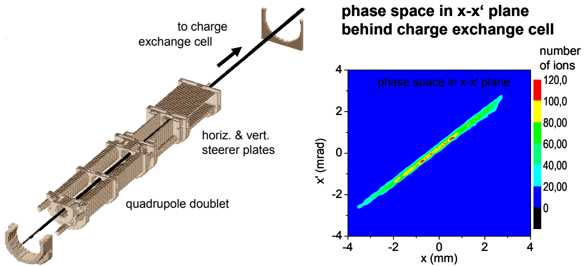
Figure 86: Atom beam line ion optics module design, taken from the former GSI mass separator beam line experiment and simulated phase space of the ion beam in the detection region for a realistic ion beam distribution entering the 10^\circ deflector chamber.
