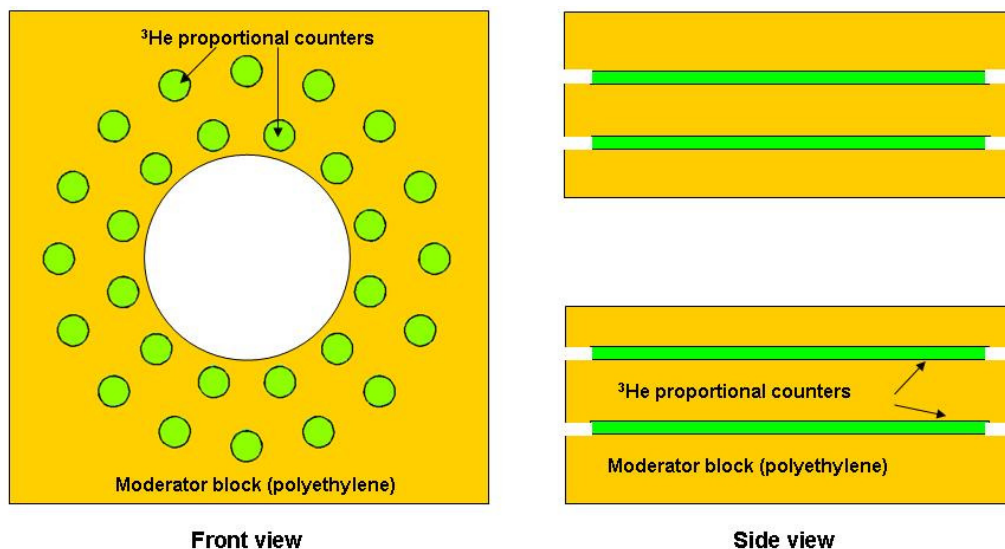
Figure 76: Sketch showing the front and side view of the 4\pi neutron detector.
