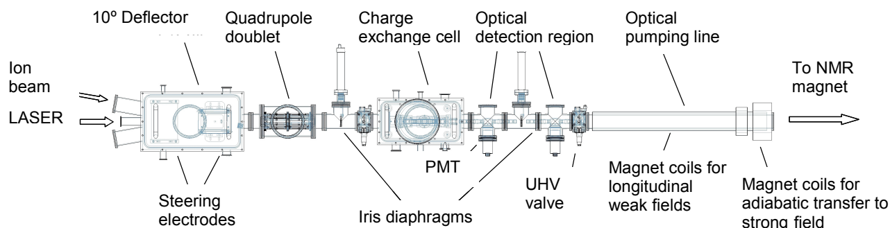
Figure 84: Technical drawing of the optical pumping and fast atomic beam laser spectroscopy line. Support frames omitted for clarity.
