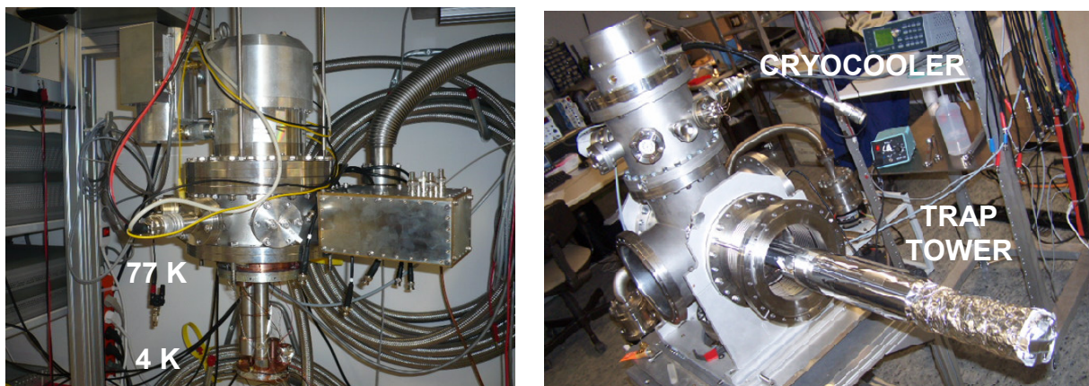
Figure 45: Left: two stage cryocooler from SUMITOMO Heavy Industries Ltd. This system is the one foreseen to cool down the preparation Penning trap at MATS. Right: cryocooler from VERICOLD placed on top of a vacuum cross to cool down a Penning trap system to be housed in a horizontal superconducting magnet.
