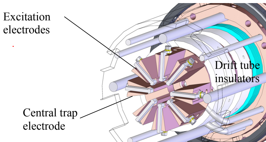
Figure 34: Section of the central drift tube of the Heidelberg EBIT design. It allows for selective cyclotron excitation of the trapped ions in the magnetic trapping mode.
