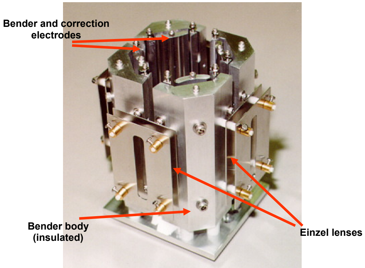
Figure 39: Picture of the quadrupole bender used for injecting SCI into an EBIT. The implementation in SIMION of such a system is shown in Figure 40.
