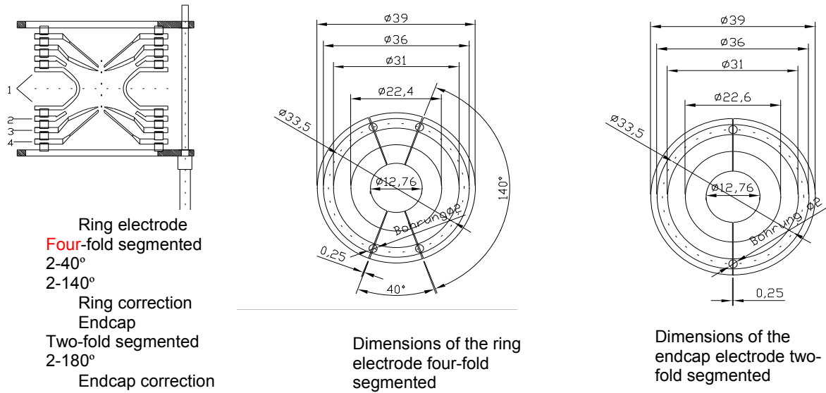
Figure 54: Technical drawing of the different parts of the hyperbolic measurement trap. From left to right: 1) assembly, 2) ring electrode and 3) endcap electrode.
