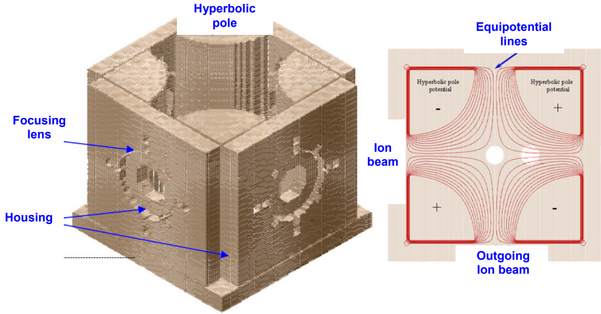
Figure 40: Left: assembly of the quadrupole deflector in a square box. The upper flange has been removed to allow for the observation of the quadrupole. Right: equipotential lines for the quadrupole.
