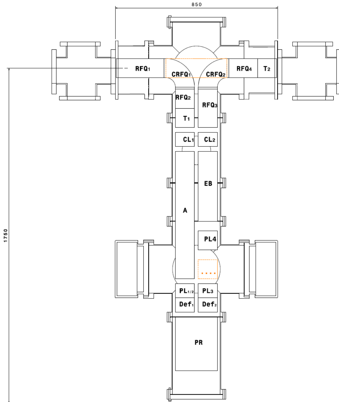
Figure 24: technical drawing of the MR-TOF-MS system. The different elements depicted in Figure 22 are shown. The different acronyms stand for: RFQ Radio Frequency Quadrupole; CRFQ curved RFQ; T linear Paul trap; CL cylindrical lens; A analyzer; PR post-analyzer reflector; PL planar lens; D detectors; G Bradbury-Nielsen gate; BC beam camera; EB energy buncher. The length in the beamline is 85 cm.
