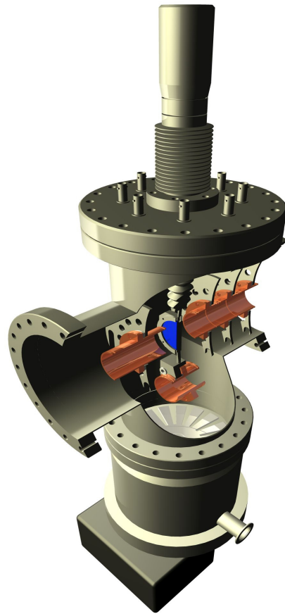
Figure 31: Mounting of an MCP detector in a CF-160 cross together with optical lenses.
