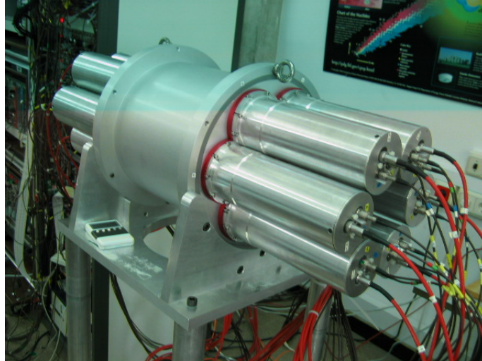
Figure 74: The BaF 2 Total Absorption Spectrometer.
