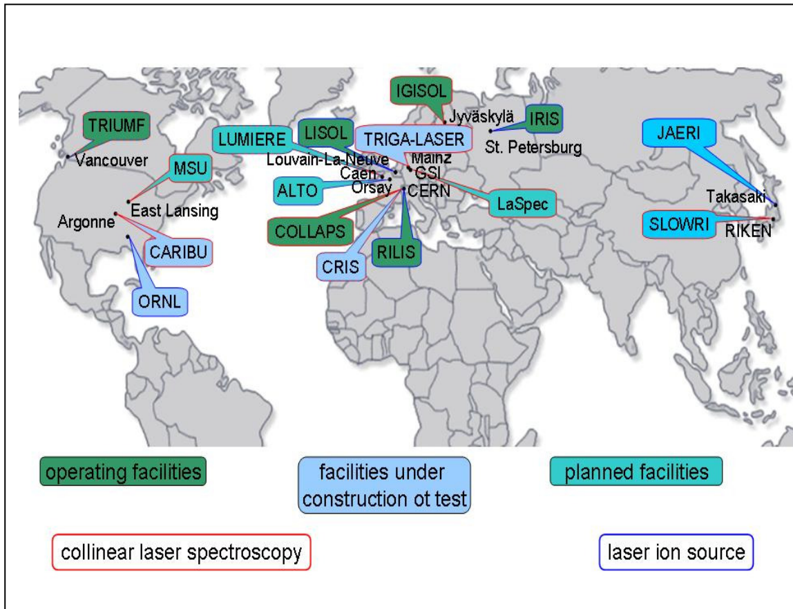
Figure 11: Overview of laser spectroscopy and laser ion source installations at on-line facilities worldwide
