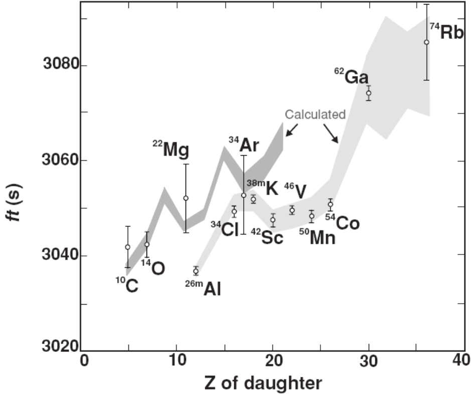
Figure 2: Experimental ft -value plotted as a function of the charge of the daughter nucleus, Z . The bands represent the theoretical quantity Ft/[(1+\delta_R)(1-\delta_C)] . The two groups distinguish those \beta emitters whose parent nuclei have isospin T_z = -1 (dark shading) from those with T_z = 0 (lighter shading) [Hard2009].
