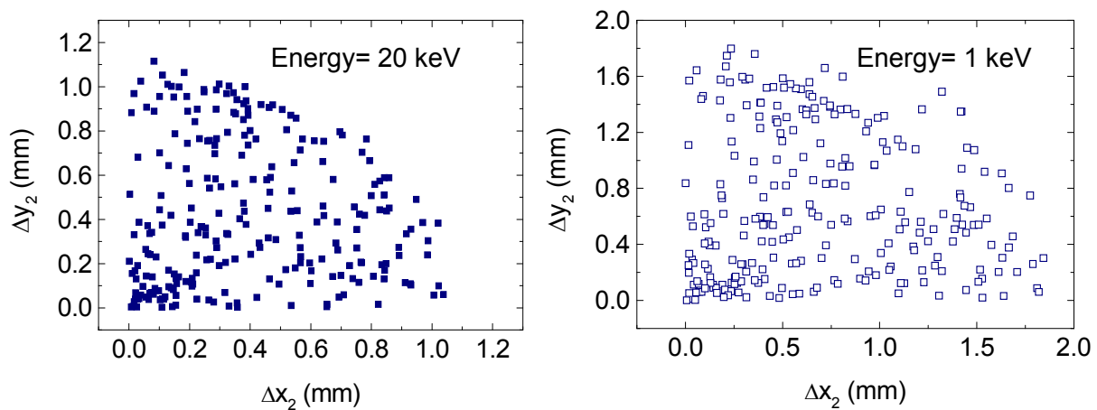
Figure 69: Difference in position impact in the y direction versus the x direction at the detector plane between the electrons from the alpha decay and electrons from conversion. The results are obtained from the same simulations as in Figure 68. The fact that there is not a circumference with a radius around 1 mm (left) or around 1.8 mm (right) is due to the z direction. The point (0,0) would correspond to a motion of the recoil nucleus in the z -direction.
