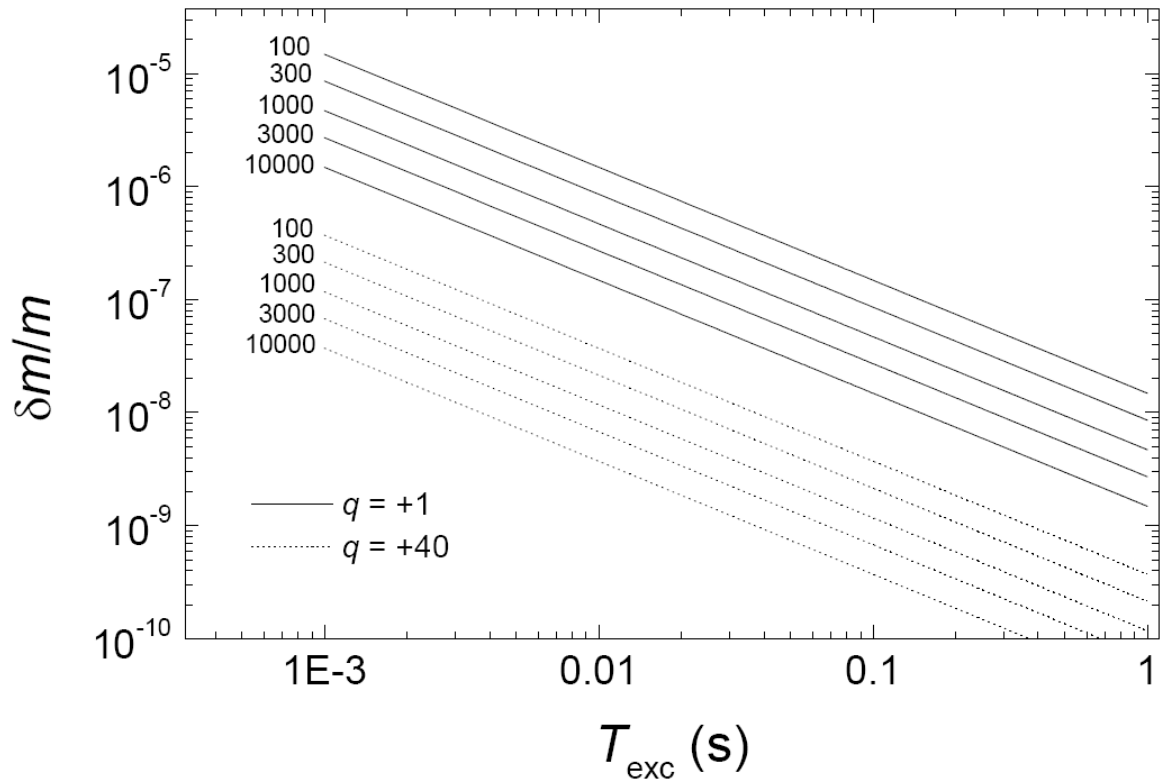
Figure 80: The achievable mass uncertainty for a nuclide with mass A = 100 u as a function of the excitation time in the Penning trap ( B = 7 T) for two sets of charge states and different numbers of detected ions. The upper set of curves belongs to singly-charged ions, the lower set of curves to ions in the charge state +40.
