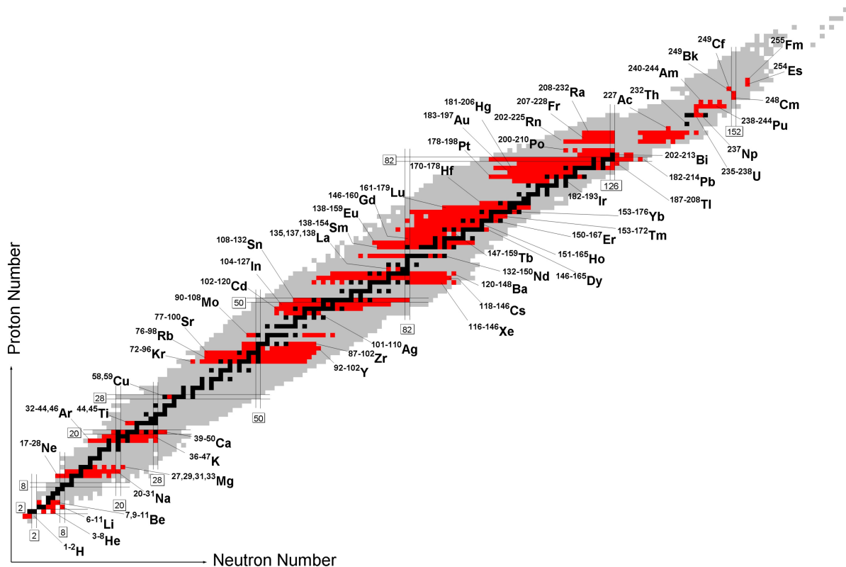
Figure 10: Chart of nuclei showing the isotopes for which optical spectroscopy was performed on-line in long isotopic chains or on nuclei far from stability (red). Black squares indicate stable nuclei, light-gray are those nuclei known to exist as bound systems. Above uranium, the experiments were performed off-line with the exception of ^{240f,242f,244f}\text{Am} ( http://www.gsi.de/forschung/ap/projects/laser/survey.html ).
