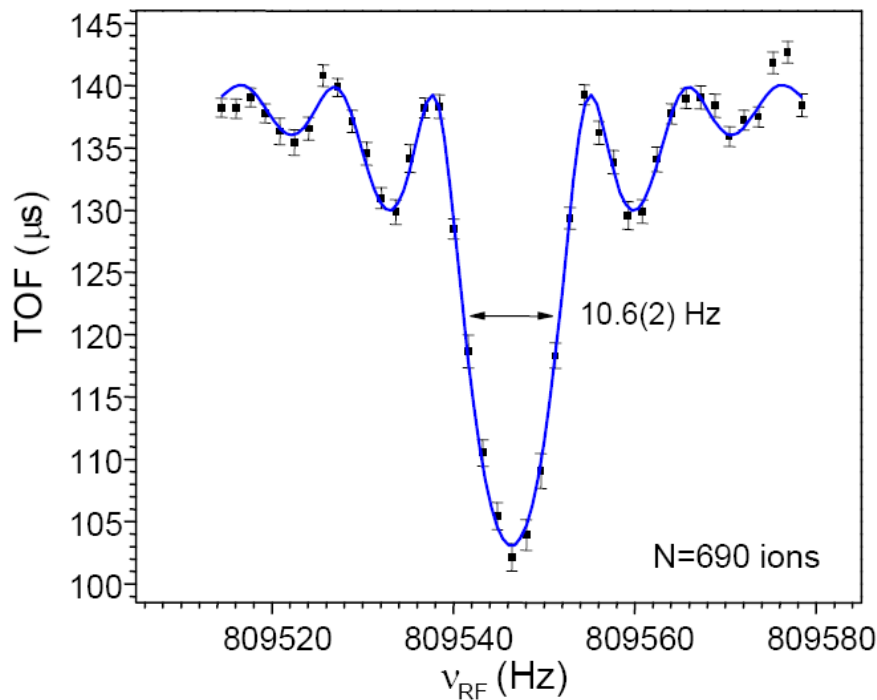
Figure 58: Time-of-Flight (TOF) resonance for \text{Cs}^+ ions. The solid line is the fit of the experimental data using the theoretical line shape described in Ref. [Koni1995]. This figure has been taken from Ref. [Elis2007].
