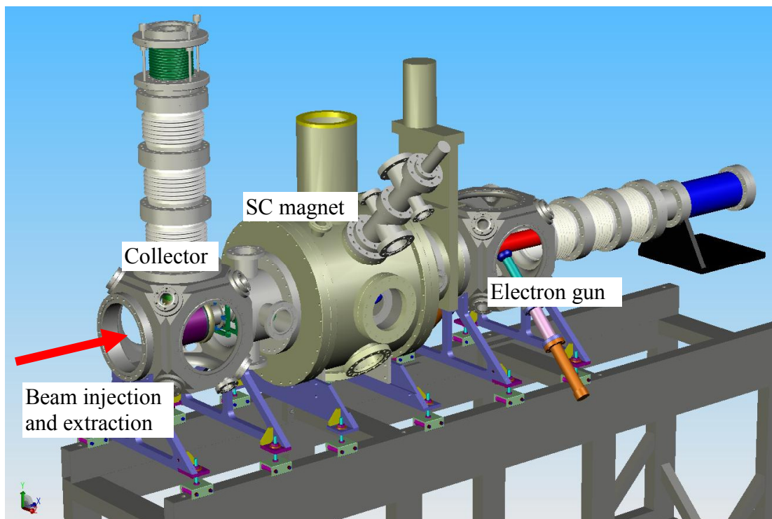
Figure 32: Overall scheme of the MATS-EBIT.
