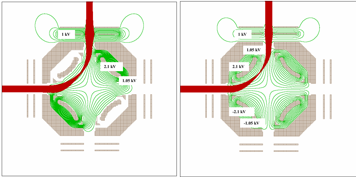
Figure 41: Q bender in symmetric configuration
