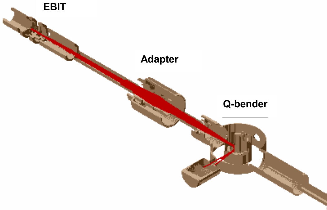
Figure 38: Simulation of ion trajectories (in red) through an electrostatic quadrupole bender to transport SCI into an EBIT. A picture of a quadrupole bender from COLUTRON is shown in Figure 39. Electrostatic lenses are provided by the companies DREEBIT and COLUTRON.
