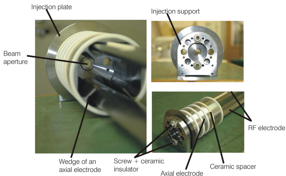
Figure 19: The figures display the main parts of the RF and axial electrodes together with the insulators.
