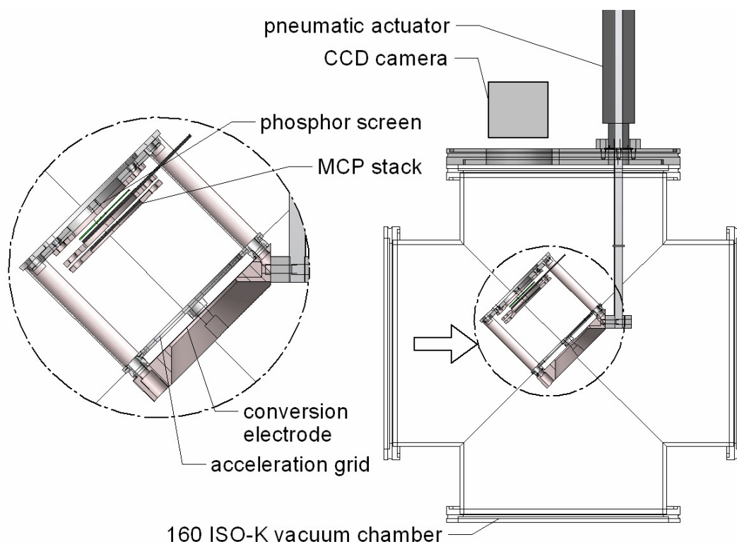
Figure 89: Ion beam monitor for ion beams with intensities of a few thousand ions per second. The ion beam coming from the left hits a conversion electrode. The emitted electrons are accelerated by a grid on a variable potential, then amplified by a stack of MCPs and imaged on a phosphor screen, which is monitored by a CCD.
