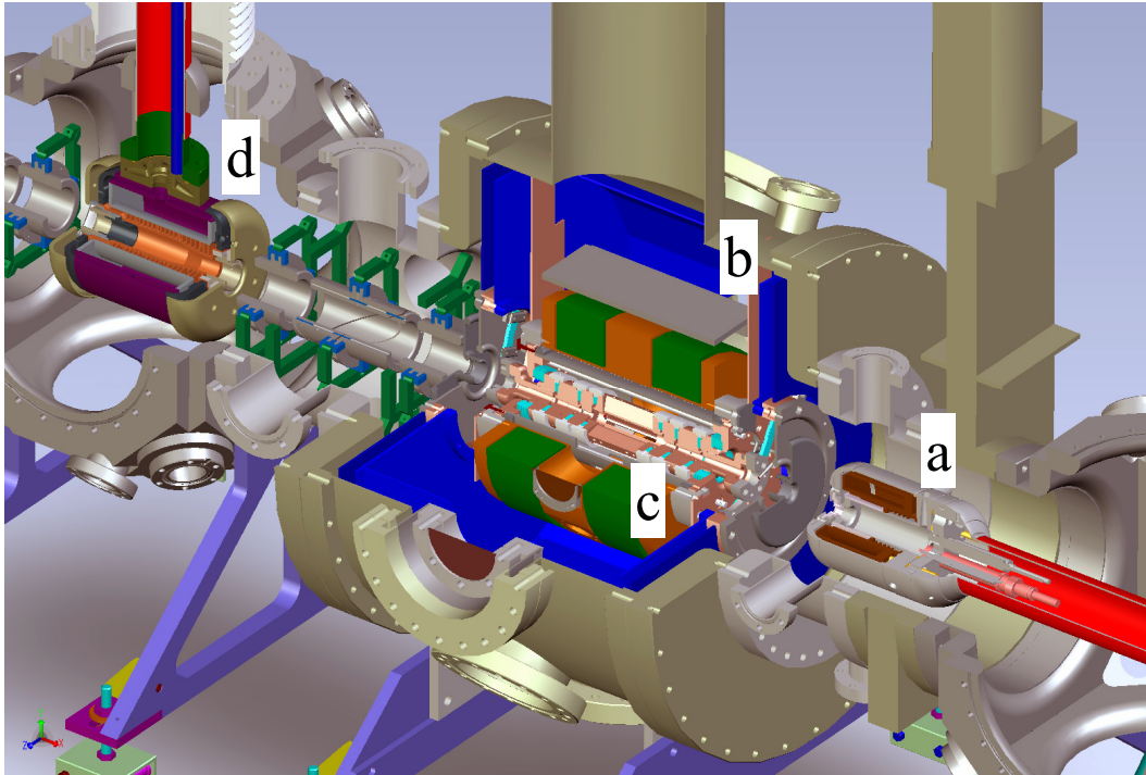
Figure 33: Section through the electron gun (a), magnet chamber (b), drift tube trap section (c) and collector (d) of the Free Electron Laser (FEL) in Hamburg, FLASH. Ion injection and extraction proceed through the collector (d).
