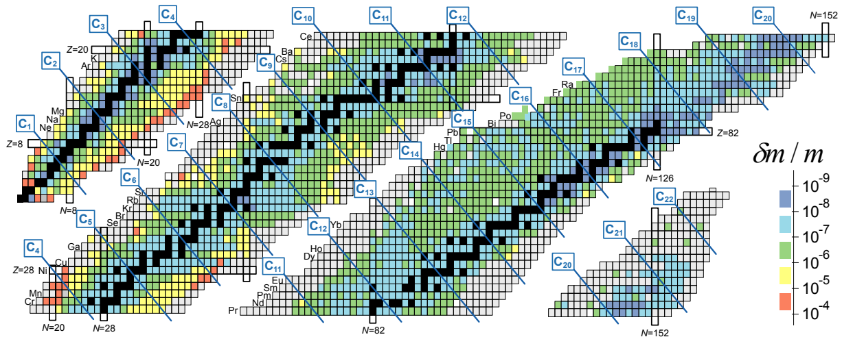
Figure 8: Nuclear chart with the relative mass uncertainties \delta m/m of all known nuclides shown in a color code (see scale bottom right of the nuclear chart - stable nuclides are marked in black) [Blau2005a]. Masses of gray-shaded nuclides are estimated from systematic trends [Audi2003]. The isobaric lines of the carbon clusters C_1 to C_{22} demonstrate the advantage of using a “carbon cluster mass grid” for calibration purposes [Blau2002].
