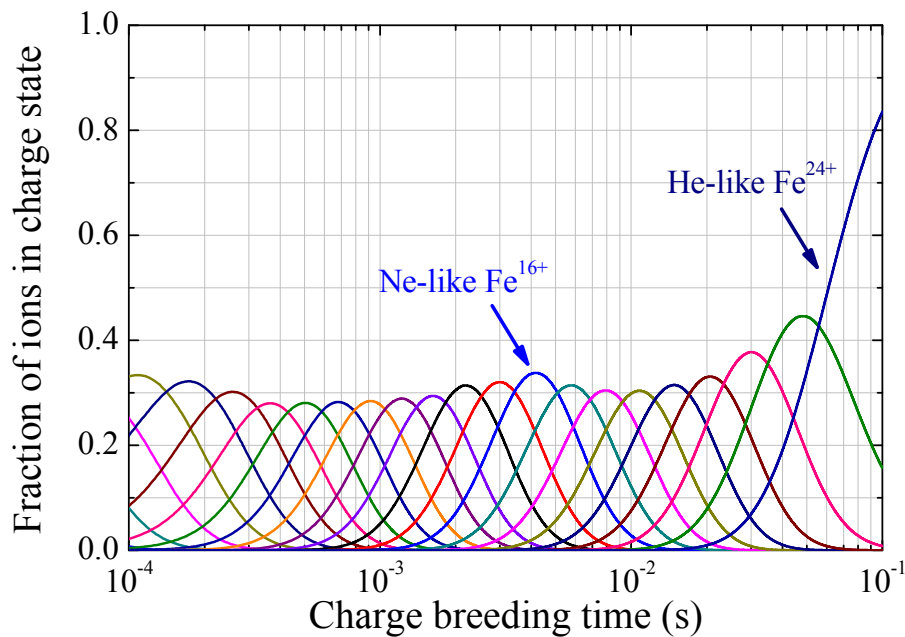
Figure 36: Evolution of the charge state of Fe ions after injection into the EBIT at 2 A beam current with a moderate electron/ion overlap of 2%, equivalent to a 1400 A/cm 2 current density
