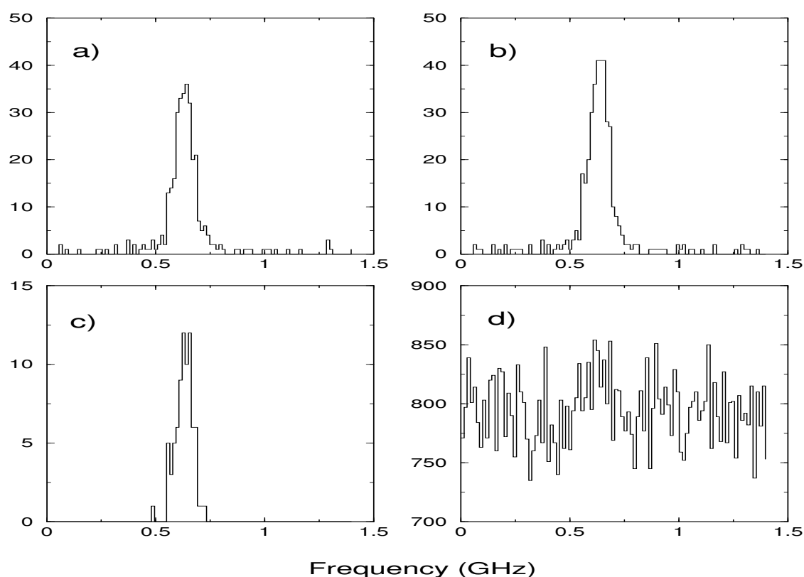
Figure 83: Burst spectroscopy of a 40,000/s niobium ion beam showing a single hyperfine resonance observed with a) a 15 \mu s observation window, b) a 25 \mu s observation window, c) >2 photons counted in a 25 \mu s window (the “burst” spectrum) and d) the single photon counts.
