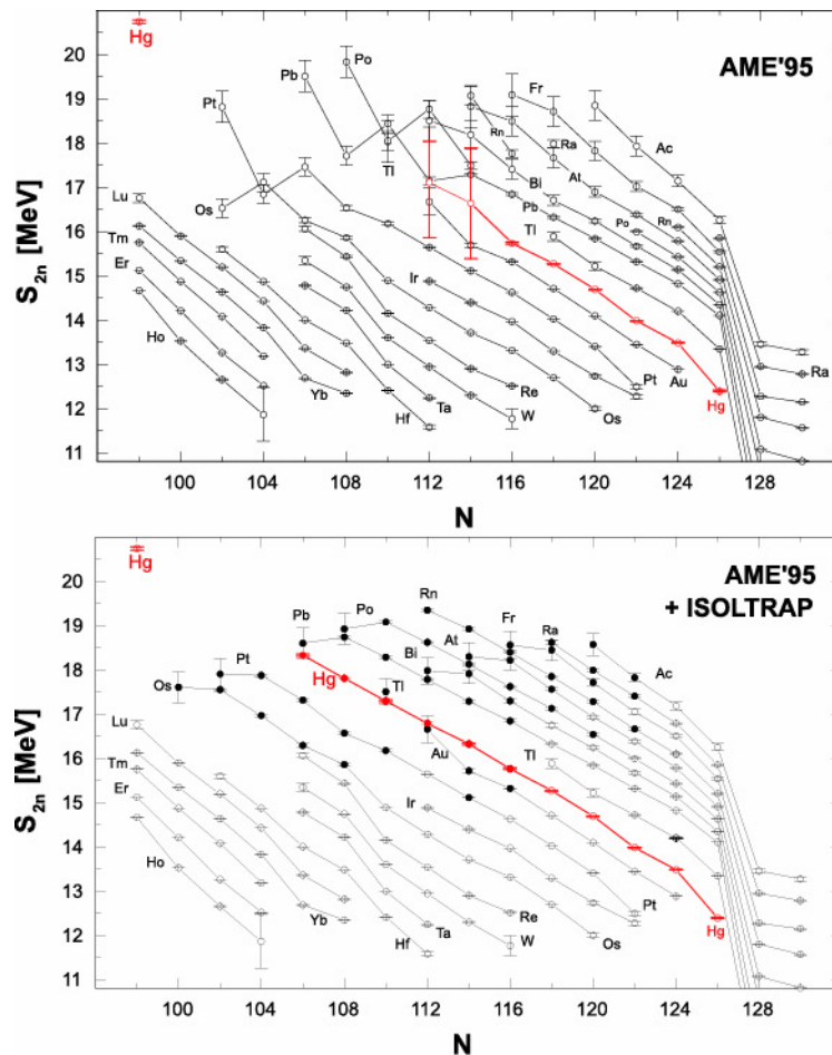
Figure 3: Two-neutron separation energies in the vicinity of Z = 82 as a function of neutron number. Shown are S_{2n} values derived from the Atomic Mass Evaluation in 1995 AME1995 (top) and a compilation including ISOLTRAP data (bottom) [Schw2001].
