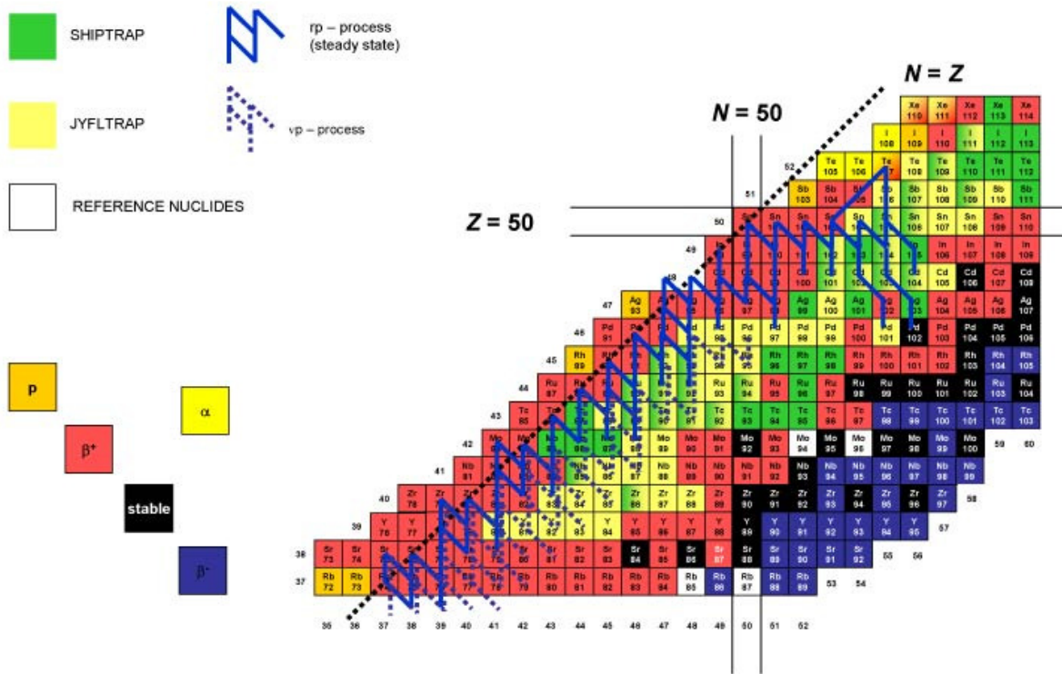
Figure 5: (Color online) Section of the nuclear chart with the upper region of the rp - and vp process pathways. Nuclides studied with the JYFLTRAP (yellow) or the SHIPTRAP (green) mass spectrometers are indicated. For a detailed review see text.
