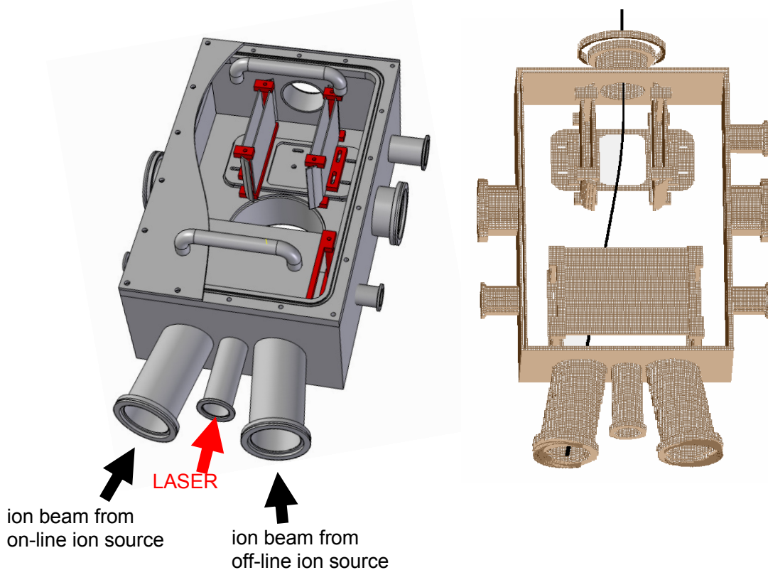
Figure 85: Technical drawing (left) showing the design of the LaSpec atomic beamline deflection chamber and ion trajectory simulations (right).
