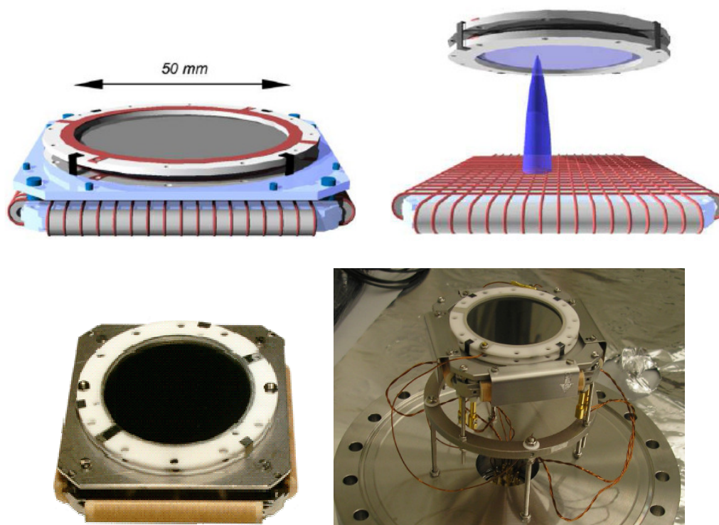
Figure 60: Position sensitive detector with delay line anode, manufactured by RoentDek.
