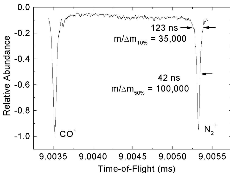
Figure 25: Mass spectrum of the isobaric doublet of \text{CO}^+ and \text{N}_2^+ obtained with the small prototype of the MR-TOF-MS. After 1433 turns, a peak width of 42 ns is measured, corresponding to a mass resolving power (FWHM) of about 10^5 . The resolving power at 10% peak height amounts to 35,000.
