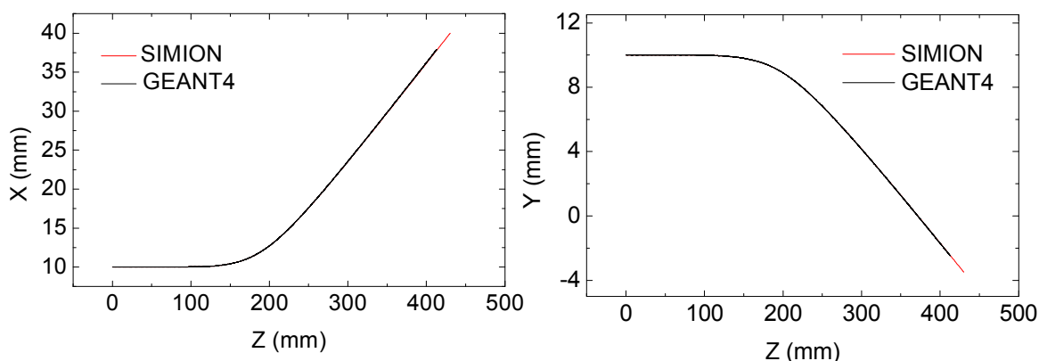
Figure 71: Simulations of \alpha -particle trajectories in a magnetic field surrounding the ‘detector trap’ and provided by the superconducting magnet shown in Figure 44. The energy of the particles is 5 MeV for this figure. The agreement between SIMION and GEANT4 was perfect for energies ranging from 1 to 10 MeV. The starting position in the radial plane was (10 mm,10 mm).
