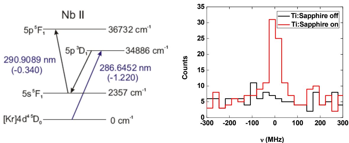
Figure 21: Optical pumping scheme for niobium and the signal obtained by collinear laser spectroscopy from the metastable state.
