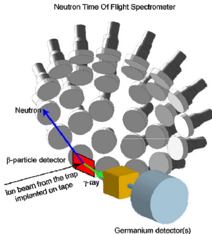
Figure 79: CIEMAT nTOF spectrometer setup as it will be used at IGISOL- Jyväskylä.
