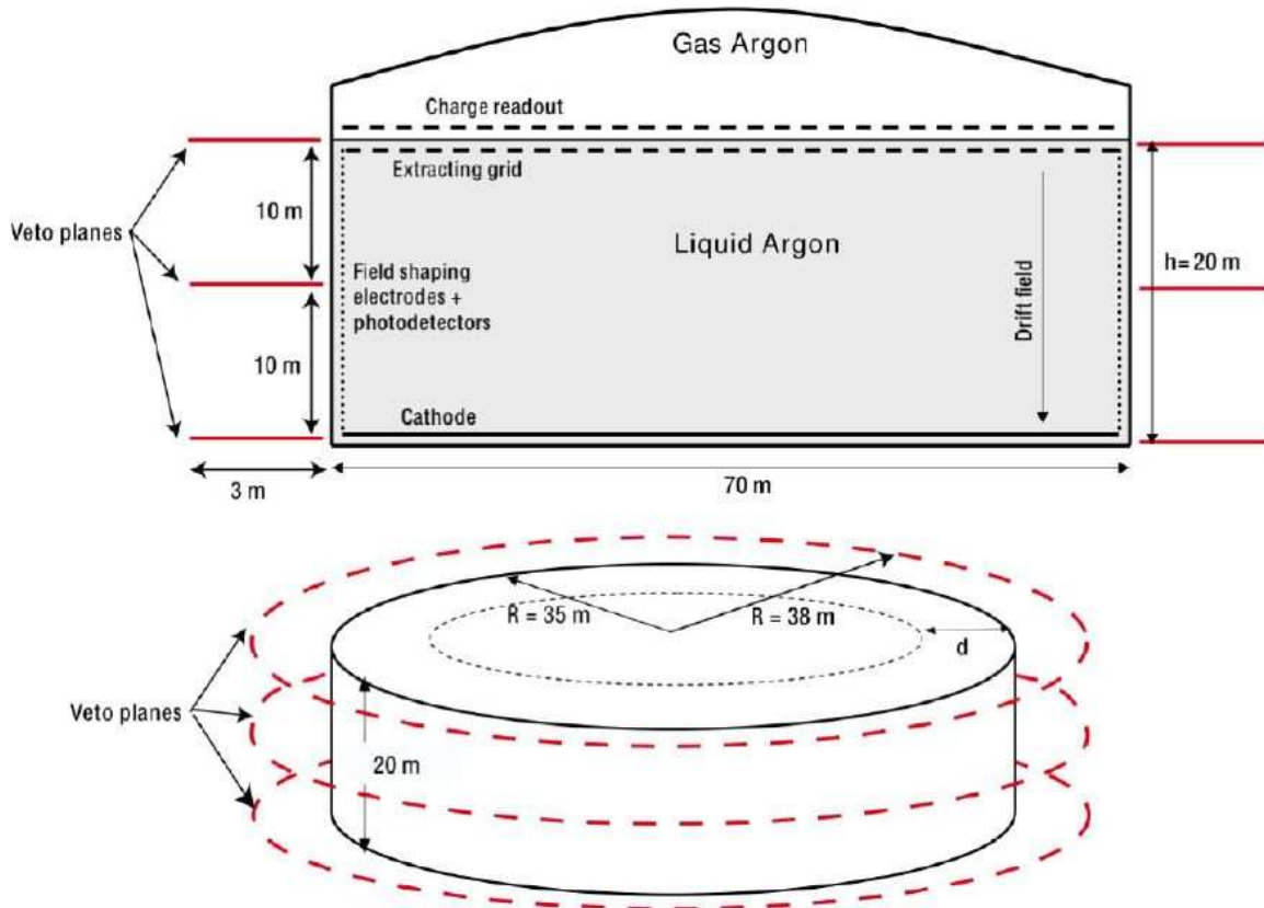
FIG. 1: Conceptual design of a 100 kton LAr TPC detector (see Ref. [51] for details). To suppress cosmogenic backgrounds, we consider the possibility to locate three large area veto planes to detect remaining penetrating cosmic ray muons passing in the vicinity of the Argon detector (see text).
