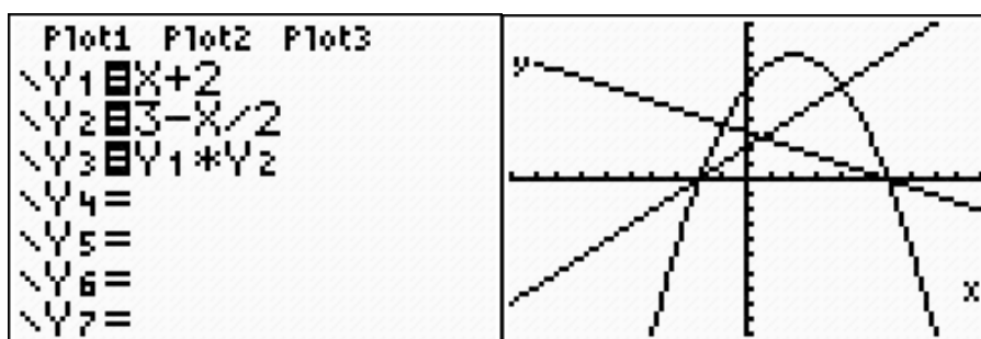
Figure 2. Exploring the product of two linear functions
