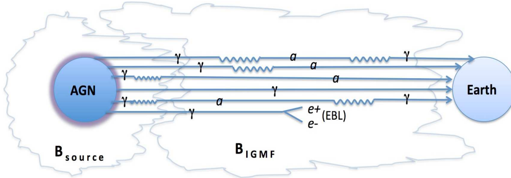
Figure 5.1 Sketch of the formalism used in this work, where both mixing inside the source and mixing in the IGMF are considered under the same consistent framework. Photon to axion oscillations (or vice-versa) are represented by a crooked line, while the symbols \gamma and a mean gamma-ray photons and axions respectively. This diagram collects the main physical scenarios that we might identify inside our formalism. Each of them are squematically represented by a line that goes from the source to the Earth.
