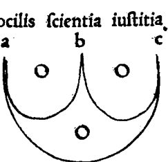
qua rectis lunares circuli lineis figuræ culis d e f
