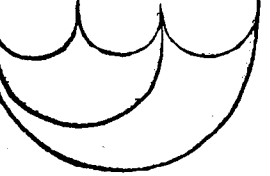
qua rectis lunares circuli lineis figuræ culis d e f
