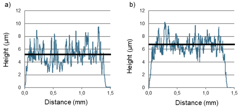
Figure 2. Comparison of the profile diagram of a printed line: a) carbon, b) silver chloride (profilometer measurements in blue, mean values in black).
