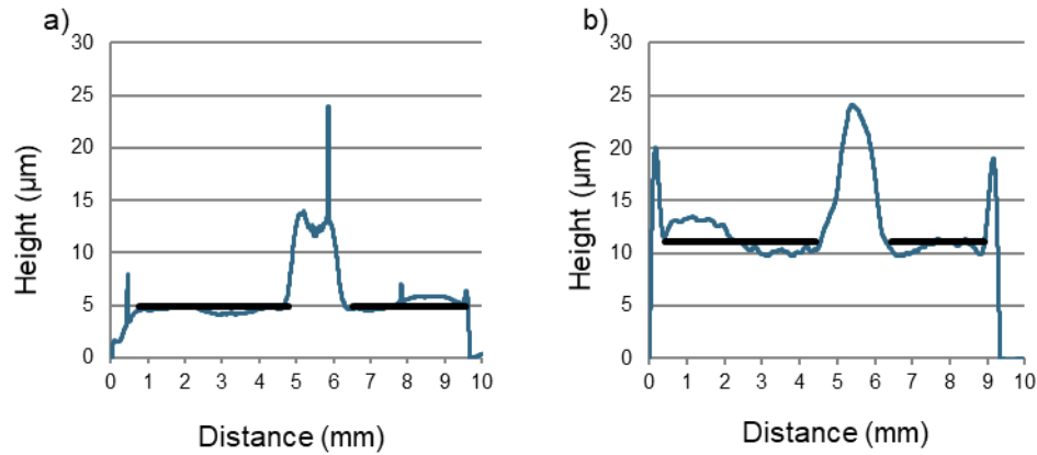
Figure 4. Comparison of the profile diagrams of a printed silver chloride line with: a) single-layer printed dielectric, b) multiple-layer printed dielectric (profilometer measurement in blue, mean in black).
