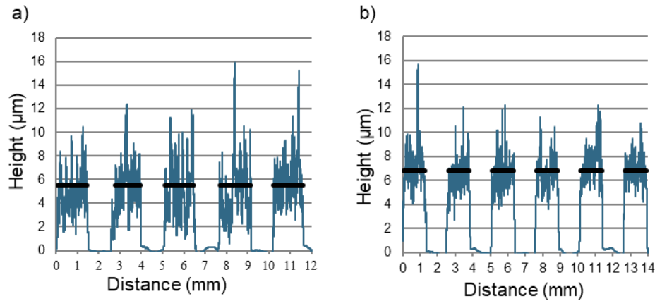
Figure 3. Comparison of the profile diagrams of several printed lines: a) carbon, b) silver chloride (profilometer measurements in blue, mean values in black).
