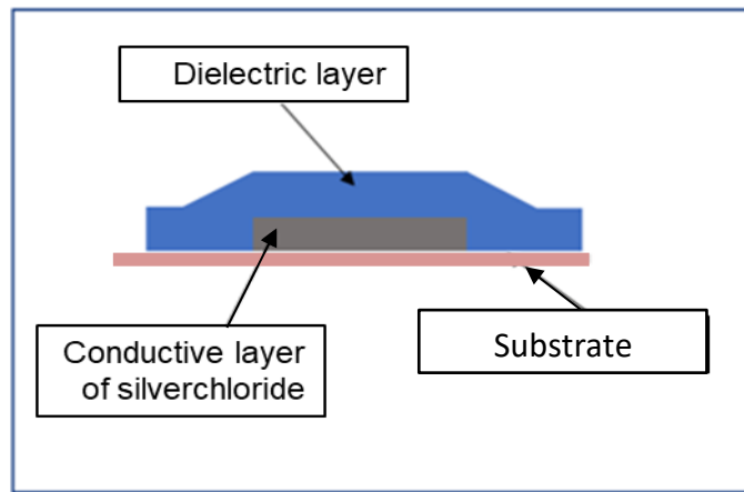
Figure 1. Cross-section scheme of the printed layers using the example of the printing of a conductor made of silver chloride with an overlying insulator.
