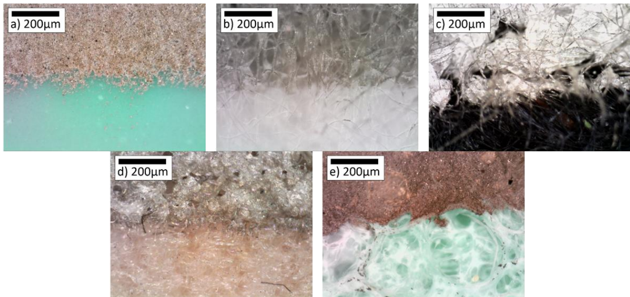
Figure 5. Selected microscope images of different substrates with printed silver paste: a) rubber glove; b) sanitary napkin; c) fabric glove; d) nylon tights; e) dishcloth. The printed silver can be observed in the top half of the images, the unprinted substrate in the bottom areas.
