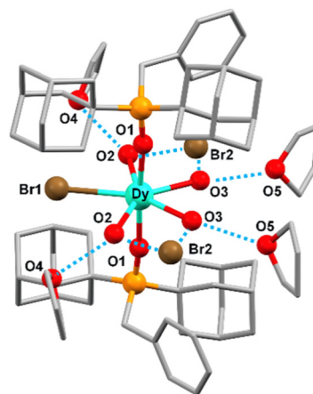
Fig. 1 Perspective view of the molecular structure of [Dy(OPAd 2 Bz) 2 (H 2 O) 4 Br] 2 Br 2 ·4THF ( 1 ). Code colours: dysprosium (cyan), oxygen (red), bromide (brown), phosphorus (orange), and carbon (grey). Hydrogen atoms are omitted for clarity. Blue dashed lines indicate hydrogen bond interactions.
