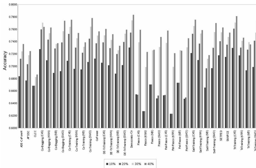
Figure 6: Labeled ratio comparison (bar chart): Inductive phase
