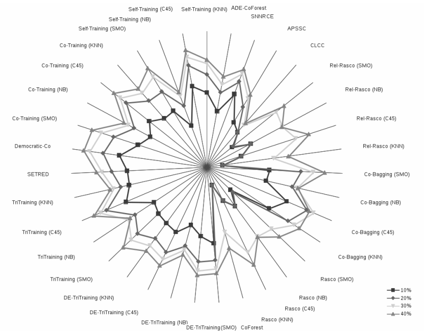
Figure 5: Labeled ratio comparison (star plot): Inductive phase
