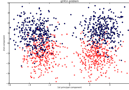
(a) g241n problem.
