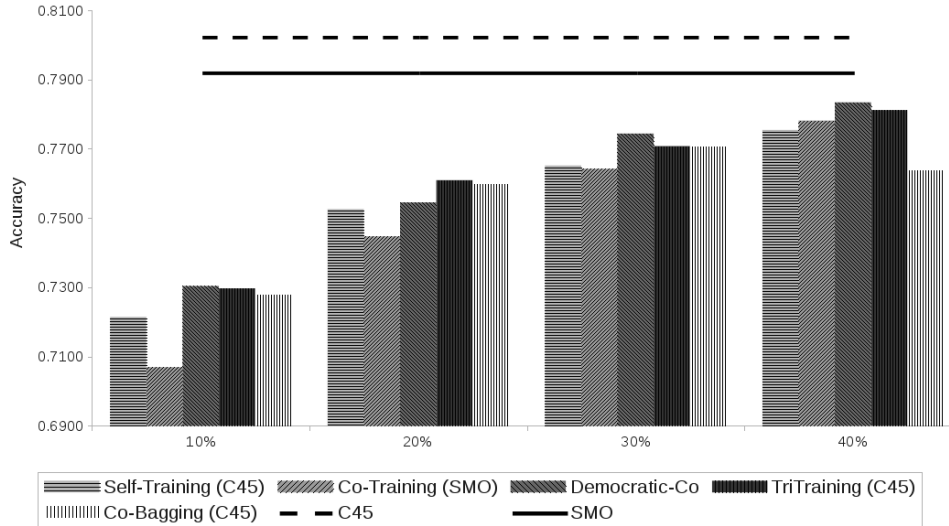
Figure 12: Differences in average test results between outstanding models and C4.5 and SMO
