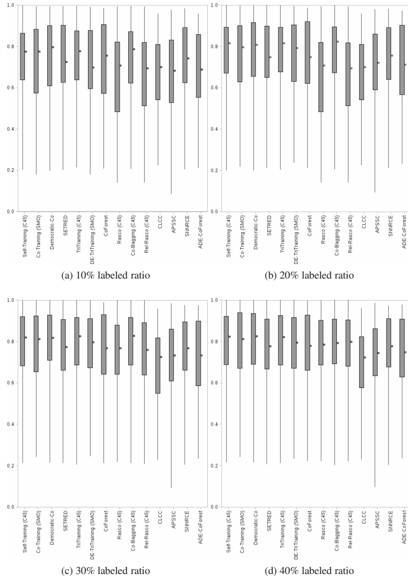
Figure 7: Box plot accuracy inductive phase
