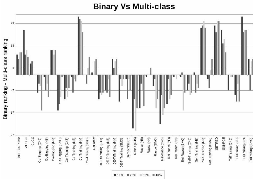
Figure 8: Differences between rankings in Binary and Multi-class domains: Inductive phase
