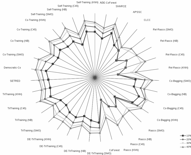
Figure 2: Labeled ratio comparison (star plot): Transductive phase
