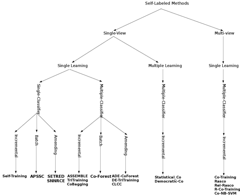
Figure 1: Self-labeled techniques hierarchy
