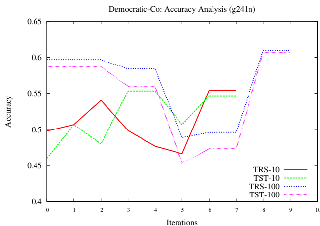
Figure 11: Transductive (TRS) and inductive (TST) accuracy of Democratic-Co in the g241n problem: 10 and 100.
