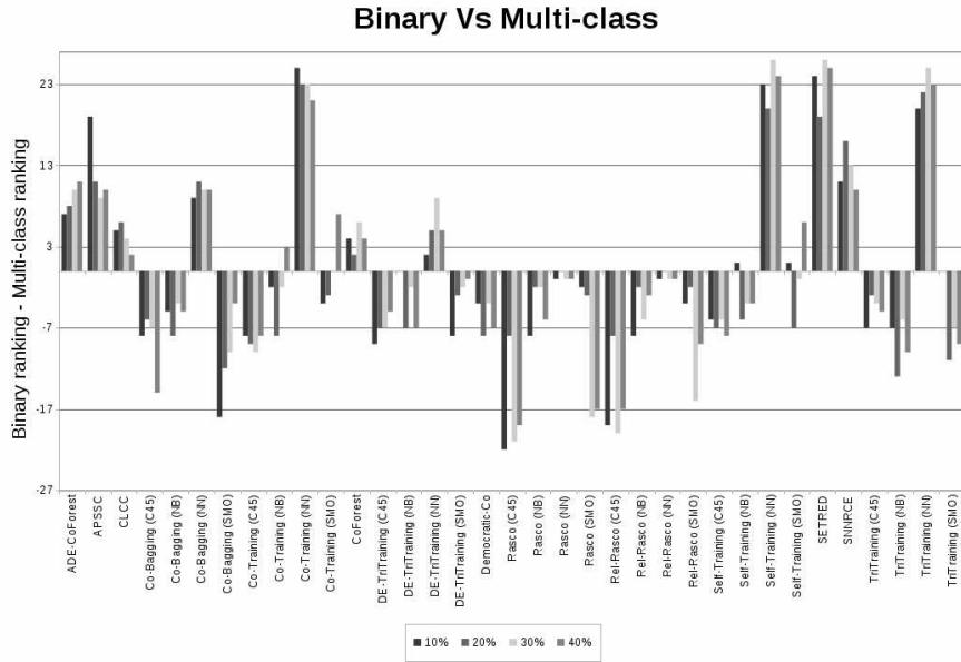
Figure 4: Differences between rankings in Binary and Multi-class domains: Transductive phase
