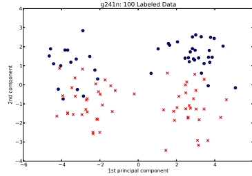
(c) g241n: 100 labeled data
