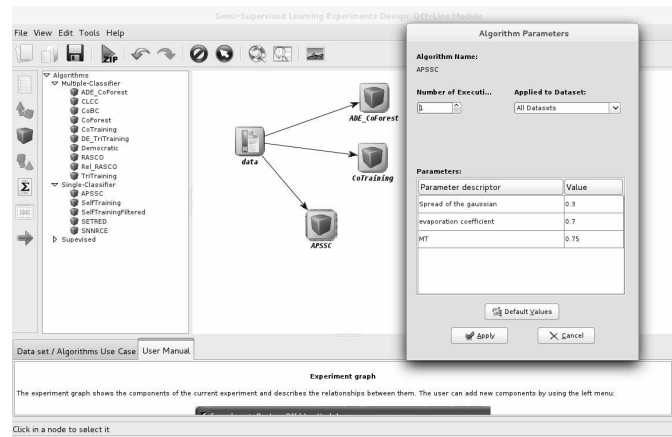
Figure A.13: A snapshot of the Semi-Supervised learning module for KEEL.
