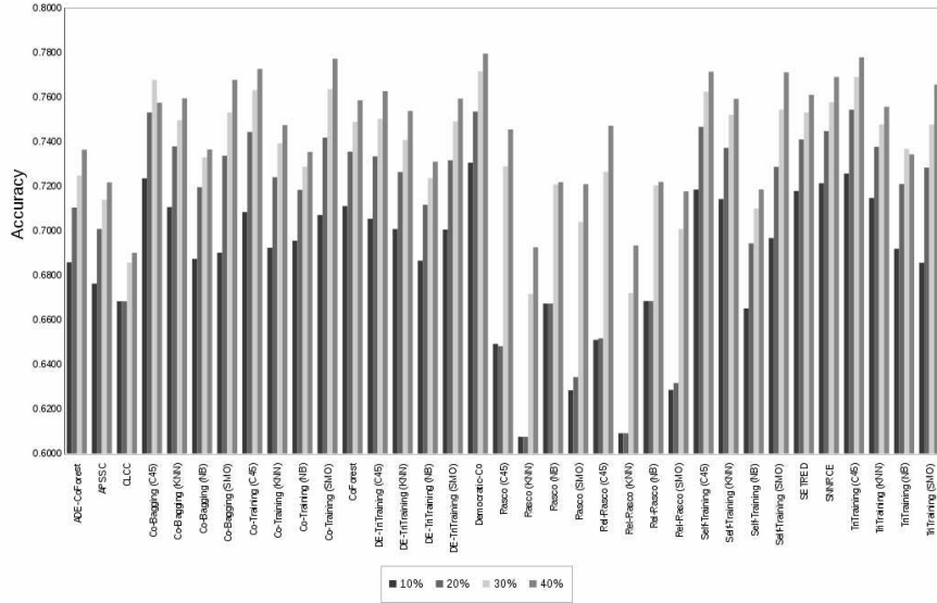
Figure 3: Labeled ratio comparison (bar chart): Transductive phase
