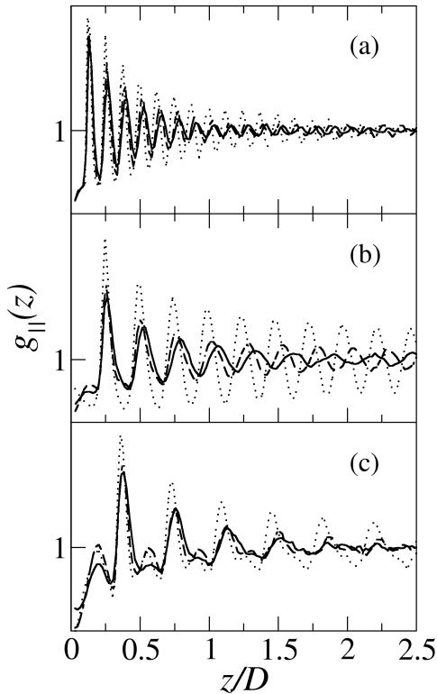
FIG. 5. Longitudinal pair-correlation function, g_{||}(z) , as a function of z , in columnar liquid crystals of oblate hard spherocylinders with length-to-diameter ratios L^* = 0.1 (a), L^* = 0.2 (b), and L^* = 0.3 (c). The solid, dashed, and dotted lines refer to the packing fractions \eta = 0.575 , 0.600 , and 0.630 , respectively.
