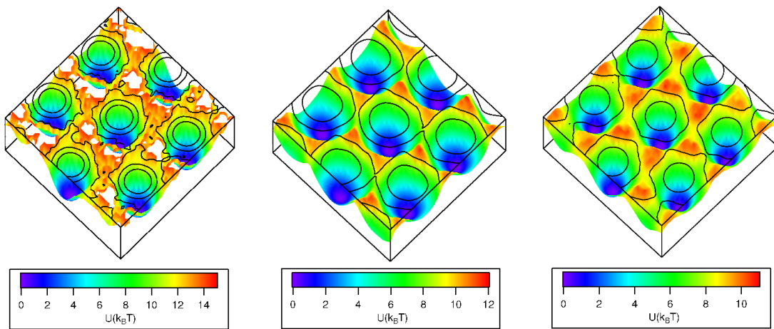
FIG. 6. (Color online). Mean-field effective potential U(x, y) in units of k_B T for the column-to-column diffusion in systems of oblate hard spherocylinders with length-to-diameter ratios L^* = 0.1, 0.2 , and 0.3 , from left to right, respectively. The packing fraction is \eta = 0.575 for the three systems. On top of each graph, isopotential lines in the xy plane with increments of 3k_B T are shown.
