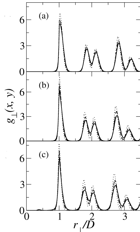
FIG. 4. Transverse pair-correlation function, g_{\perp}(r_{\perp}) , as a function of r_{\perp} = \sqrt{x^2 + y^2} , in columnar liquid crystals of oblate hard spherocylinders with length-to-diameter ratios L^* = 0.1 (a), L^* = 0.2 (b), and L^* = 0.3 (c). The solid, dashed, and dotted lines refer to the packing fractions \eta = 0.575 , 0.600 , and 0.630 , respectively.
