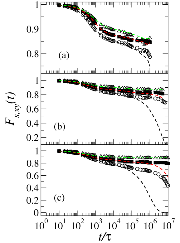
FIG. 14. (Color online). Transverse self intermediate scattering functions, F_{s,xy}(t) , for systems of oblate hard spherocylinders with length-to-diameter ratios L^* = 0.1 (a), L^* = 0.2 (b), and L^* = 0.3 (c), evaluated at packing fractions \eta = 0.575 (circles), \eta = 0.600 (squares), and \eta = 0.630 (triangles). The black, red, and green dashed lines are Gaussian approximations (see text for details).
