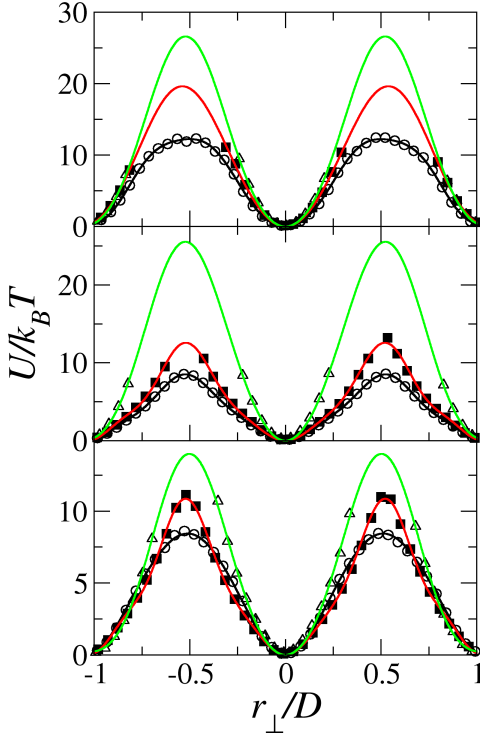
FIG. 7. (Color online). Transverse section of the mean-field effective potential U(x, y) in Fig. 6 for the column-to-column diffusion in columnar liquid crystals of hard oblate spherocylinders with varying length-to-diameter ratios L^* and packing fraction \eta . From top to bottom: L^* = 0.1, 0.2 , and 0.3 . Circles, squares, and triangles, refer to \eta = 0.575, 0.600 , and 0.630 , respectively. The solid lines are fits with m = 5 harmonic modes (see Eq. (8)).
