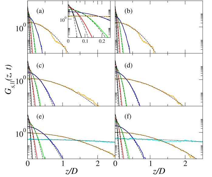
FIG. 9. (Color online). Longitudinal component of the self-part of the van Hove function, G_{s,||}(z, t) , of columnar liquid crystals of OHSCs with length-to-diameter ratios L^* = 0.1 (a, b), L^* = 0.2 (c, d), and L^* = 0.3 (e, f), as a function of z . The packing fractions are \eta = 0.575 (left column) and \eta = 0.600 (right column). The black, red, green, blue, and orange solid curves refer to the time scales t^* = 10^3, 10^4, 10^5, 10^6 , and 10^7 , respectively. The dashed lines are Gaussian fits. At L^* = 0.1 and \eta = 0.575 , we zoom in on shorter distances to better appreciate the deviations from Gaussianity (see inset).
