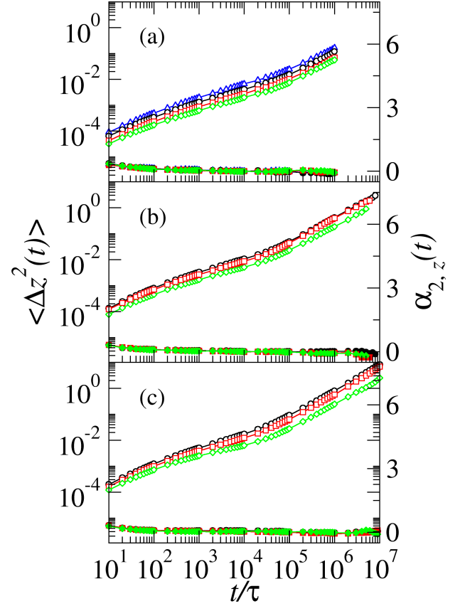
FIG. 11. (Color online). Mean square displacement (open symbols), in units of D^2 , and non-Gaussian parameter (solid symbols) along the nematic director, for systems of oblate hard spherocylinders with length-to-diameter ratios L^* = 0.1 (a), L^* = 0.2 (b), and L^* = 0.3 (c). Circles, squares, and diamonds refer to packing fractions \eta = 0.575, 0.600 , and 0.630 , respectively. For comparison, also the results at L^* = 0.1 and \eta = 0.500 are shown (triangles). Note that the vertical axes of MSDs and NGPs are on the left and right, respectively.
