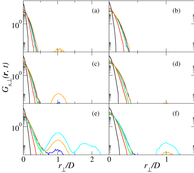
FIG. 10. (Color online). Transverse component of the self-part of the van Hove function, Eq. (5), of columnar liquid crystals of OHSCs with length-to-diameter ratios L^* = 0.1 (a, b), L^* = 0.2 (c, d), and L^* = 0.3 (e, f), as a function of r_{\perp} = \sqrt{x^2 + y^2} . The packing fractions are \eta = 0.575 (left column) and \eta = 0.600 (right column). The black, red, green, blue, orange, and cyan solid curves refer to the time scales t^* = 10^2, 10^3, 10^4, 10^5, 10^6 , and 10^7 , respectively.
