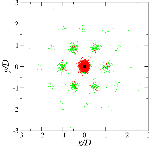
FIG. 8. (Color online). Particle displacements in the planes perpendicular to the nematic director of N = 1280 oblate hard spherocylinders with length-to-diameter ratio L^* = 0.3 at \eta = 0.575 in the columnar phase, collected at t^* = 10 (black points), t^* = 10^6 (red), and t^* = 10^7 (green).
