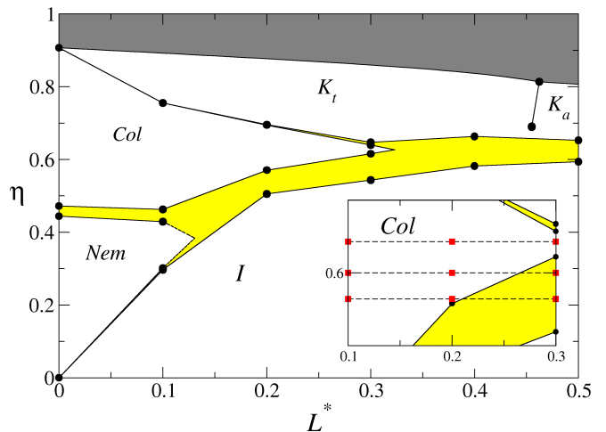
FIG. 2. (Color online). Phase diagram of oblate hard spherocylinders in packing fraction ( \eta ) versus length-to-diameter ratio ( L^* ) as obtained by free-energy calculations from Refs. [79, 80]. I , Nem , Col , K_t , and K_a indicate the isotropic, nematic, columnar, tilted crystal, and aligned crystal phases, respectively. The light-shaded area denotes a two-phase coexistence region, whereas the dark-shaded area contains inaccessible state points which lie above the close packing line. In the inset, we show the nine state points studied in this paper (red squares).
