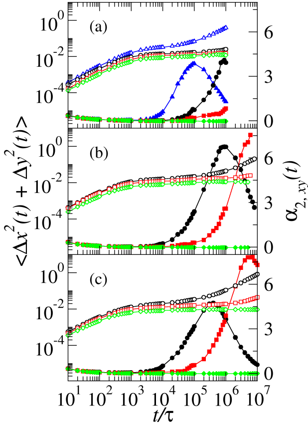
FIG. 12. (Color online). Mean square displacement (open symbols), in units of D^2 , and non-Gaussian parameter (solid symbols) in the plane perpendicular to the nematic director, for systems of oblate hard spherocylinders with length-to-diameter ratios L^* = 0.1 (a), L^* = 0.2 (b), and L^* = 0.3 (c). Circles, squares, and diamonds refer to packing fractions \eta = 0.575 , 0.600 , and 0.630 , respectively. For comparison, also the results at L^* = 0.1 and \eta = 0.500 are shown (triangles). Note that the vertical axes of MSDs and NGPs are on the left and right, respectively.
