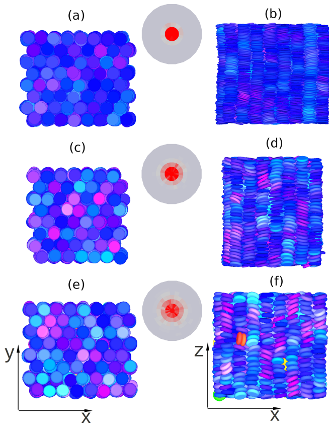
FIG. 3. (Color online). Top (left) and front (right) views of the columnar phase of oblate hard spherocylinders with L^* = 0.1 (a, b), L^* = 0.2 (c, d), and L^* = 0.3 (e, f), at \eta = 0.575 . The gray spheres in the middle show the orientational distribution of the molecular short axes. The particles assume different colors according to their orientation.
