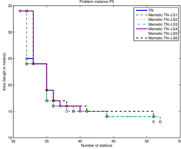
Figure 8: Attainment surface plots of the memetic advanced TSALBP-NSGA-II for instance P5.
