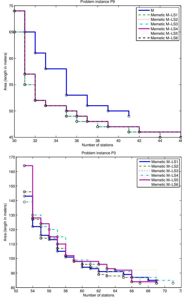
Figure 4: Attainment surface plots of the MACS MAs for instances P3 and P9.
