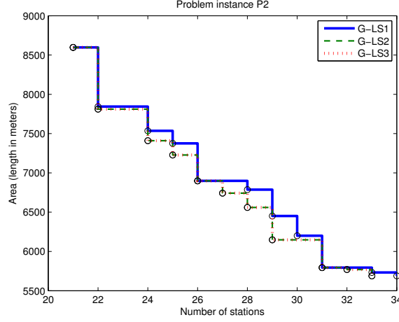
Figure 6: Attainment surface plots of the GRASP methods for instance P2.
