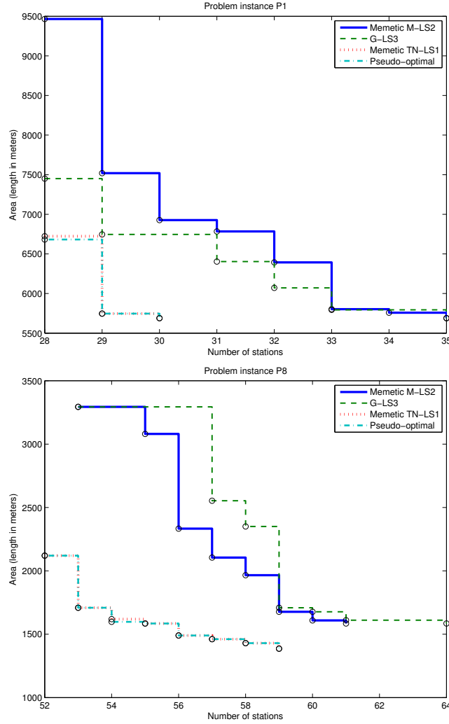
Figure 11: Attainment surface plots of the best variant of each of the three memetic designs for instances P1 and P8.
