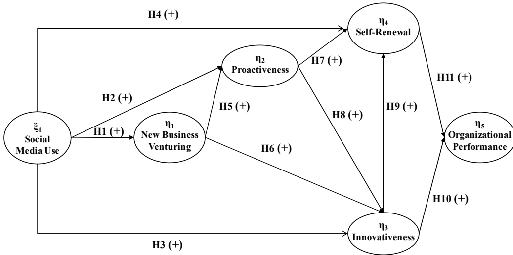
Figure 1: Conceptual model
