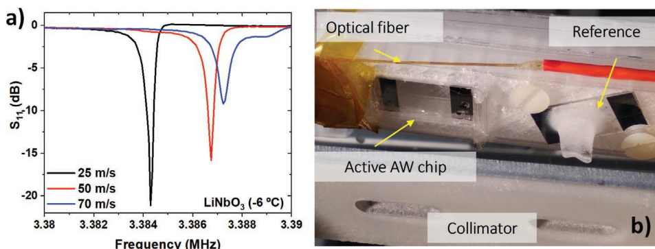
Figure 6. Results of active anti-icing test in an IWT. a) Return loss spectra recorded for a \text{LiNbO}_3 plate at -6^\circ\text{C} in dry conditions under the action of different wind speeds as indicated. b) Photograph of the sample holder emplaced in the IWT behind the collimator after conducting an active anti-icing experiment where a high amount of glacial ice became accreted on the reference sample. The AW-activated chip remained ice-free. Main elements of the experiment appear labeled in the photograph.
