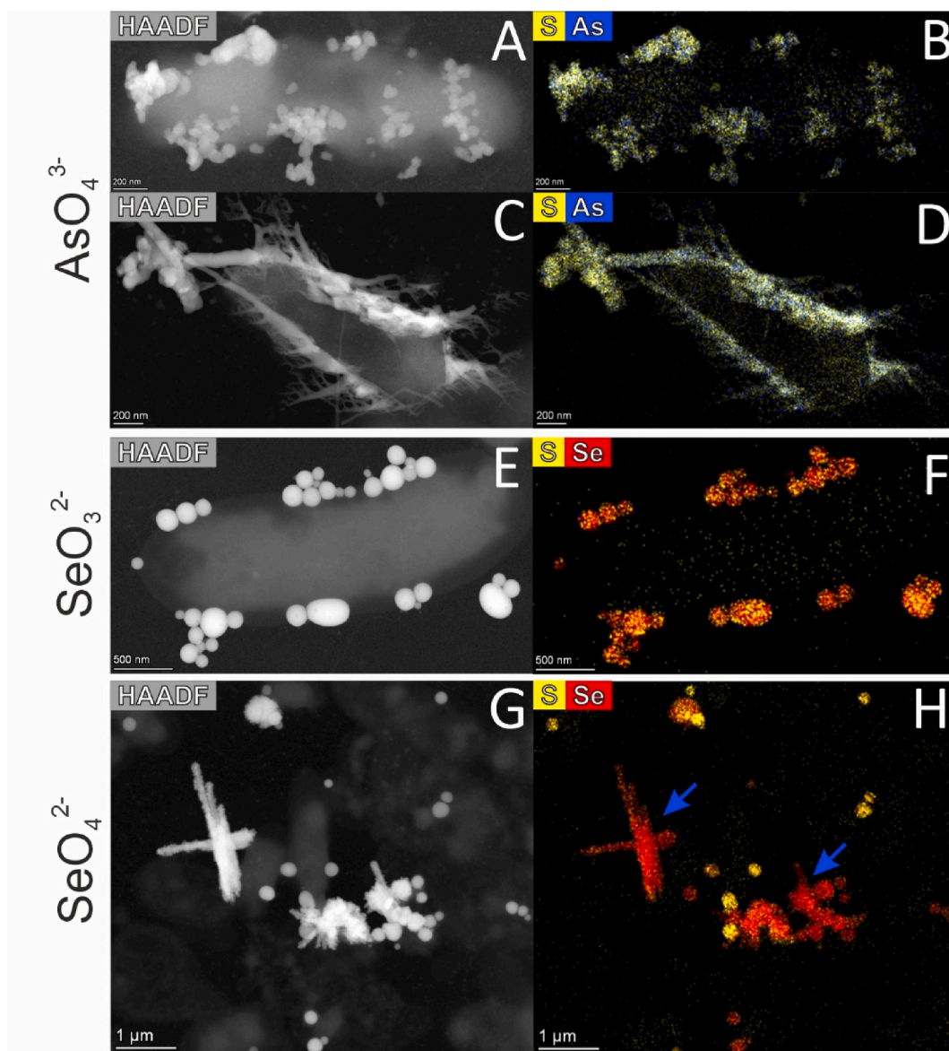
Fig. 3. STEM HAADF images (left panels) with the corresponding EDS elemental maps (right panels) obtained from bacterial cells and biomineralization products in growth media containing \text{AsO}_4^{3-} (A–D), \text{SeO}_3^{2-} (E–F), and \text{SeO}_4^{2-} (G–H). (A–B) Globular particles of As–S phases (with approximately \text{As}_2\text{S}_3 composition); (C–D) Network of As–S nanorods (with approximately \text{AsS} composition); (E–F) Uniformly globular Se nanoparticles with significant associated S content; (G–H) Aggregates of globular and lath-shaped particles of \text{Se}(\text{-S})^0 (blue arrows) with minor and globular \text{Se}(\text{-S})^0 particles with significant S content.
