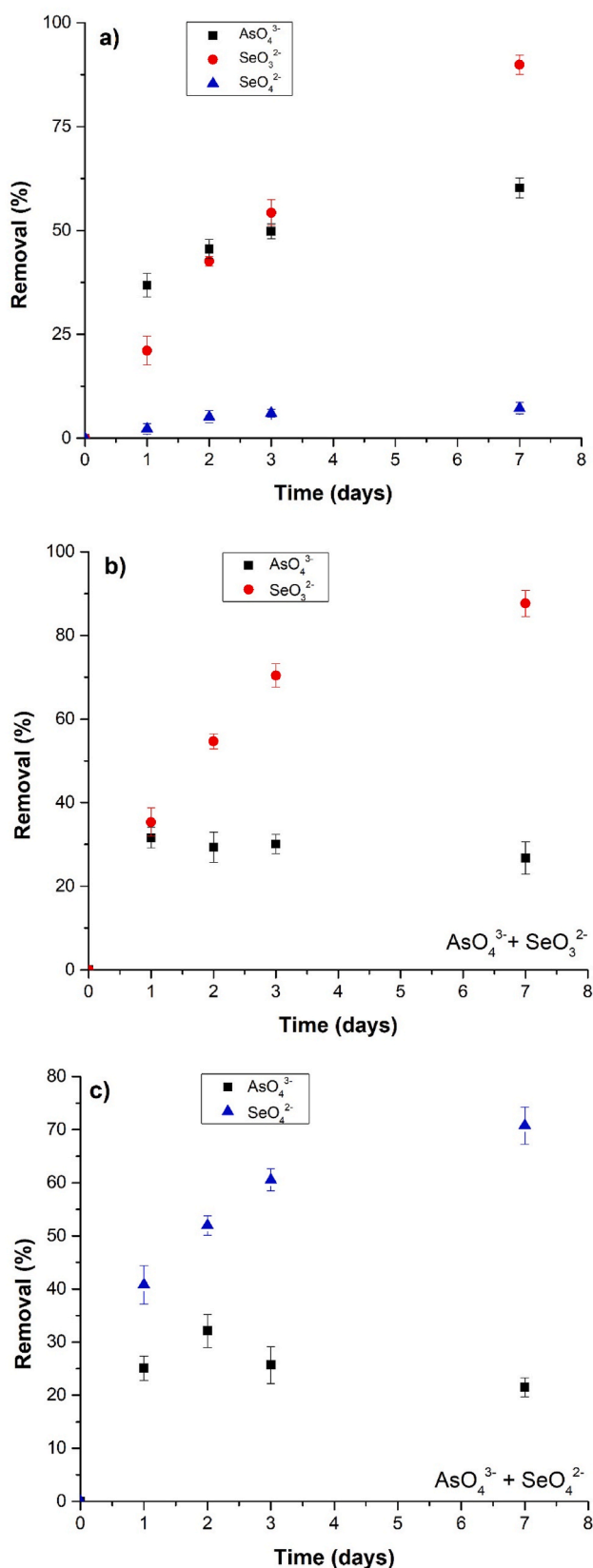
Fig. 2. As and Se removal by Shewanella in BMM. a) \text{AsO}_4^{3-} , \text{SeO}_4^{2-} , and \text{SeO}_3^{2-} removal as a function of incubation time. For easier understanding, the results are presented in the same panel, although the incubations were performed separately; b) \text{AsO}_4^{3-} + \text{SeO}_3^{2-} removal (mixed incubation); c) \text{AsO}_4^{3-} + \text{SeO}_4^{2-} removal (mixed incubation).
