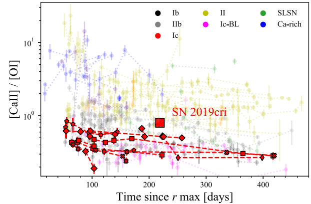
Figure 18. The [Ca II] \lambda\lambda 7291, 7323 /[O I] \lambda\lambda 6300, 6364 plane (Prentice et al., submitted) with SN 2019cri (red square) in context against SNe Ic (red) and other transients (see legend). The ratio of SN 2019cri is marginally larger than SNe Ic at the same epoch. It may be expected however, that if this ratio is a measure of core oxygen mass, that SN 2019cri would be lower than the other transients based upon the light curve and snapshot spectral model, which would indicate a relatively large O mass.
