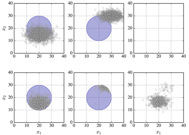
FIGURE 5 Output of the PPN from Figure 4a given for numerical places p_1^{(\mathcal{N})} (leftmost panel) to p_3^{(\mathcal{N})} (rightmost panel) at k = 0 (upper panels) and k = 1 (lower panels)
