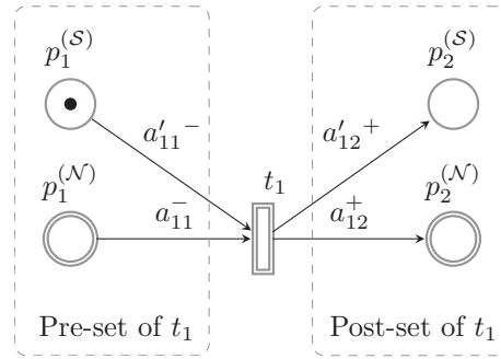
FIGURE 2 Illustration of a sample PPN with two numerical places ( p_1^{(\mathcal{N})}, p_2^{(\mathcal{N})} ), two symbolic places ( p_1^{(\mathcal{S})}, p_2^{(\mathcal{S})} ), and one transition ( t_1 ). Note that numerical nodes are drawn using double lines
