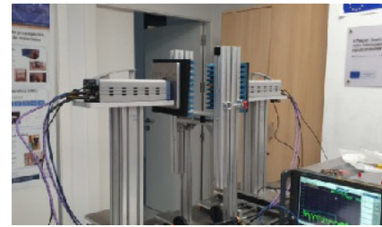
Fig. 1: (a) Measurement scheme used for characterization of materials in free space. (b) Photograph of the setup used for material characterization.
