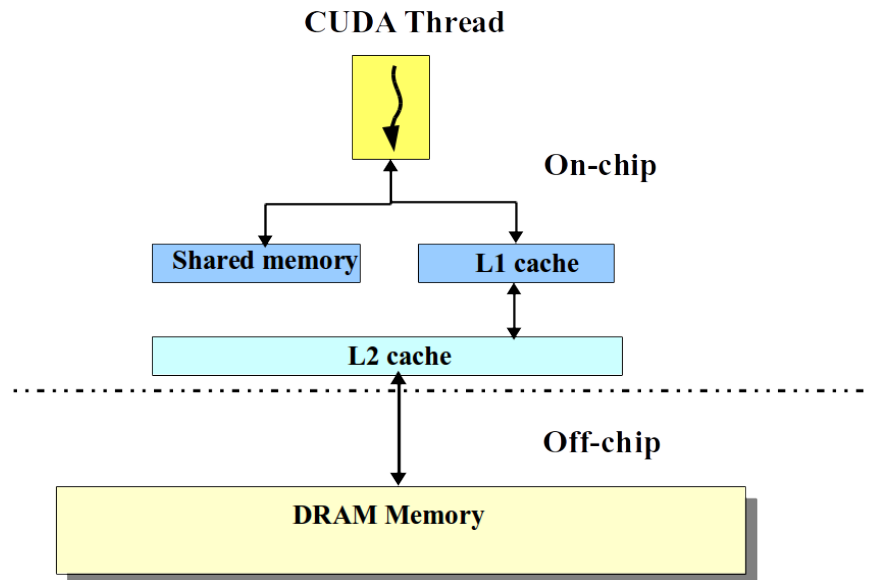
Fig. 13 Memory hierarchy in modern CUDA-enabled GPUs
