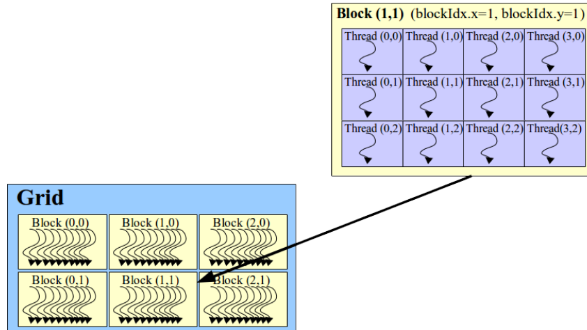
Fig. 7 Grid of thread blocks
