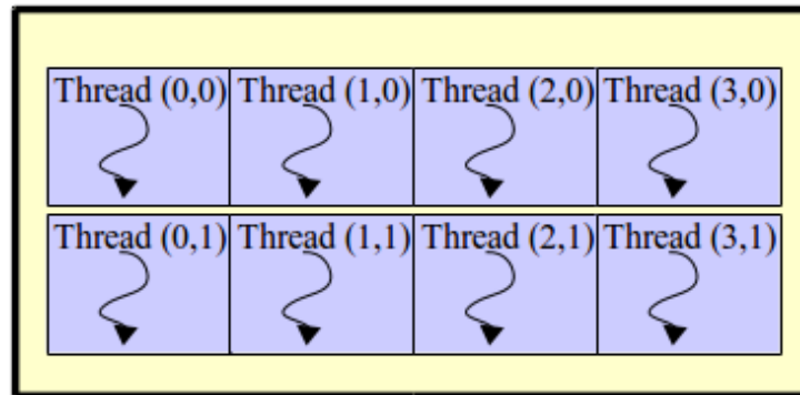
Fig. 6 Structure of 1D and 2D Blocks of CUDA threads
