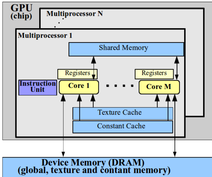
Fig. 4 CUDA hardware model
