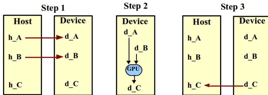
Fig. 16 Description of Data Transfers and Kernel Launch in a CUDA program
