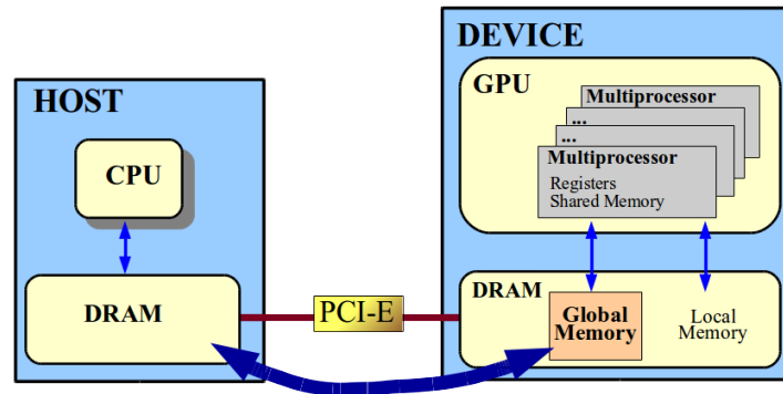
Fig. 15 Host-device memory transfer
