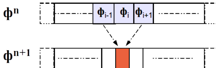
Fig. 17 2-point stencil of the Lax-Friedrichs method
