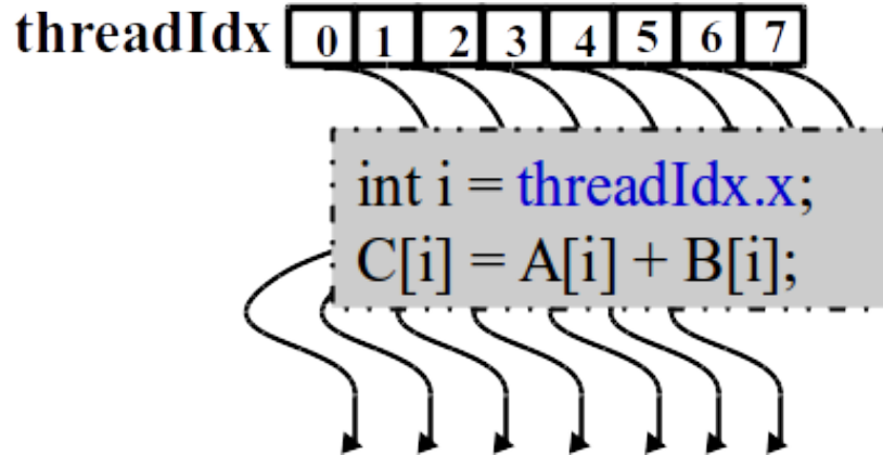
Fig. 5 Thread array for a naive CUDA kernel
