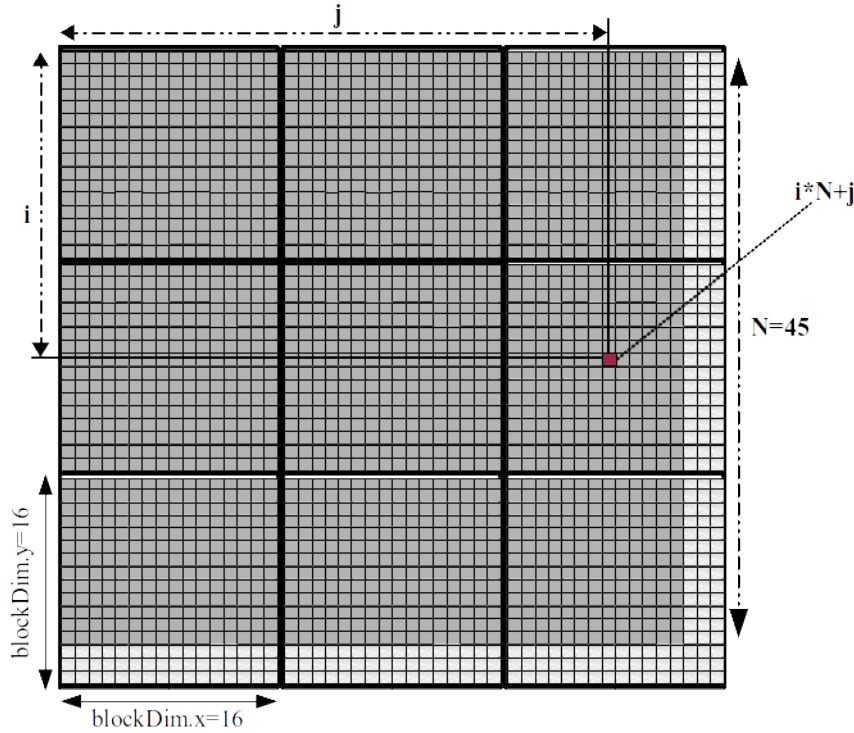
Fig. 9 Mapping of a 2D grid of 16 \times 16 blocks to a 45 \times 45 matrix
