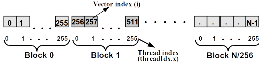
Fig. 8 Mapping of a vector to one-dimensional blocks
